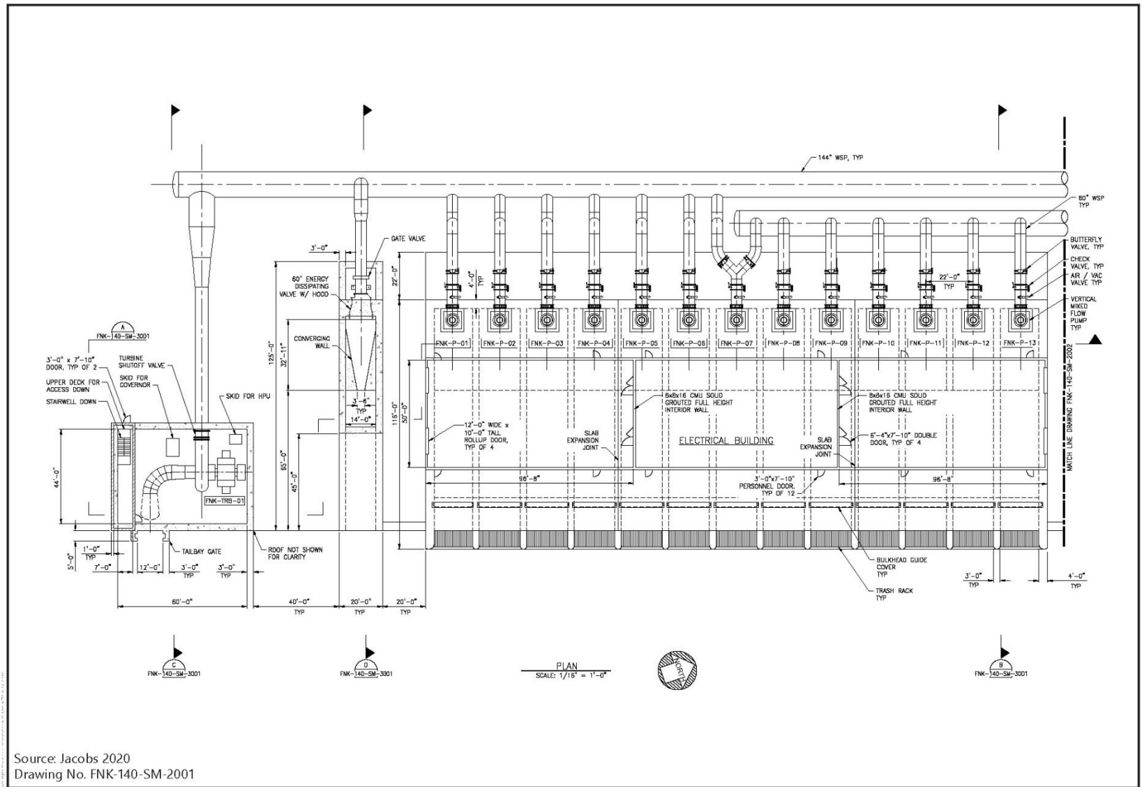
Figure 2-16A Funks Pumping Generating Plant Facilities
