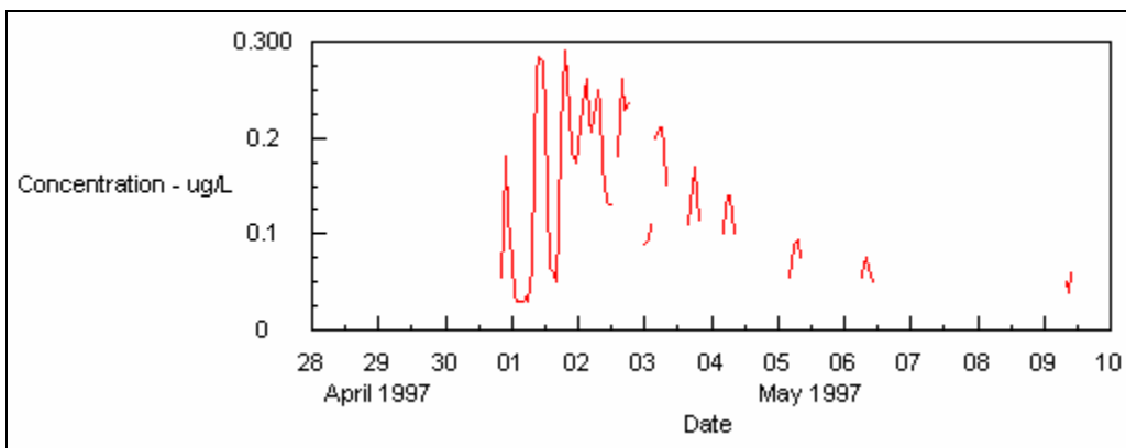
Figure 4-17: Tracer Concentration at Grantline Canal near Tracy Blvd. Bridge.
