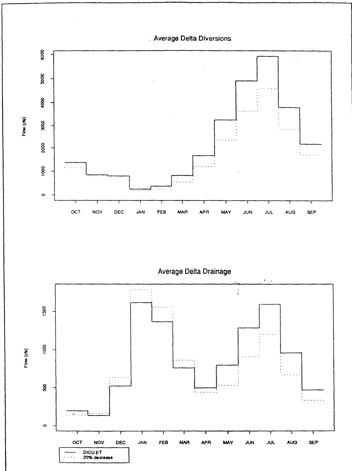
Figure 8-14. Sensitivity of Evapotranspiration Decrease
