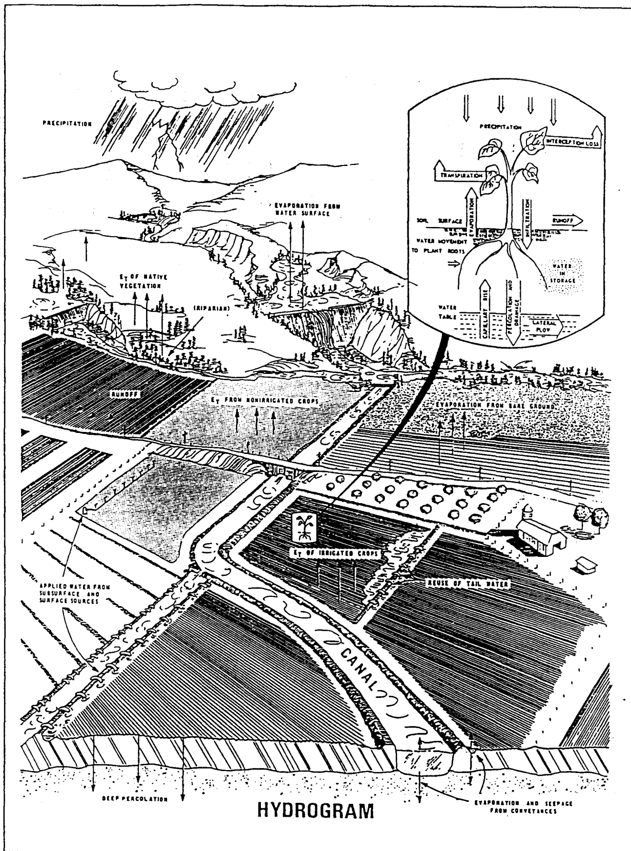
Figure 2-1. Hydrologic Cycle
