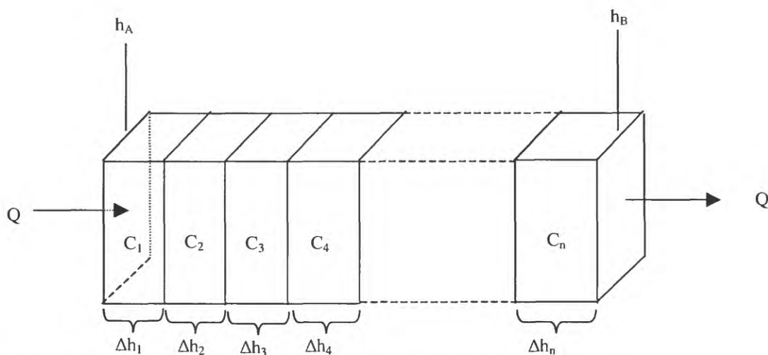
Figure 4.-- Calculation of conductance through several prisms in series.
