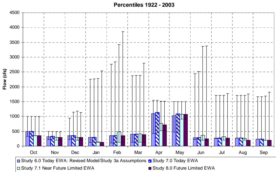
Figure 10-122 Goodwin Releases 50 th Percentile Monthly Releases with the 5 th and 95 th as the Bars
