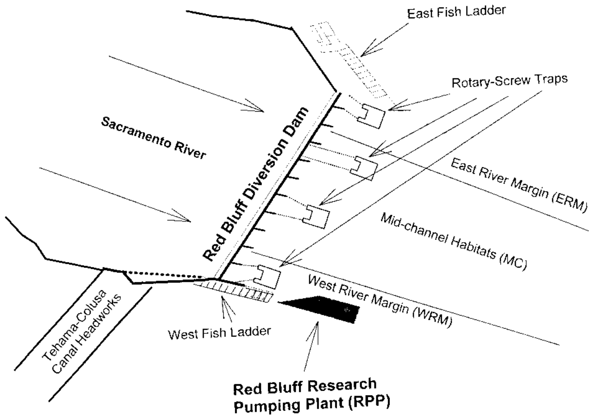
Figure 2.--Rotary-screw trap sampling transect at Red Bluff Diversion Dam (RK391) on the Sacramento River, CA.
