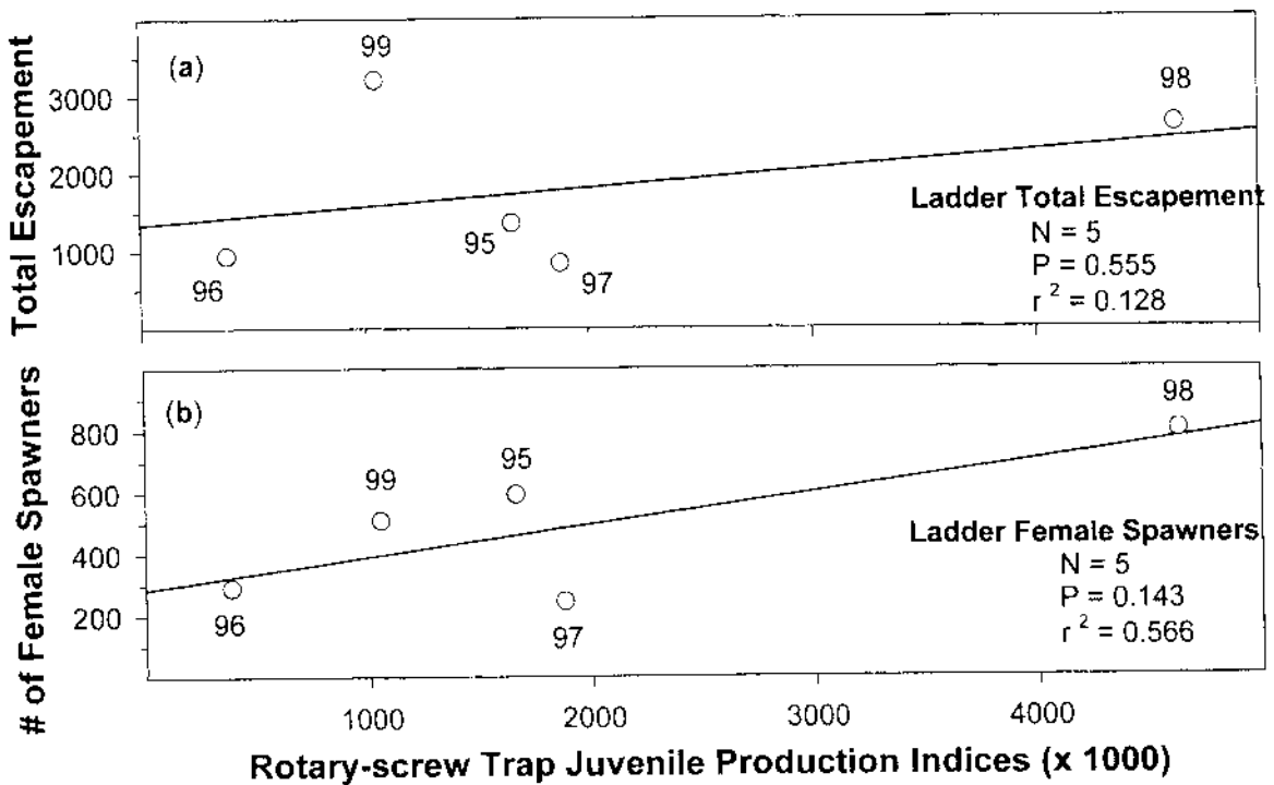
Figure 14. Linear relationship between rotary-screw trap juvenile production indices (JPI's) and RBDD ladder count derived (a) total escapement estimates and (b) estimates of the number of female spawners (FS).
