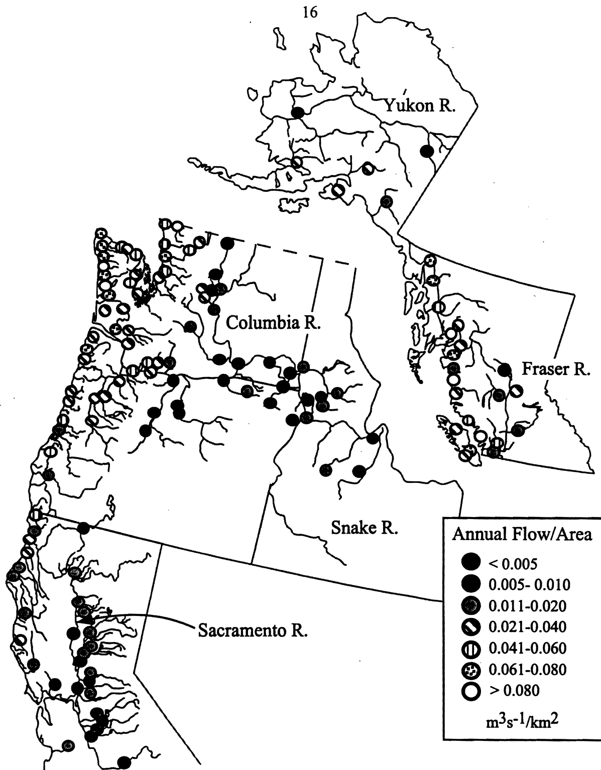
Figure 5. Average annual flow per area ( m^3seconds(s)^{-1}km^{-2} ) for selected river basins in Alaska, British Columbia, Washington, Oregon, California, and Idaho. Values were calculated as the average annual flow for each gauging station divided by the reported gauged area. Based on USGS streamflow data (Hydrosphere Data Products, Inc. 1993) and Inland Water Directorate streamflow data (Environment Canada 1991) (modified from Weitkamp et al. 1995).
