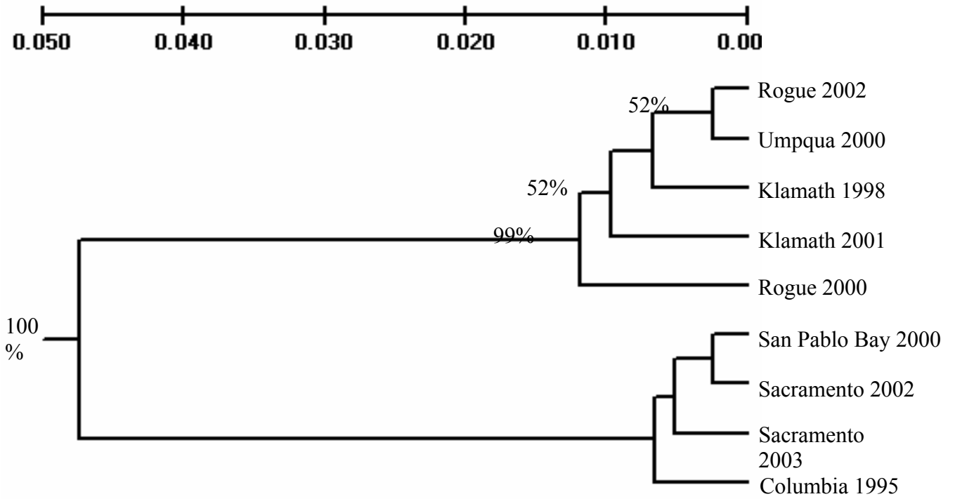
Figure 1. UPGMA dendrogram from green sturgeon samples was built using Nei's unbiased minimum genetic distance. The distance between each collection was calculated by bootstrapping 1000 times and node support represented as a percentage of the trees which displayed similar topology (J. Israel and B. May pers. comm.).
