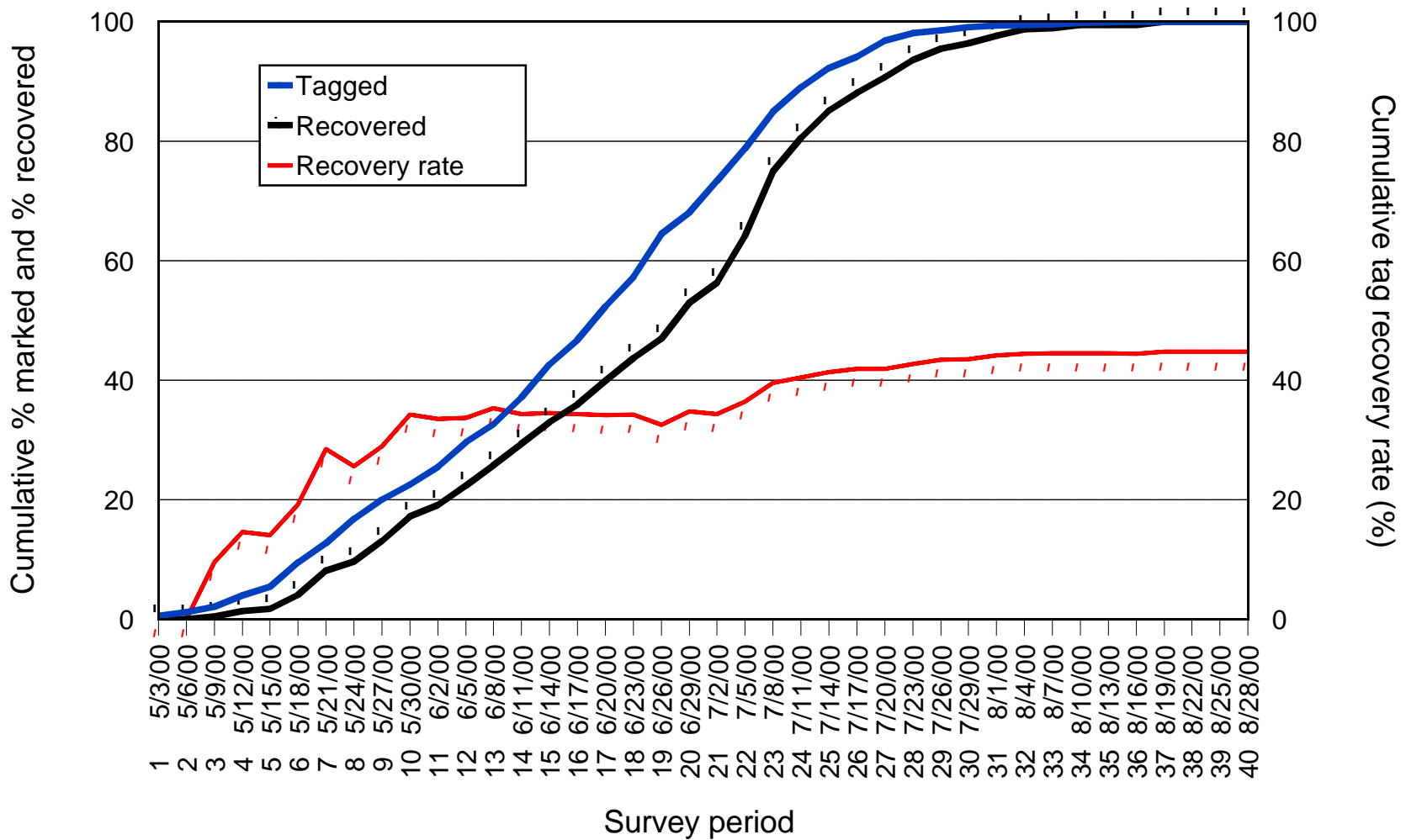
Figure 4. Comparison of temporal distribution of tagging versus recovering of tagged fresh carcasses and tag recovery rate ( n tagged/ n recovered) during the upper Sacramento River winter-run chinook salmon escapement survey, May - August 2000.
