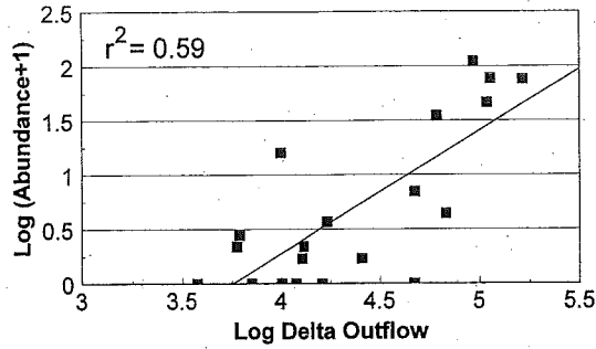
FIGURE 7.—Relationship ( \log_{10} ) between age-0 fall midwater trawl abundance and average delta outflow during February–May.
