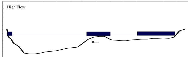
Figure 5.24. Representation of the existing channel with the riparian berm and the rehabilitated channel with salmonid fry rearing habitat (represented by the boxes) at low, intermediate, and high flows.
