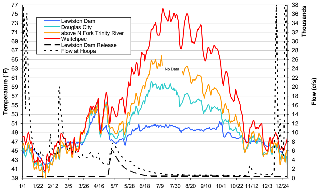
Figure 11-24. Trinity River water temperatures and flow at monitoring sites in a dry year type, actual measured water temperatures (2002).
