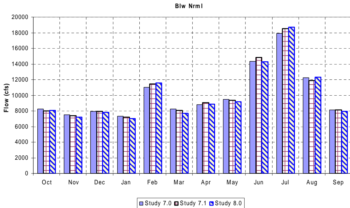
Figure 10-7 Keswick+Nimbus Releases – Below Normal
