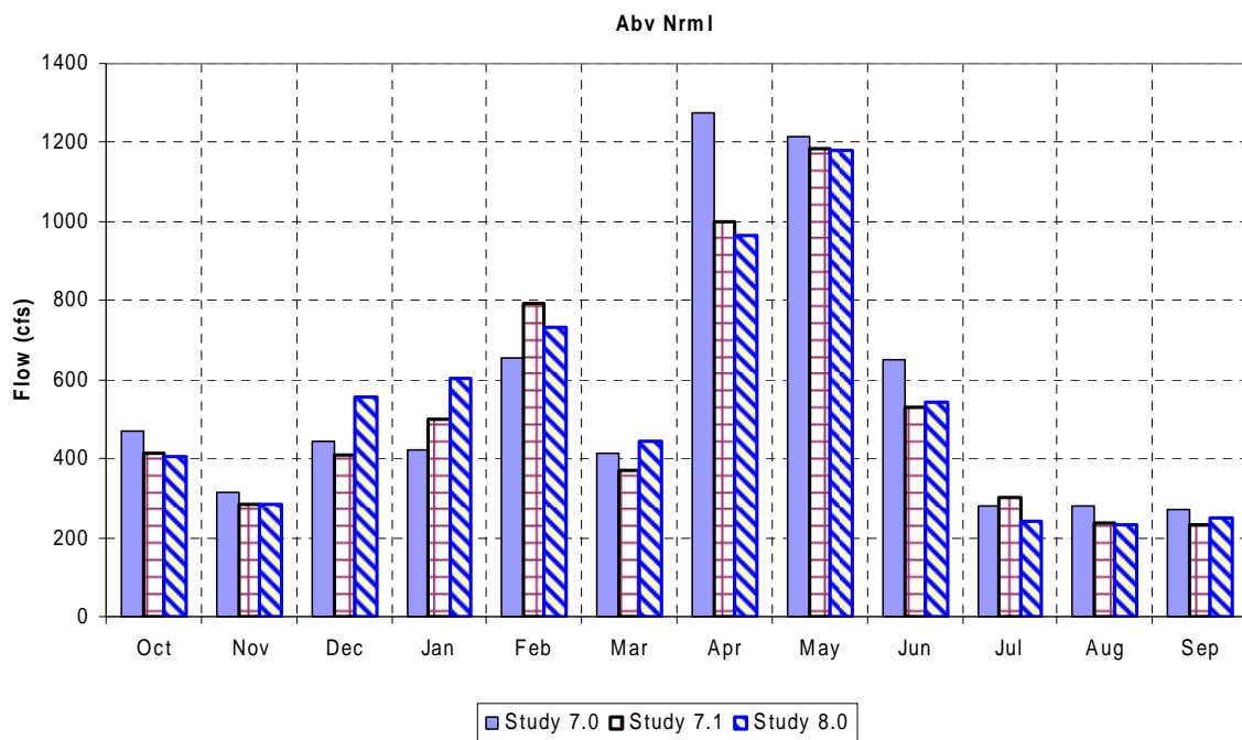
Figure 10-125 Average Above Normal Year (40-30-30 Classification) Monthly Goodwin Releases
