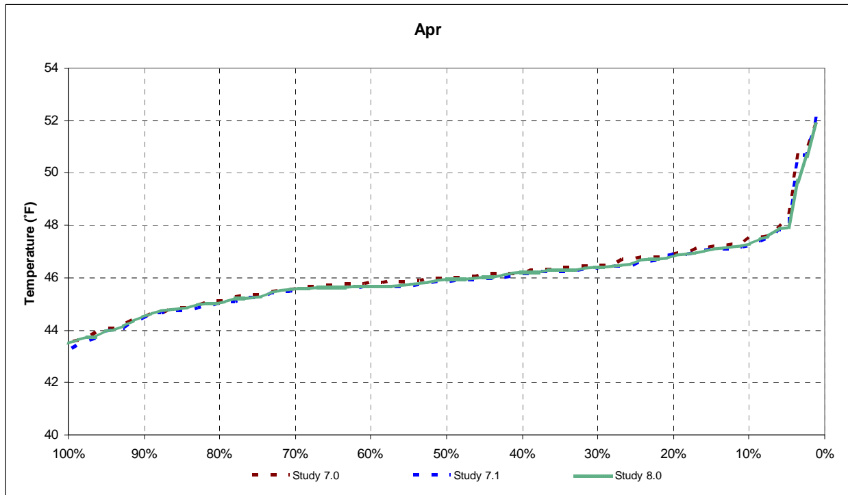
Figure 10-58 Shasta Tailbay End-of-April Exceedence
