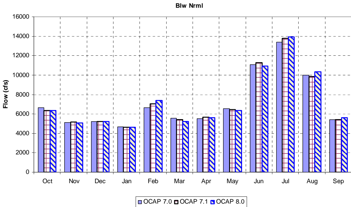
Figure 10-51 Average Below Normal Year (40-30-30 Classification) Monthly Releases from Keswick
