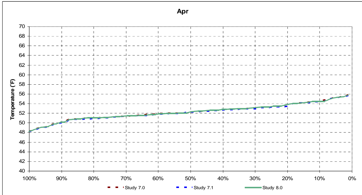
Figure 10-82 Bend Bridge End-of-April Exceedence
