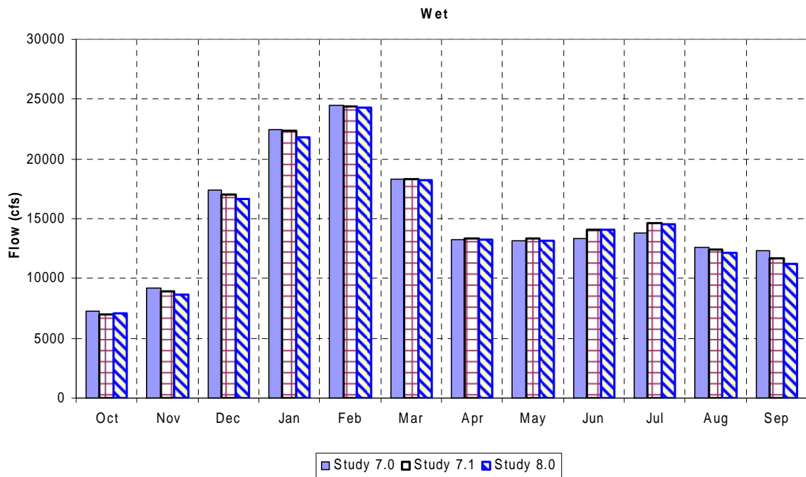
Figure 10-5 Keswick+Nimbus Releases - Wet
