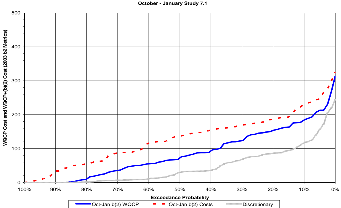
Figure 9-11 Oct – Jan WQCP and Total (b)(2) Costs Probability of Exceedance Study 7.1
