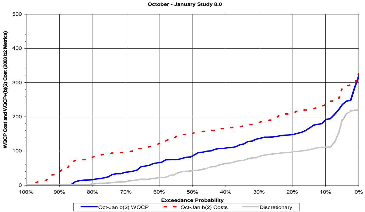
Figure 9-12. Oct – Jan WQCP and Total (b)(2) Costs Probability of Exceedance Study 8.0
