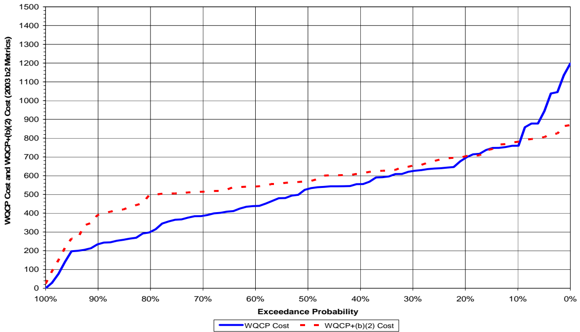
Figure 9-14. Annual WQCP and Total (b)(2) Costs Probability of Exceedence for Study 7.1
