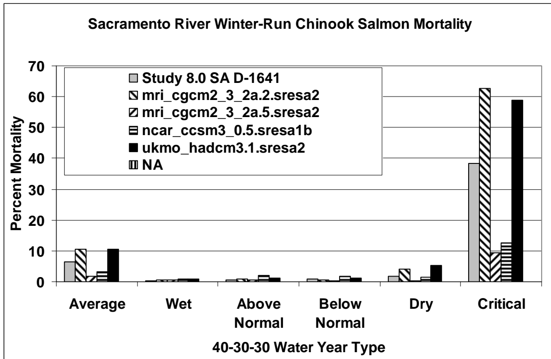
Figure 11-62. Sacramento River winter-run Chinook egg mortality with climate change scenarios compared to study 8.0 from Reclamation egg mortality model.
