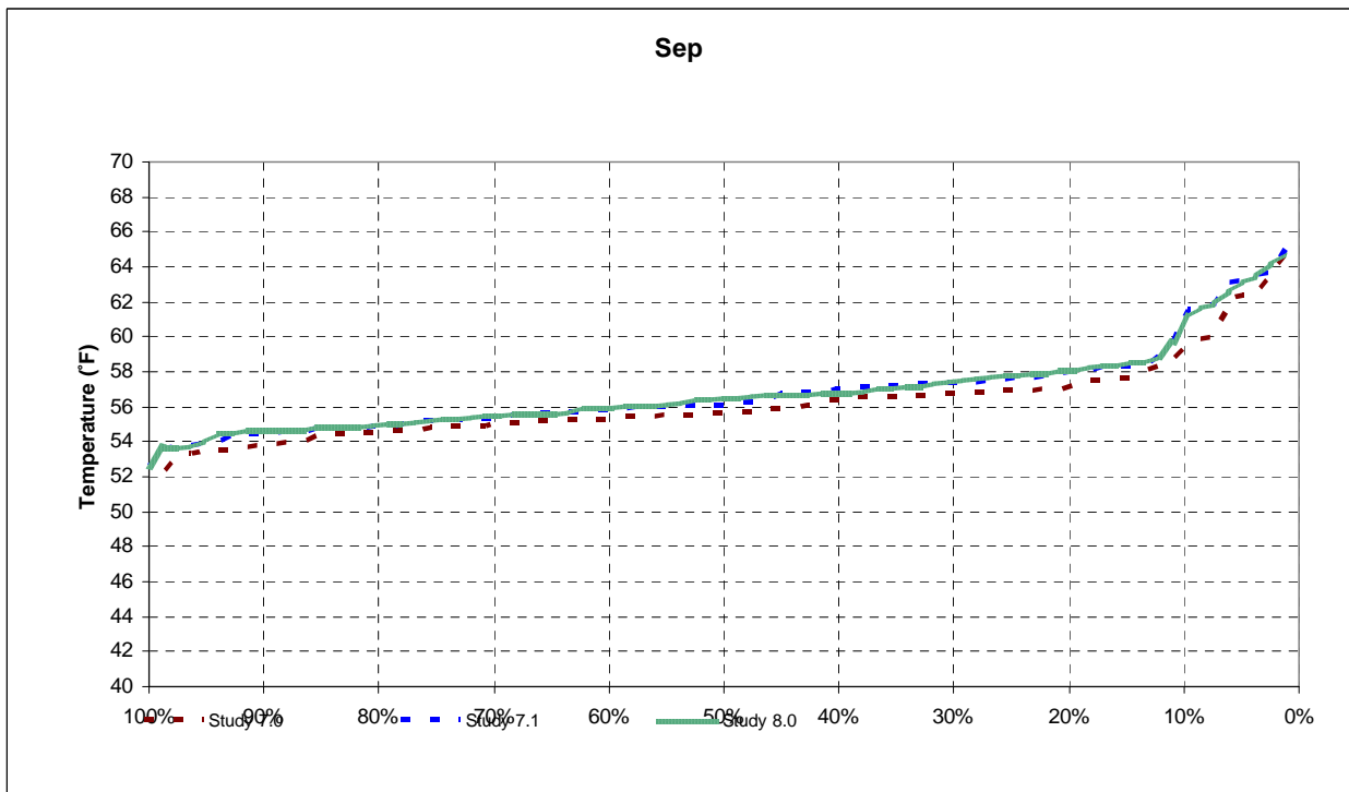
Figure 10-79 Balls Ferry End-of-September Exceedence
