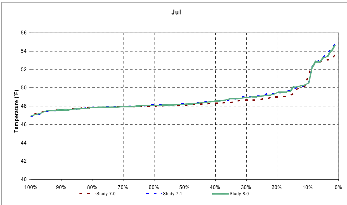
Figure 10-61 Shasta Tailbay End-of-July Exceedence
