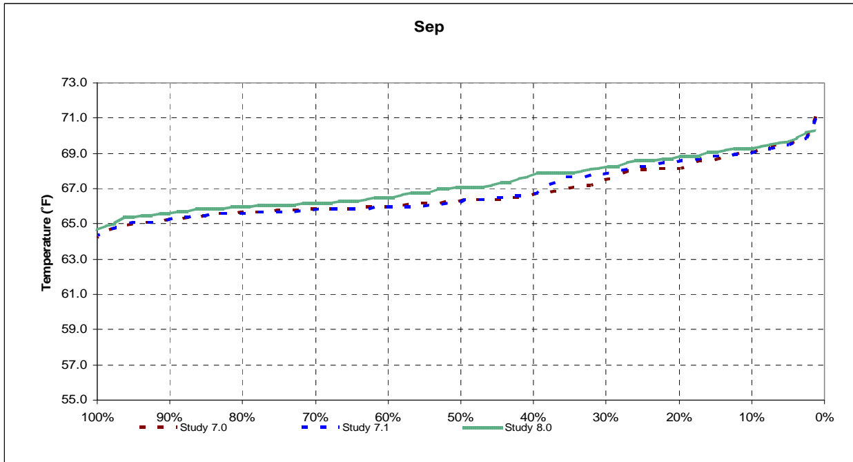
Figure 10-117 Watt Avenue End-of-September Exceedence
