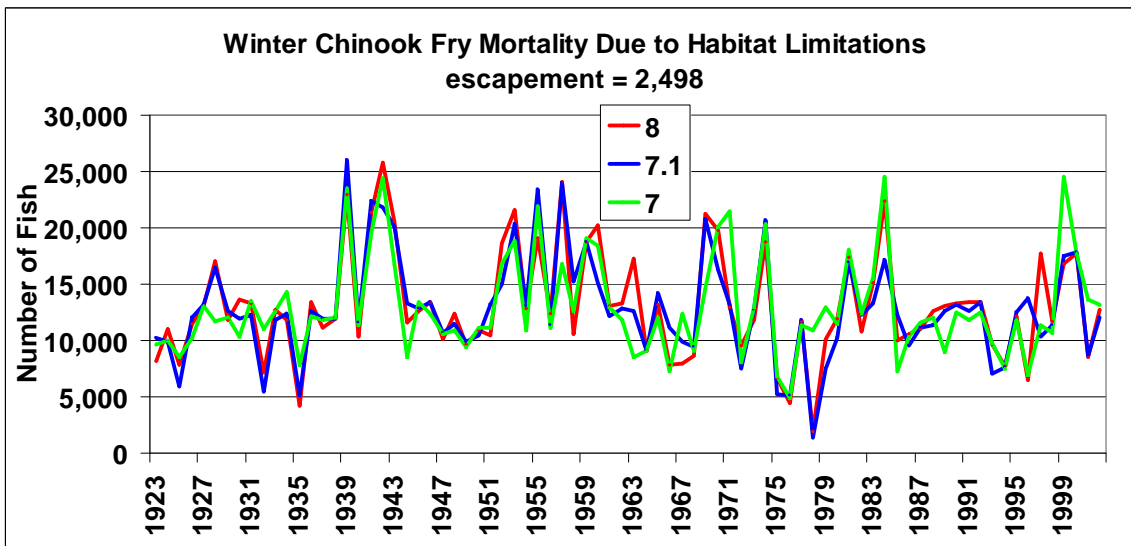
Figure 11-43. Winter-run Chinook salmon fry mortality due to habitat limitations by water operational scenario, 1923-2002 from SALMOD model. Study 7.0 represents current operations, 7.1 represents near future operations, and 8.0 represents future operations.
