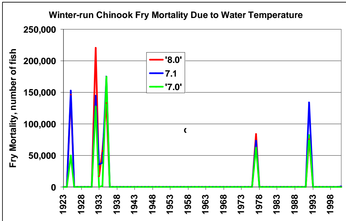
Figure 11-42. Winter-run Chinook fry mortality due to water temperature by operational scenario. Study 7.0 represents current operations, 7.1 represents near future operations, and 8.0 represents future operations.
