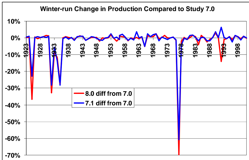
Figure 11-38. Percentage change in juvenile winter-run Chinook production past Red Bluff of future operational scenarios compared with the current scenario from the SALMOD model. Study 7.0 represents current operations, 7.1 represents near future operations, and 8.0 represents future operations
