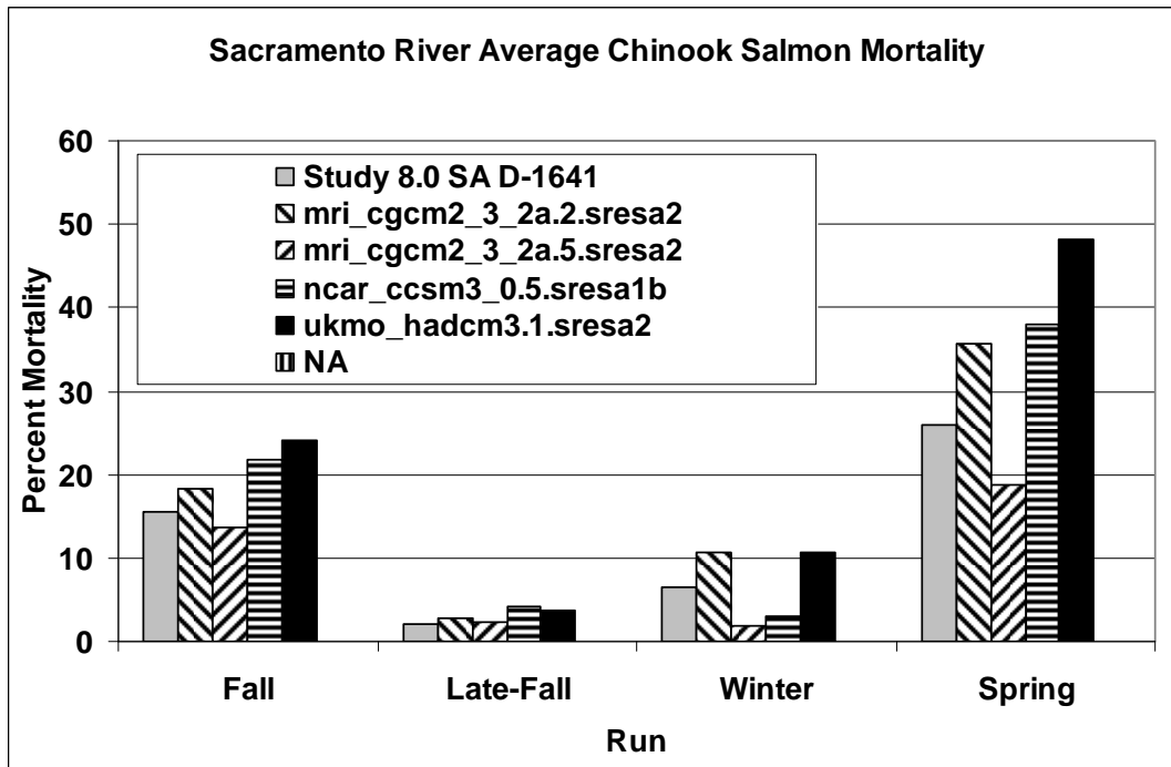
Figure 11-66. Sacramento River average Chinook salmon mortality by run and climate change scenario from Reclamation salmon egg mortality model.
