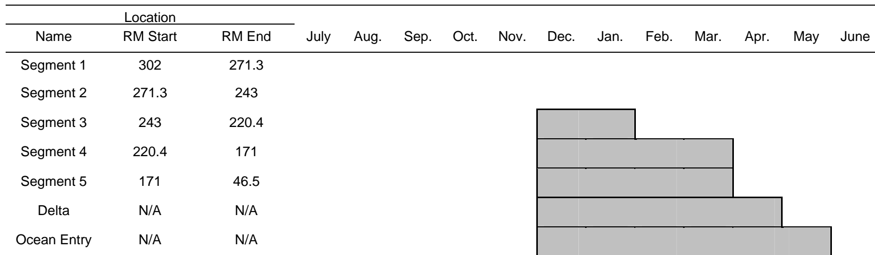
Figure 11-58. Monthly spatial distribution of winter-run Chinook salmon pre-smolts and smolts in the IOS Winter-Run Life Cycle Model during OCAP Biological Assessment model runs from IOS model.
