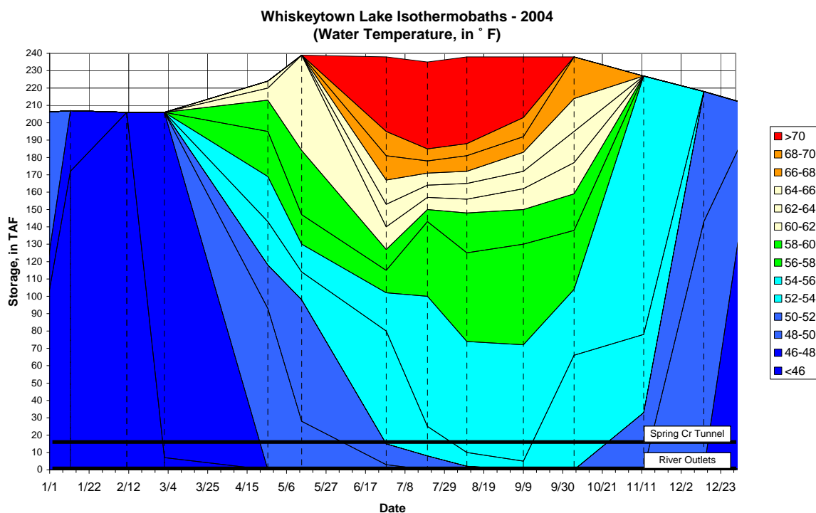
Figure 11-30. Whiskeytown Lake isothermobaths in 2004.
