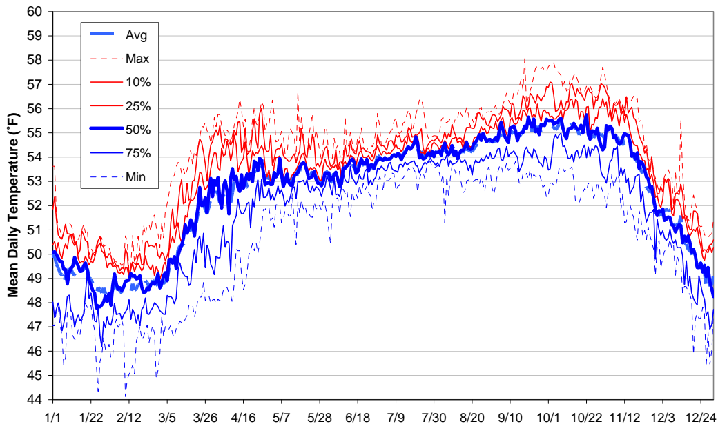
Figure 11-5. Sacramento River at Balls Ferry seasonal temperature exceedence, 1997-2007 (actual temperatures, not modeled).
