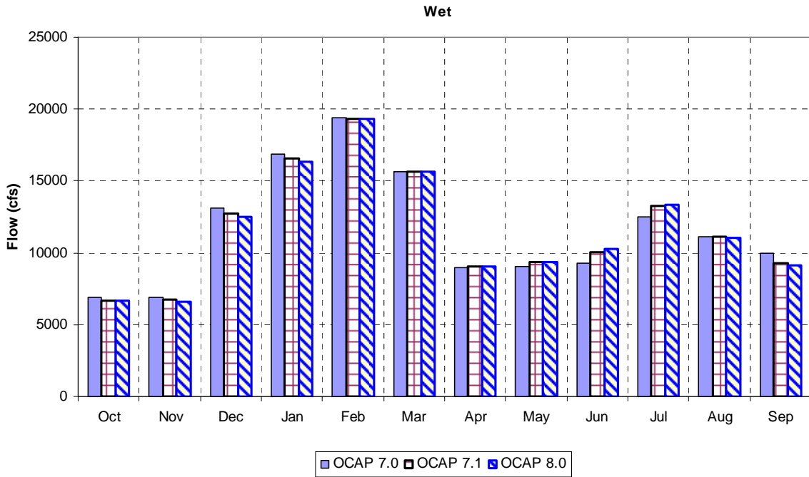
Figure 10-49 Average Wet Year (40-30-30 Classification) Monthly Releases from Keswick
