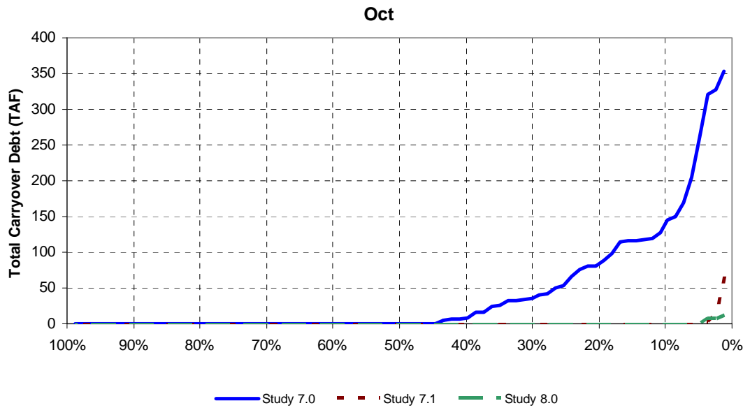
Figure 9-17. Combined Carryover Debt at CVP and SWP San Luis, Simulated in CalSim- II, at the End (Oct) and Start (Nov) of the Carryover Debt Assessment Year
