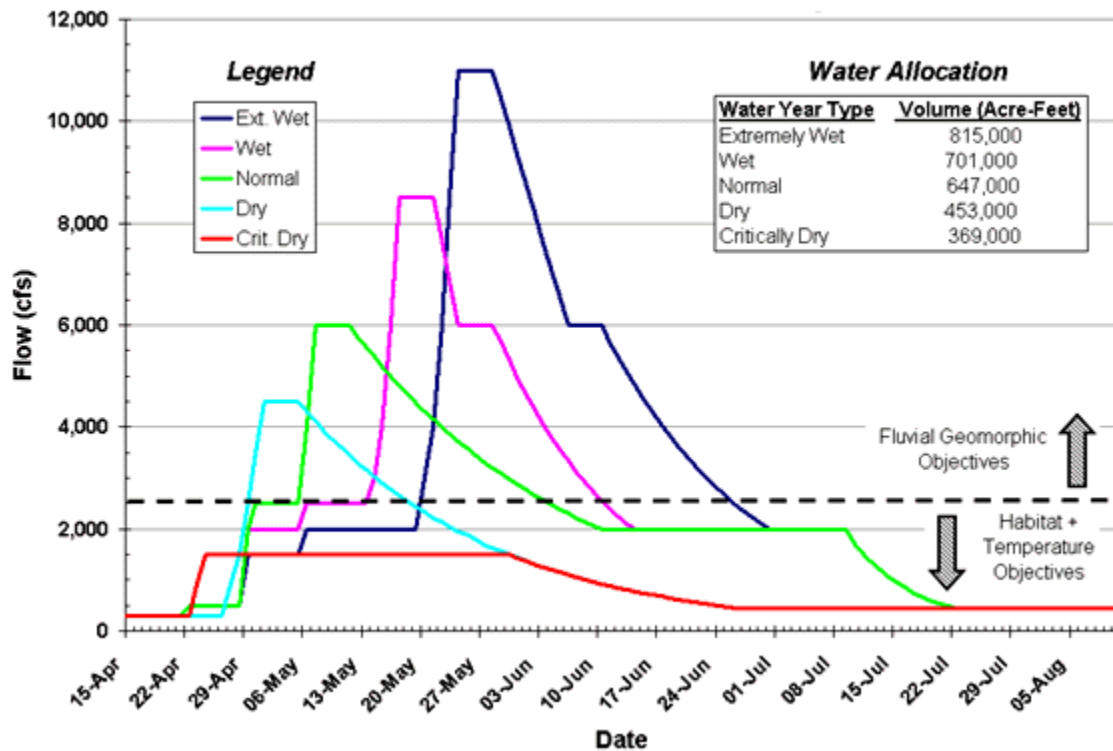
Figure 11-27. Trinity River Restoration Program recommended flow releases from Lewiston Dam to the Trinity River including functional performance ranges.
