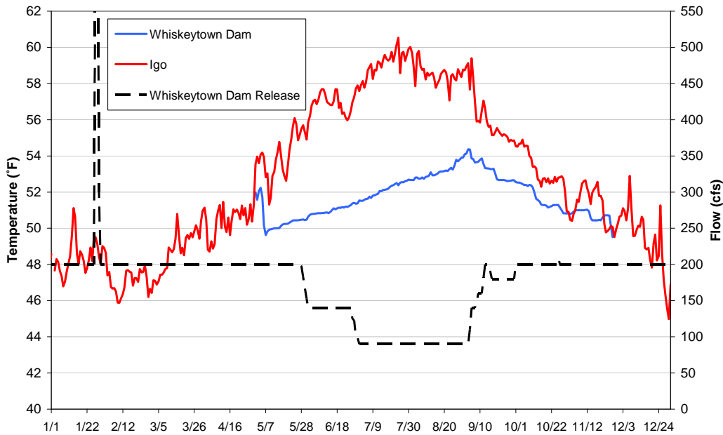
Figure 11-12. Clear Creek mean daily temperature at Whiskeytown Dam and Igo in an above normal water year, actual measured water temperatures (2003).
