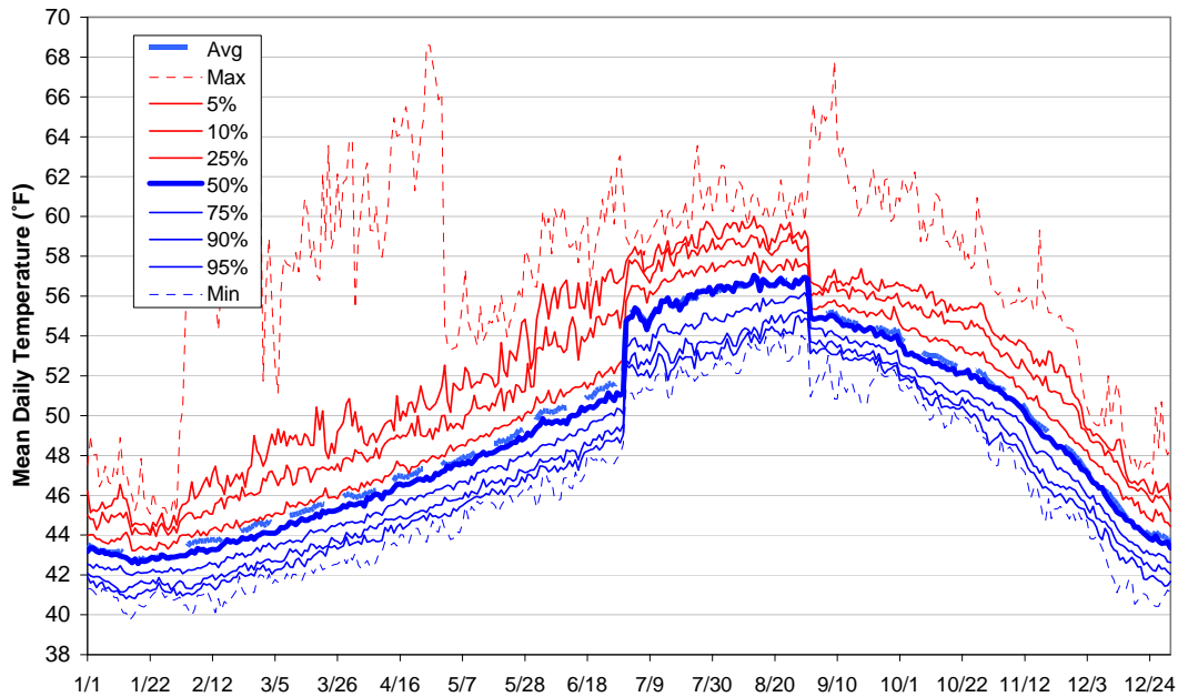
Figure 11-29. Water temperature exceedence in Clear Creek at Igo in OCAP modeling study 7.0 throughout the Calsim modeling hydrological record.
