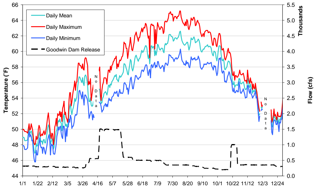
Figure 11-21. Stanislaus River at Orange Blossom Bridge daily temperature fluctuation and flow in a dry water year, actual measured water temperatures (2001).
