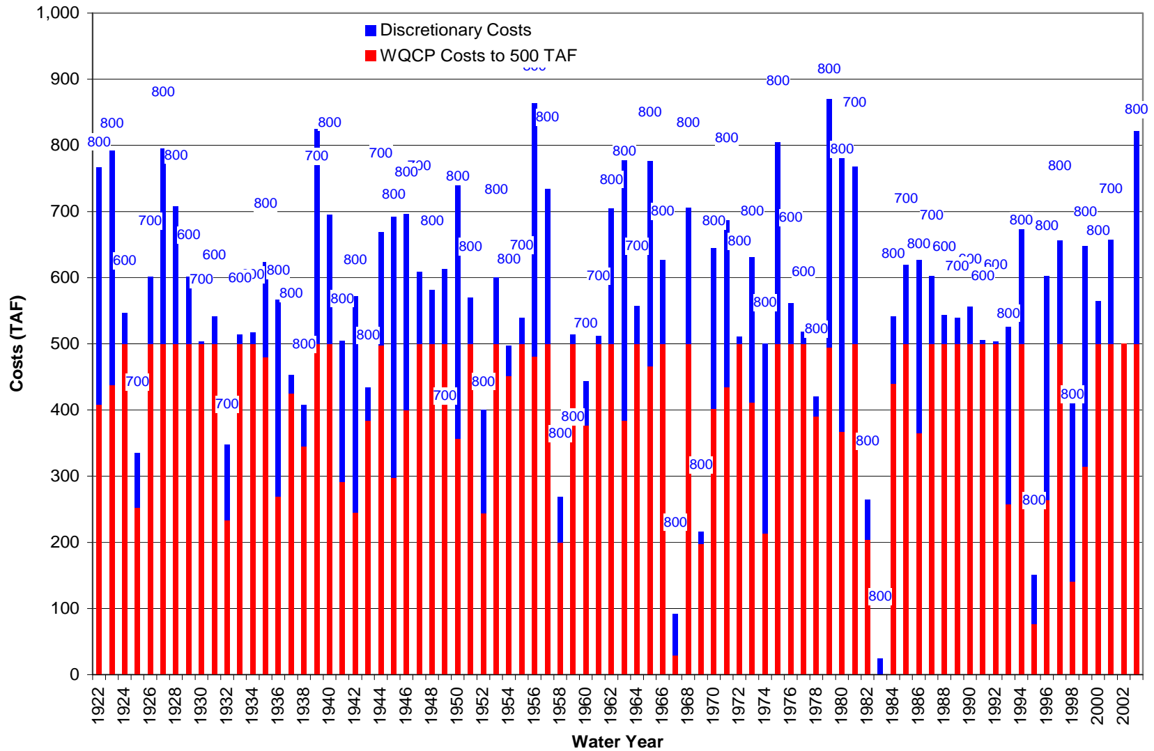
Figure 9-8 Study 7.1 Total Annual WQCP and Total (b)(2) Costs
