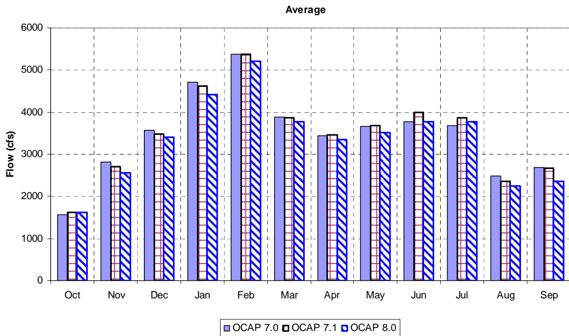
Figure 10-94 Average Monthly Nimbus Release
