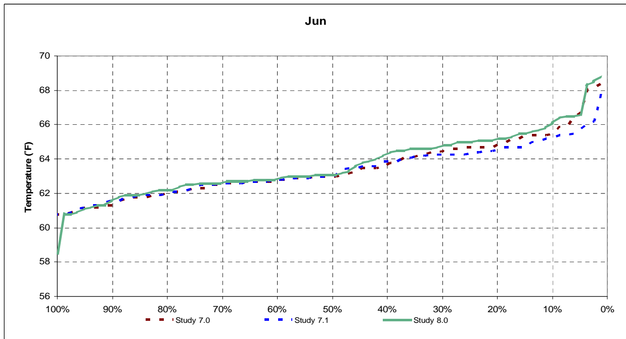
Figure 10-102 Folsom Tailbay End-of-June Exceedence
