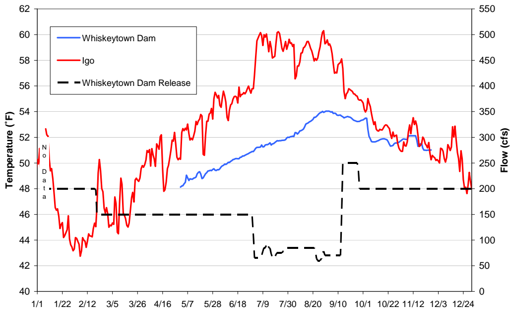
Figure 11-11. Clear Creek mean daily temperature at Whiskeytown Dam and Igo in a dry year, actual measured water temperatures (2002).
