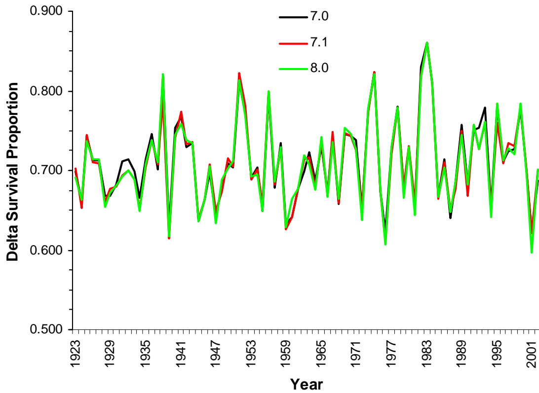
Figure 11-57. Annual winter-run Chinook salmon Delta survival under three OCAP water operation scenarios, 1923-2002 from IOS model. Study 7.0 represents current operations, 7.1 represents near future operations, and 8.0 represents future operations.
