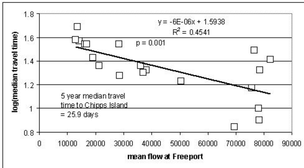
Figure 6-23 Relationship between mean flow (cfs) in the Sacramento River and the log10 time to recapture in the FWS Chipps Island Trawl for Coleman Hatchery late-fall-run Chinook salmon smolts. The explanatory variable is mean flow at Freeport for 30 days beginning with the day of release from Coleman Hatchery. The response variable is an average of median days to recapture for November through January releases during winter 1993–94 through 1998–99.
