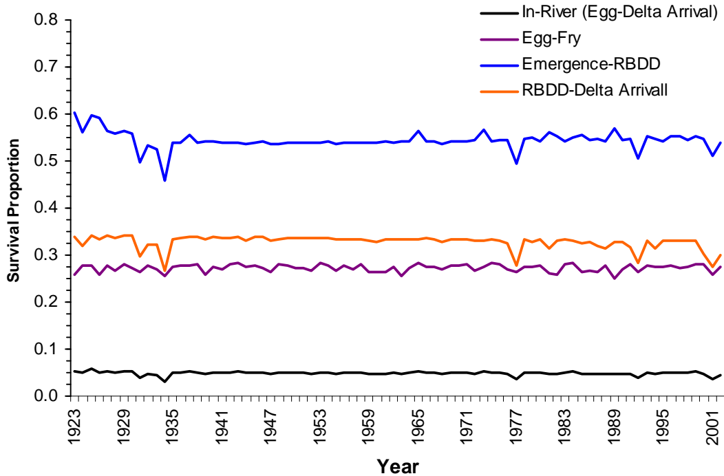
Figure 11-56. Annual winter-run Chinook salmon in-river survival (egg-Delta arrival) for water operation scenario 7.0 and its three components: 1) egg to fry, 2) fry emergence to RBDD, and 3) RBDD to Delta arrival, 1923-2002 from IOS model.
