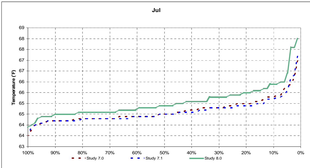
Figure 10-103 Folsom Tailbay End-of-July Exceedence
