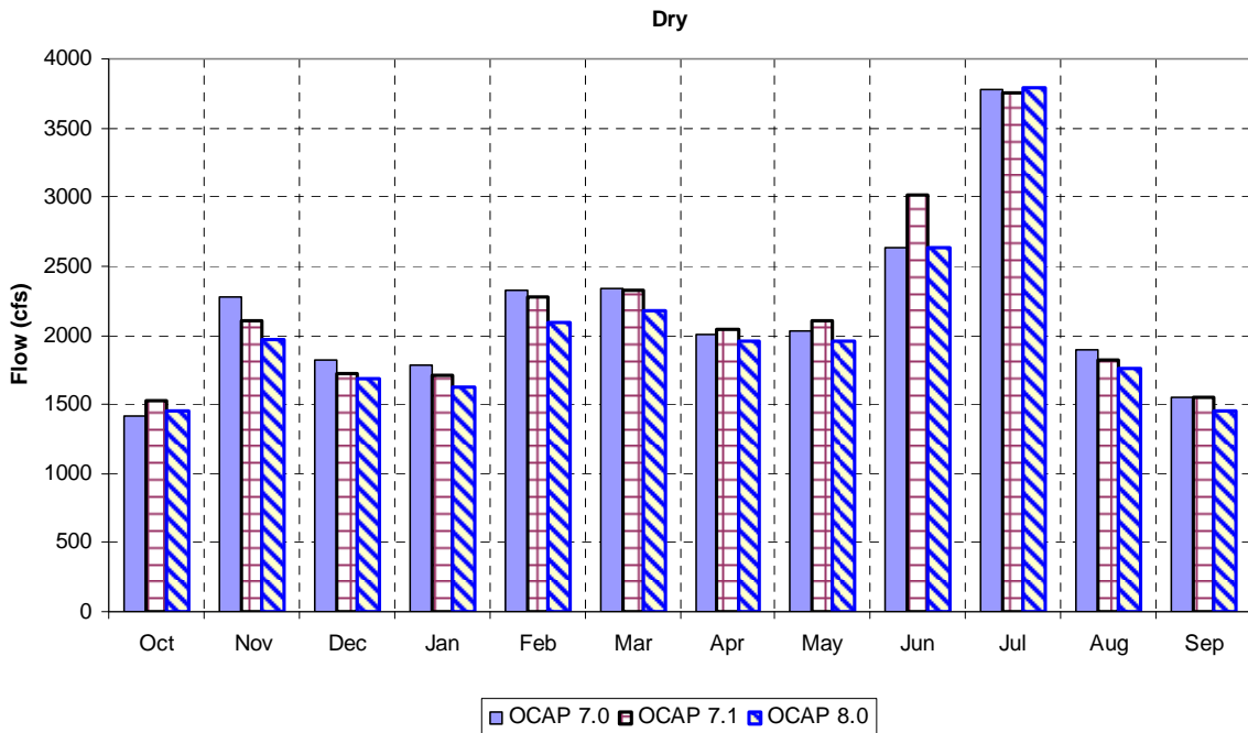
Figure 10-98 Average Dry Year (40-30-30 Classification) Monthly Nimbus Release
