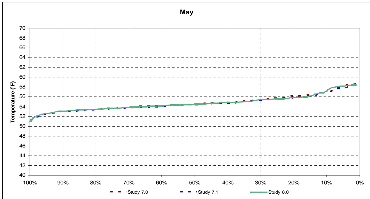
Figure 10-83 Bend Bridge End-of-May Exceedence
