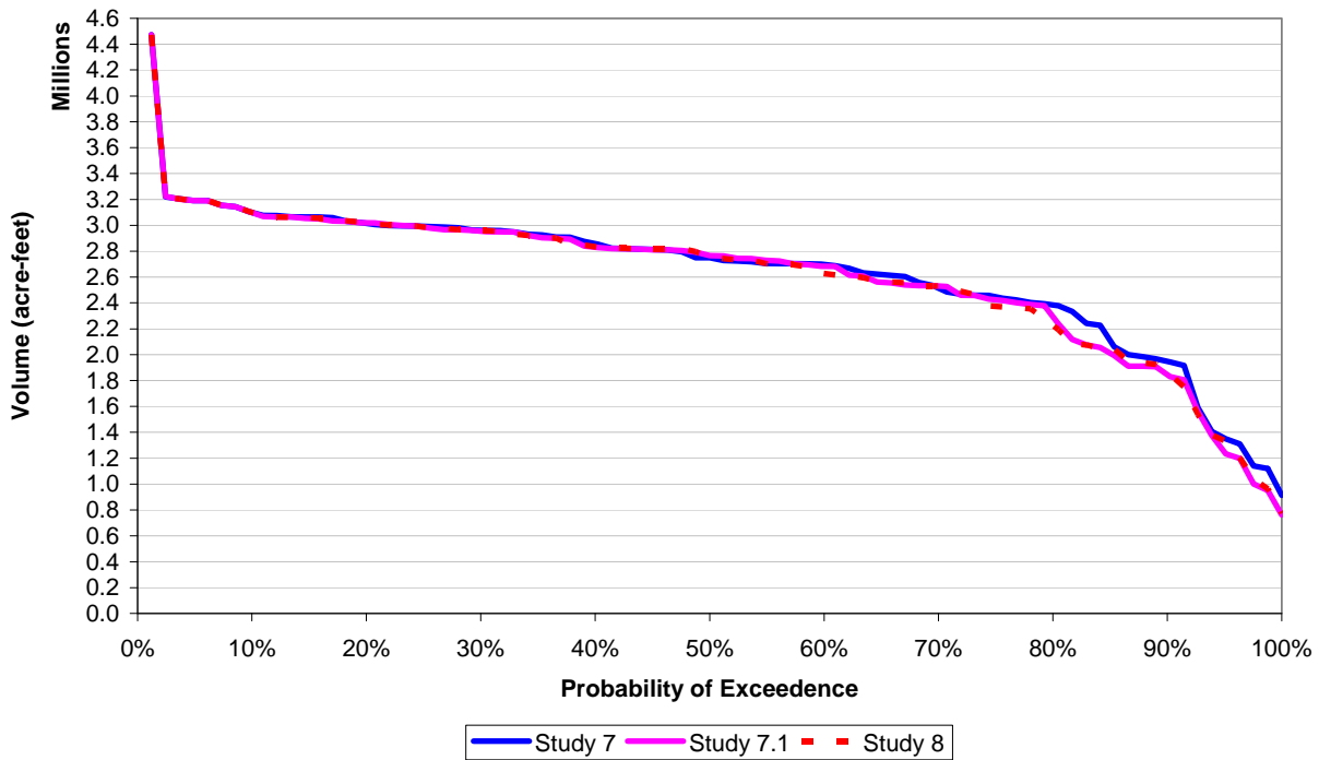
Figure 10-54 52°F index of coldwater availability
