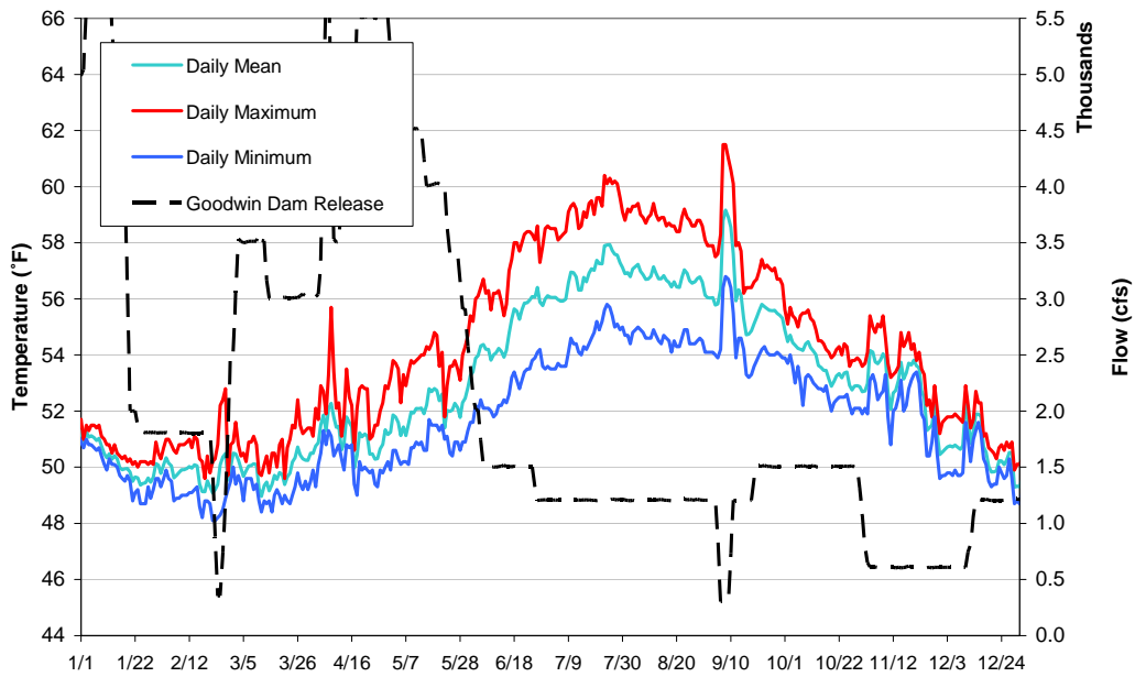
Figure 11-22. Stanislaus River at Orange Blossom Bridge daily temperature fluctuation and flow in a wet water year, actual measured water temperatures (2006).
