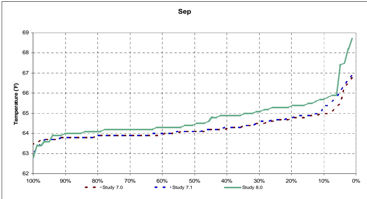
Figure 10-105 Folsom Tailbay End-of-September Exceedence
