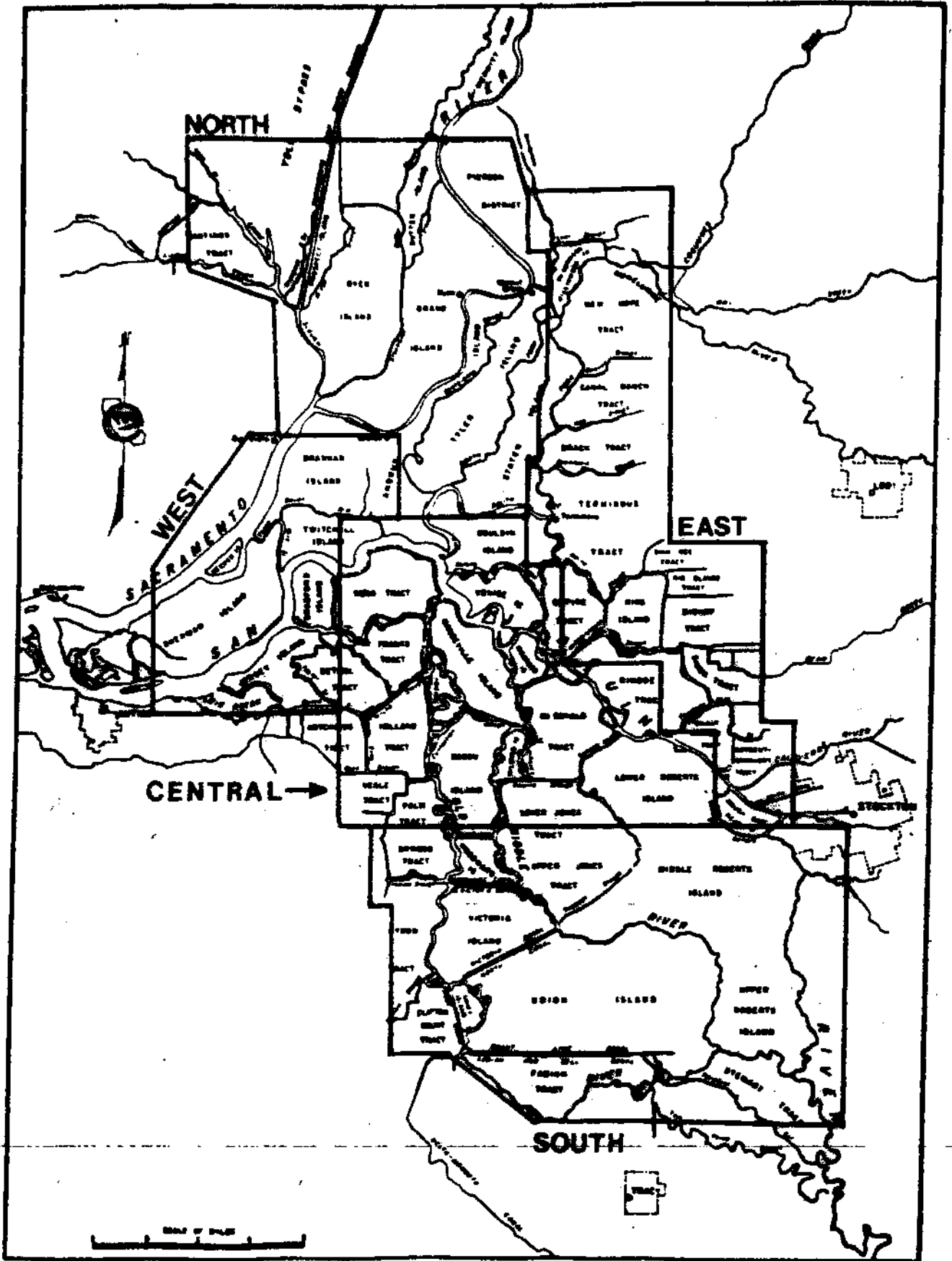
Figure 1. Subareas of the Sacramento-San Joaquin Delta used in the analyses of the resident fish survey data and in which sample sites were chosen according to a random stratified sampling design.
