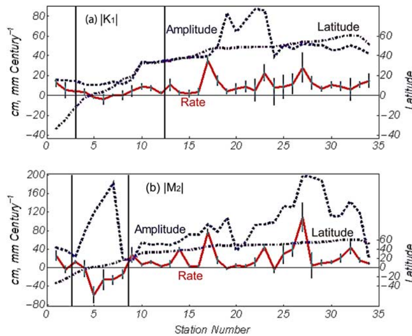
Figure 2. Spatial distribution of amplitude (cm) and amplitude trend ( \text{mm century}^{-1} ) for (a) K_1 and (b) M_2 by station number; station latitude, 95% confidence limits, and amphidrome boundaries are also shown.
