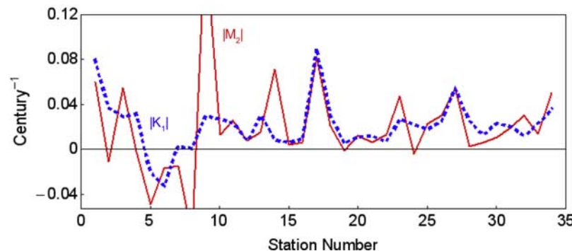
Figure 3. Spatial distribution of relative amplitude trend ( \text{century}^{-1} ) for K_1 and M_2 by station number.
