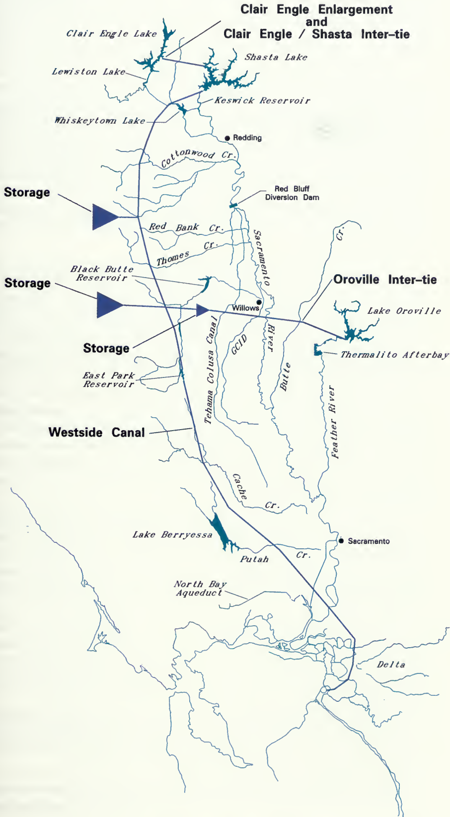
Figure 11-13. Westside Sacramento Valley Storage and Conveyance Concepts
