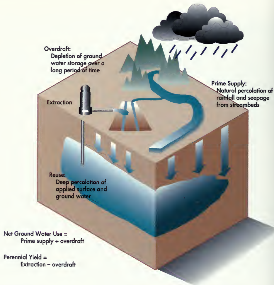
Figure 4-1. Components of Ground Water Use and Sources of Recharge
