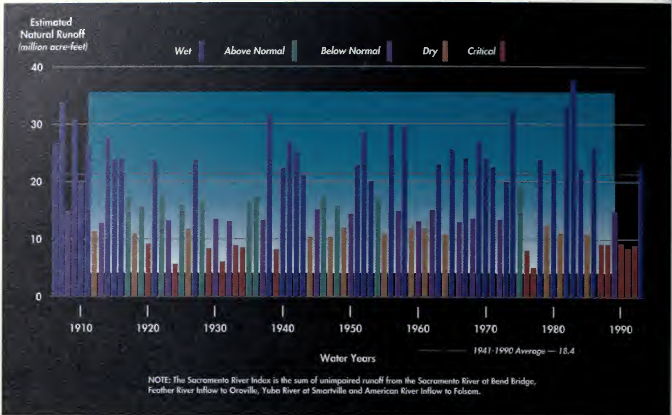
Figure 3-3. The Sacramento River Index Since 1906
