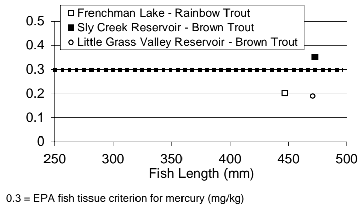
Figure 4. Tissue mercury concentrations in trout from Little Grass Valley Reservoir, Frenchman Lake, and Sly Creek Reservoir
