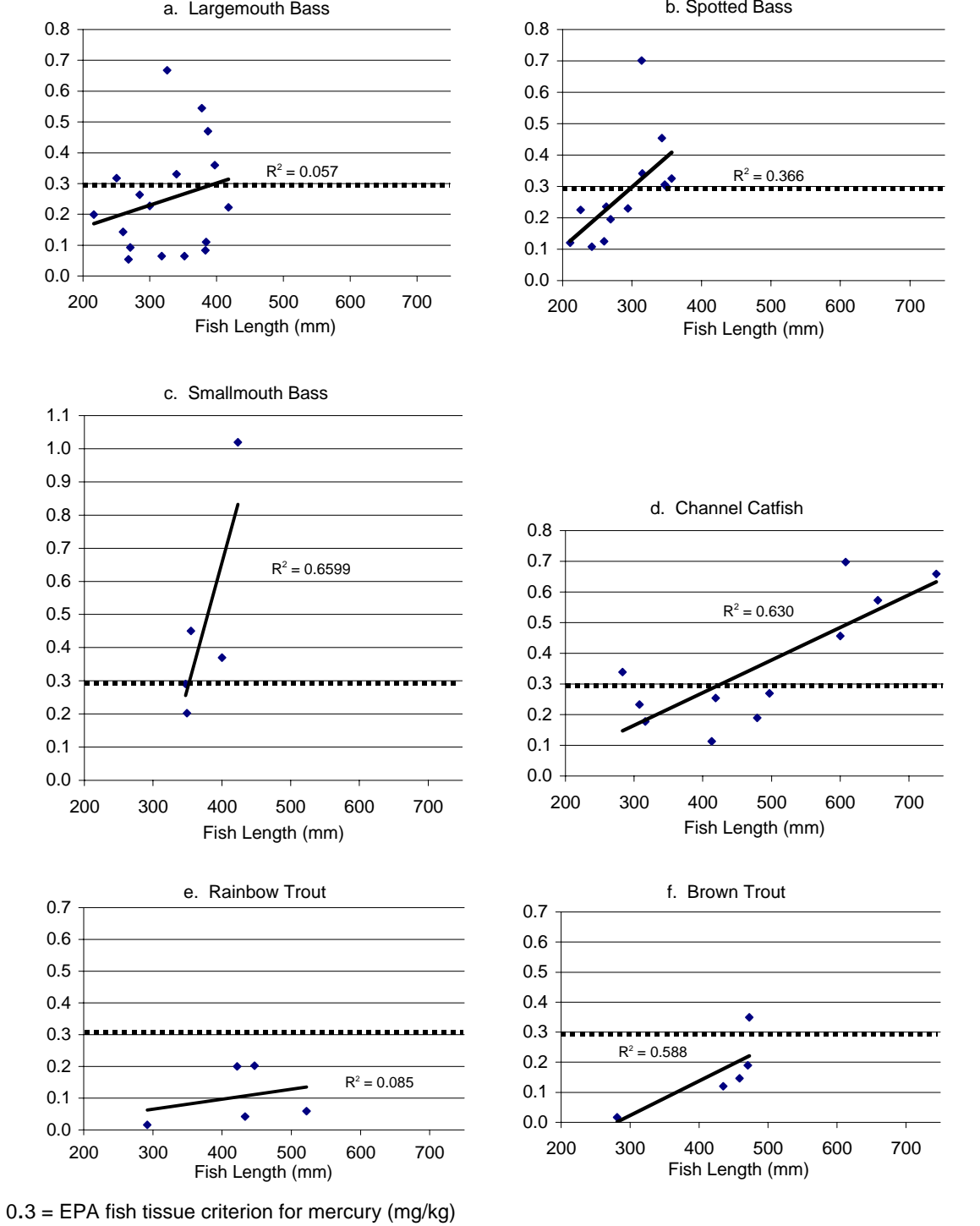
Figure 19. Relationships between mercury concentration and fish size for fish species collected from all sites
