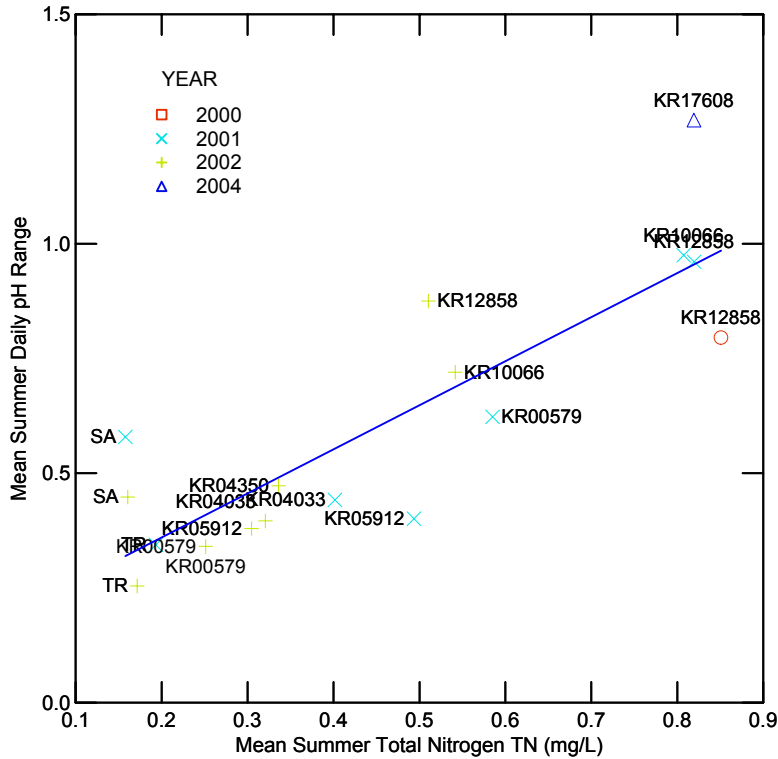
Figure 41. Mean summer daily pH range versus mean summer total nitrogen (TN) for 2000-2004. While there is some scatter, these data show a statistically significant linear relationship ( p < 0.0001 , r^2 = 0.6921 ). The Salmon River site (site code SA) shows a higher pH range than other sites with low TN concentrations. The data in this chart suggest that a mean TN concentration of 0.2 mg/L would hold mean daily pH range to 0.3 or less (Salmon River cite excepted), and a mean TN concentration of 0.5 mg/L or lower would hold mean daily pH range to less than 0.5. Regression equation: \text{MeanDailyRange\_pH} = 0.1679 + 0.9604 \text{ Mean\_TN}
