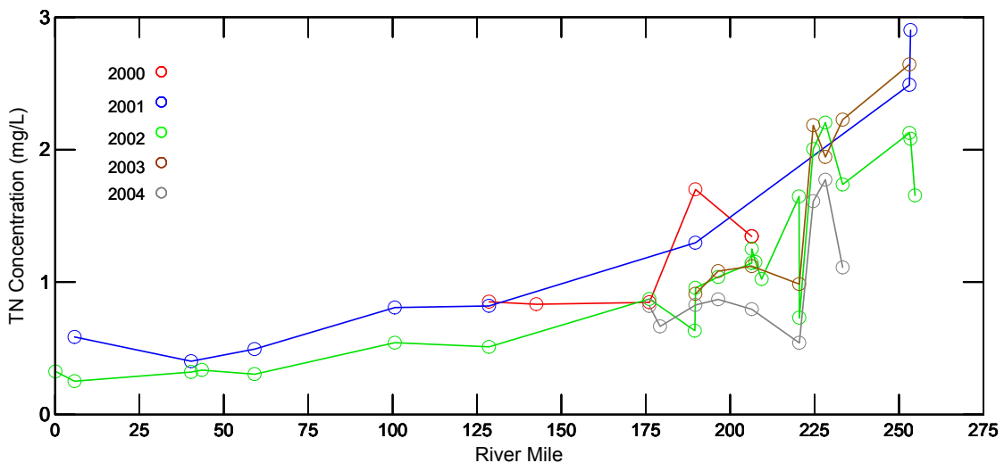
Figure 25. Longitudinal profile of mean summer total nitrogen concentrations in Klamath River mainstem sites for the year 2000-2004 (reservoirs excluded). Sites with less than three measurements in a summer were excluded from this graph.
