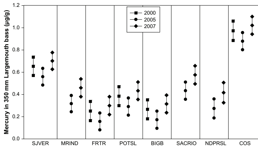
Fig. 6. Predicted mercury concentrations (mean \pm 95% confidence intervals) for 350-mm largemouth bass at eight sites sampled by the Project in 2005 and 2007, and by Davis et al. (2008a,b). Refer to Table 1 for site abbreviations.
