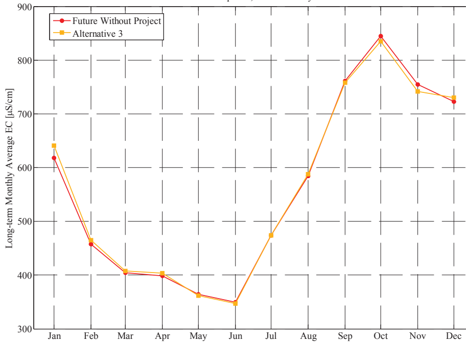
Old River at Rock Slough Salinity Long-term Monthly Average of Simulated EC 2030 Level of Development; Severe Fishery Restrictions
