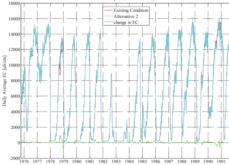
Chippis Island Salinity Daily Average of Simulated EC 2005 Level of Development; Severe Fishery Restrictions
