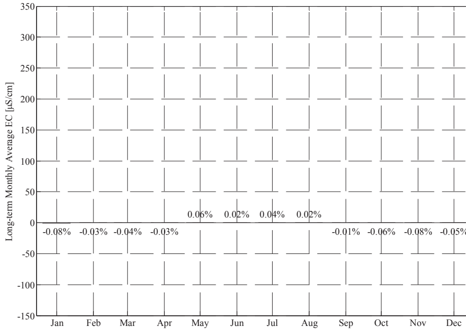
Cache Slough at City of Vallejo Intake Salinity Change from Existing Condition for Long-term Monthly Average of Simulated EC 2005 Level of Development; Severe Fishery Restrictions Alternative 3
