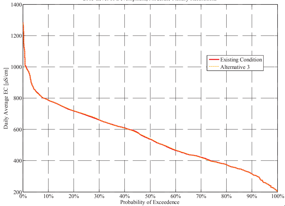
Jones Pumping Plant Salinity Cumulative Distribution of Daily Average of Simulated EC 2005 Level of Development; Moderate Fishery Restrictions
