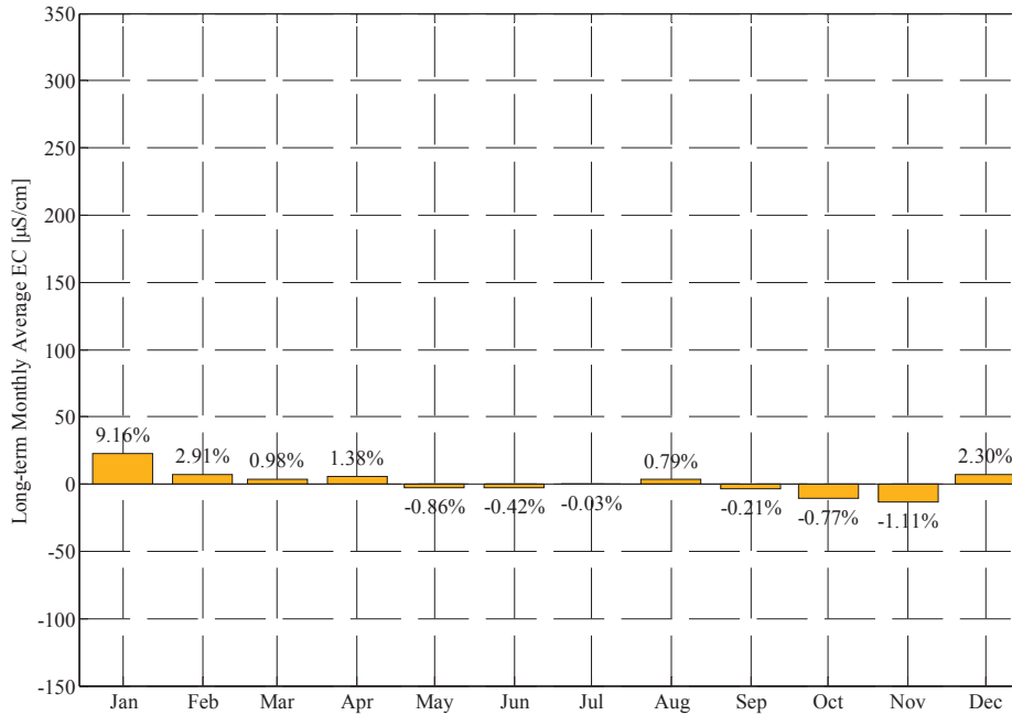
Old River at Rock Slough Salinity Change from Future Without Project for Long-term Monthly Average of Simulated EC 2030 Level of Development; Severe Fishery Restrictions Alternative 3
