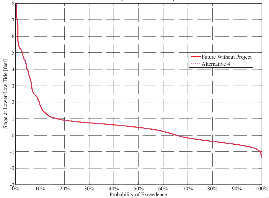
Doughty Cut above Grant Line Canal Barrier Water Level at Lower-Low Tide 2030 Level of Development; Moderate Fishery Restrictions
