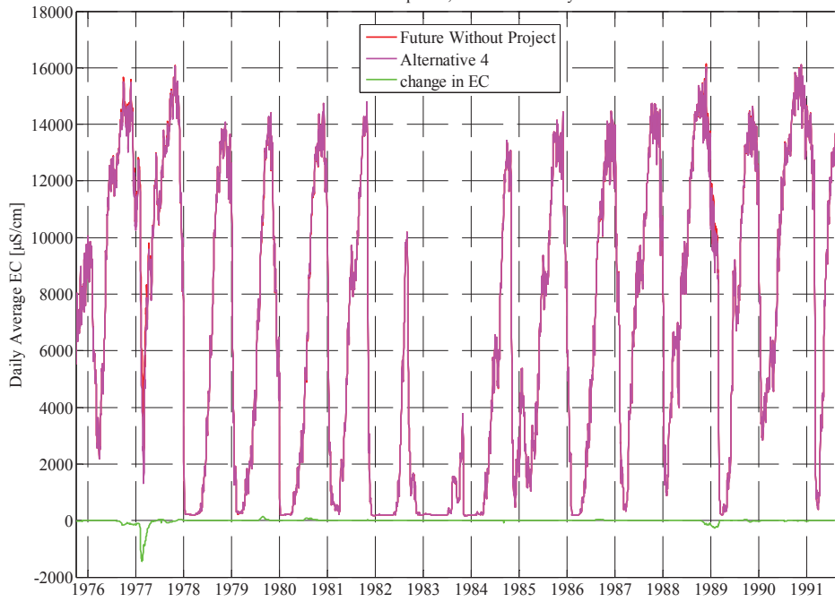
Chippis Island Salinity Daily Average of Simulated EC 2030 Level of Development; Moderate Fishery Restrictions
