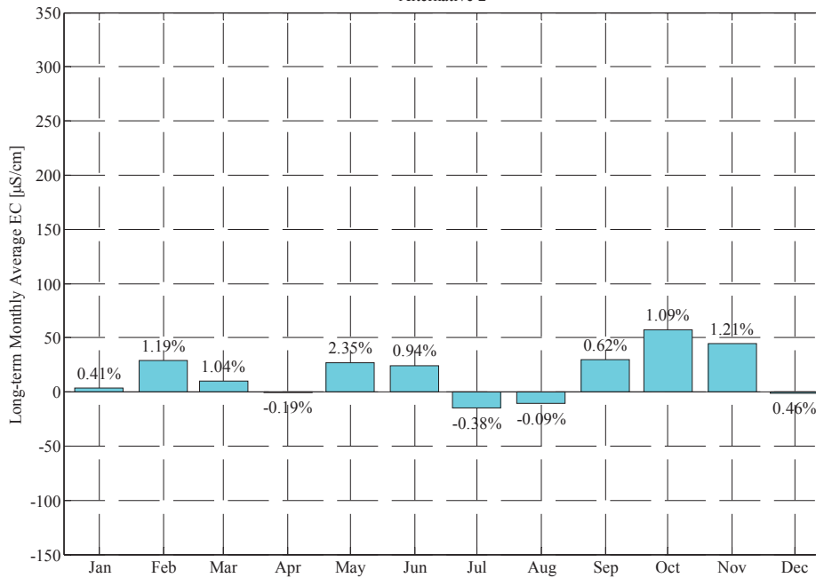
Collinsville Salinity Change from Existing Condition for Long-term Monthly Average of Simulated EC 2005 Level of Development; Severe Fishery Restrictions Alternative 2
