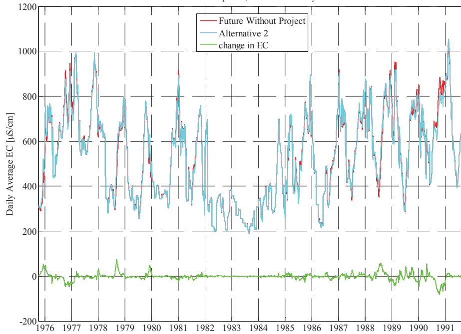
Clifton Court Forebay Entrance Salinity Daily Average of Simulated EC 2030 Level of Development; Moderate Fishery Restrictions
