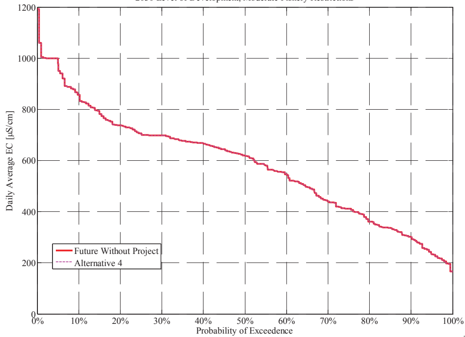
San Joaquin River at Vernalis Salinity Cumulative Distribution of Daily Average of Simulated EC 2030 Level of Development; Moderate Fishery Restrictions
