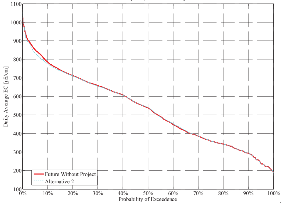
Clifton Court Forebay Entrance Salinity Cumulative Distribution of Daily Average of Simulated EC 2030 Level of Development; Moderate Fishery Restrictions
