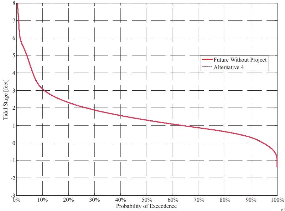
Doughty Cut above Grant Line Canal Barrier Tidal Water Level (simulated every 15 minutes) 2030 Level of Development; Moderate Fishery Restrictions
