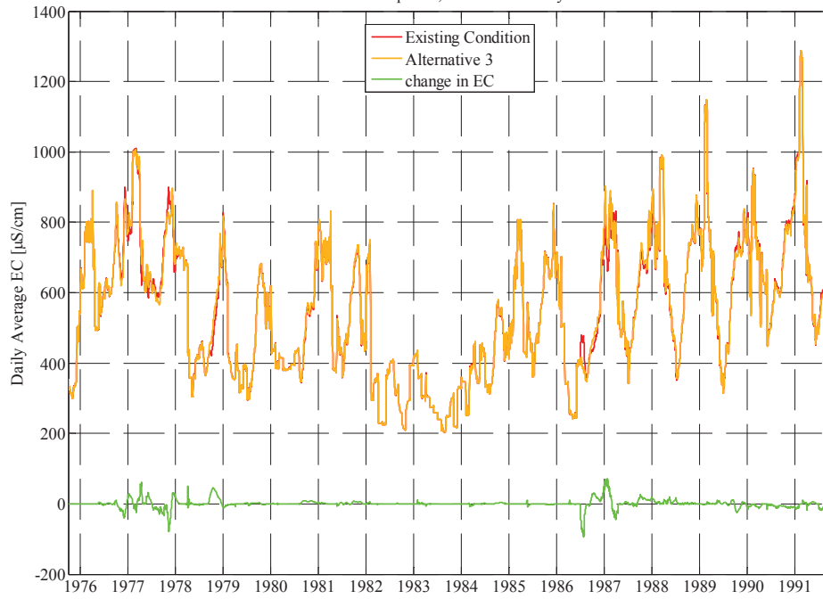
Jones Pumping Plant Salinity Daily Average of Simulated EC 2005 Level of Development; Moderate Fishery Restrictions
