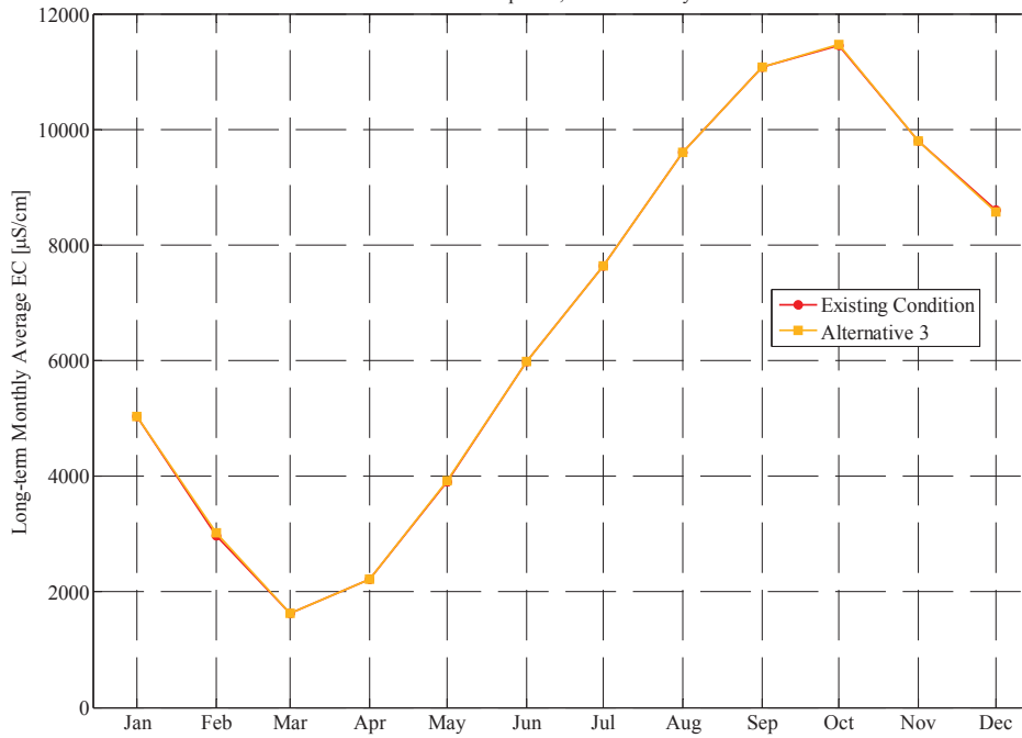
Chippis Island Salinity Long-term Monthly Average of Simulated EC 2005 Level of Development; Severe Fishery Restrictions
