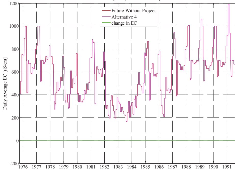
San Joaquin River at Vernalis Salinity Daily Average of Simulated EC 2030 Level of Development; Moderate Fishery Restrictions
