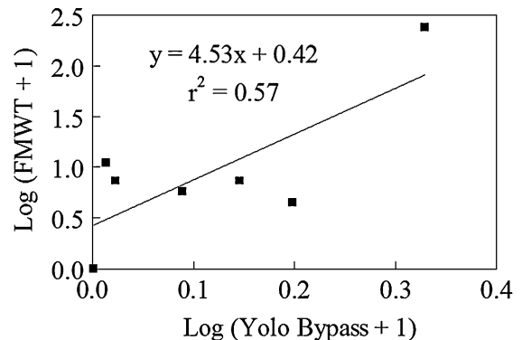
Figure 5. Relationship between production of age-0 splittail in Yolo Bypass compared to overall system-wide production as estimated from the California Department of Fish and Game's Fall Midwater Trawl Survey (FMWT).
