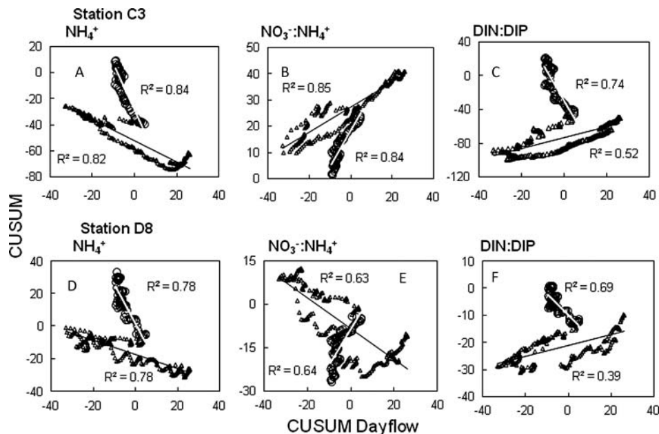
Figure 8 Correlation between the CUSUM trend in dayflow and the CUSUMS of (A) \text{NH}_4^+ at C3; (B) ratio of \text{NO}_3^-:\text{NH}_4^+ at C3; (C) ratio of DIN:DIP at C3; (D) \text{NH}_4^+ at D8; (E) ratio of \text{NO}_3^-:\text{NH}_4^+ at D8; (F) ratio of DIN:DIP at D8. All trends are for the period since the establishment of the wastewater treatment facility in the upper Sacramento (1984–2005). For each panel, the open triangles are for 1984–1999 and the closed circles are for the POD years, 2000–2005.
