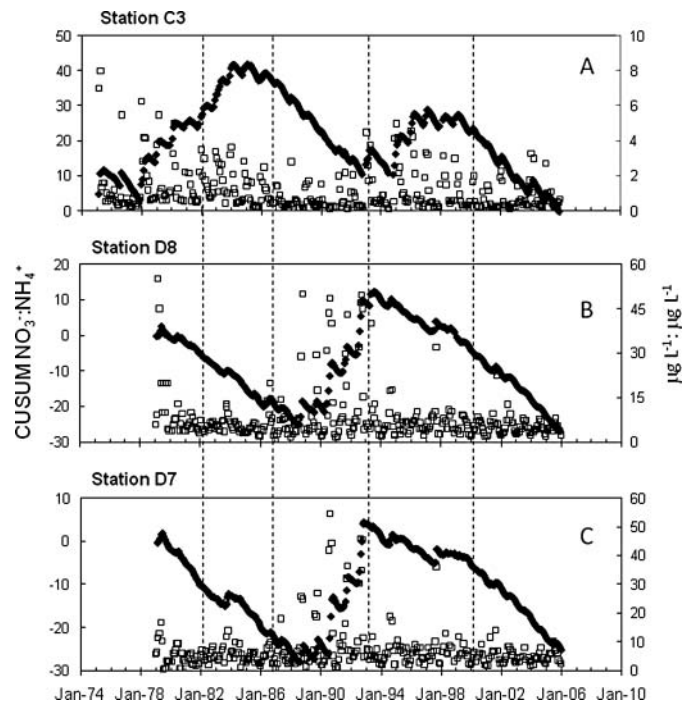
Figure 4 CUSUM values (primary axis, filled diamonds) as a function of time for the ratio of nitrate:ammonium ( \text{NO}_3^-:\text{NH}_4^+ ) concentrations for (A) the upper Sacramento at station C3; (B) and (C) Suisun Bay at stations D8 and D7. The secondary axis (open squares) for all panels gives the actual data in \mu\text{g L}^{-1}:\mu\text{g L}^{-1} . The vertical dashed lines are guides to delineate the major periods discussed in the text.
