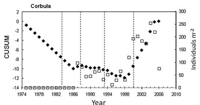
Figure 13 CUSUM values (primary axis, filled diamonds) as a function of time for the clam Corbula amurensis . The secondary axis (open squares) gives the actual abundance data in individuals m^{-2} . The vertical dashed lines are guides to delineate the major periods discussed in text.
