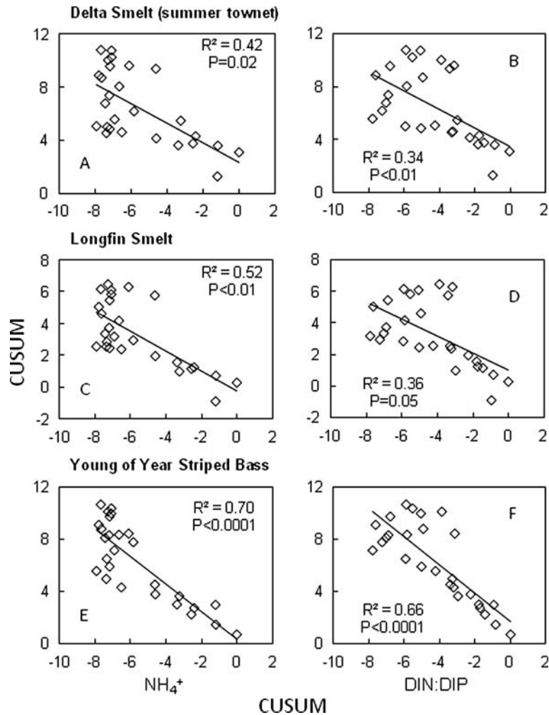
Figure 19 Correlations between the CUSUM trends in \text{NH}_4^+ and DIN:DIP at station D8 in Suisun Bay and CUSUM trends in delta smelt (panels A–B; summer towntnet index), longfin smelt (panels C–D), and young-of-the-year striped bass (panels E–F). All correlations cover the period 1975–2005.
