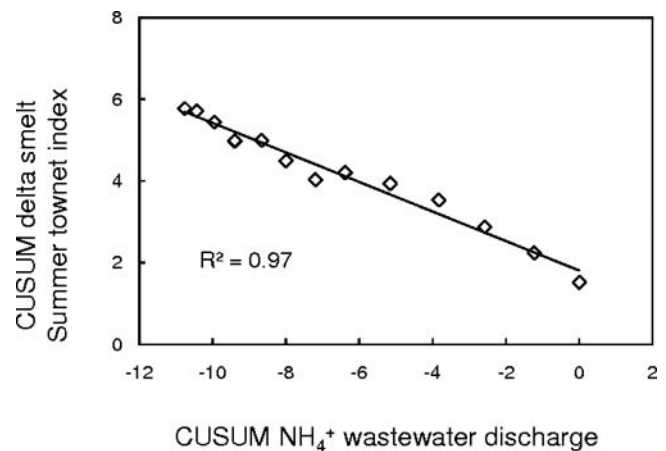
Figure 22 Correlation between the trend in CUSUM in ammonium concentration in wastewater discharge in the upper Sacramento River and the trend in CUSUM delta smelt, estimated from the summer tounet index.
