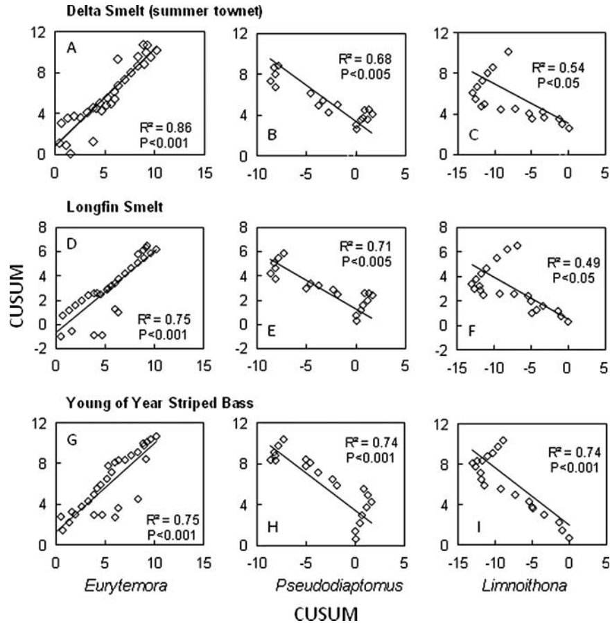
Figure 21 Correlations between the CUSUM trends in the copepods Eurytemora affinis , Pseudodiaptomus forbesi and Limnoithona tetraspina in Suisun Bay and CUSUM trends in delta smelt (panels A–C; summer tounet index), longfin smelt (panels D–F) and young-of-the-year striped bass (panels G–I). All correlations cover the period 1975–2005 for E. affinis , and 1987–2005 for the other copepods.
