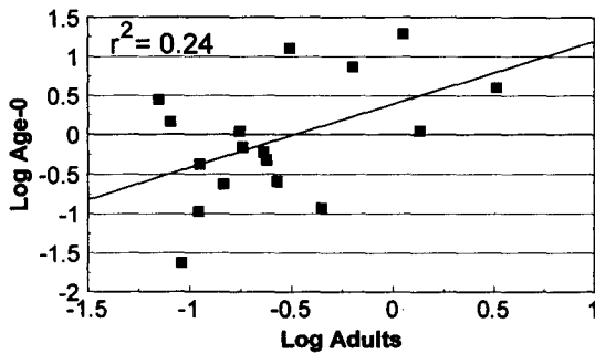
FIGURE 5.—Suisun Marsh survey stock–recruitment relationship ( \log_{10} ) for adult versus age-0 splittails.
