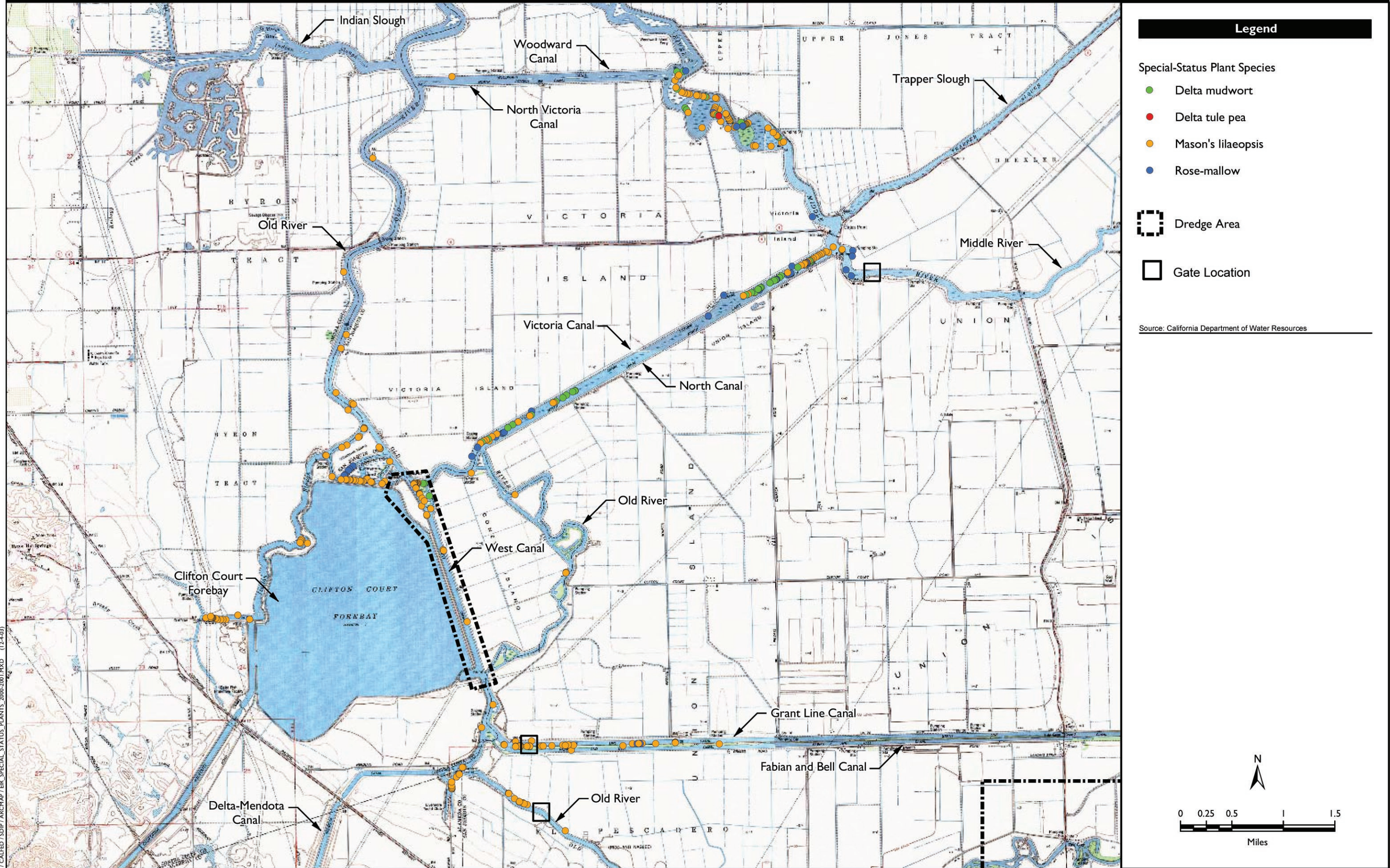
Figure 6.2-10. Locations of Special-Status Plants in the Study Area
