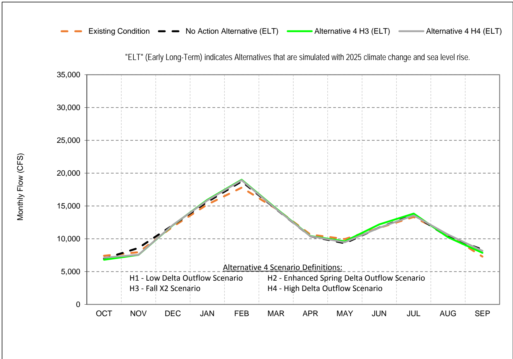
Figure 4.3.2-2 Sacramento River Flow at Bend Bridge for Alternative 4A, Long-Term Average
