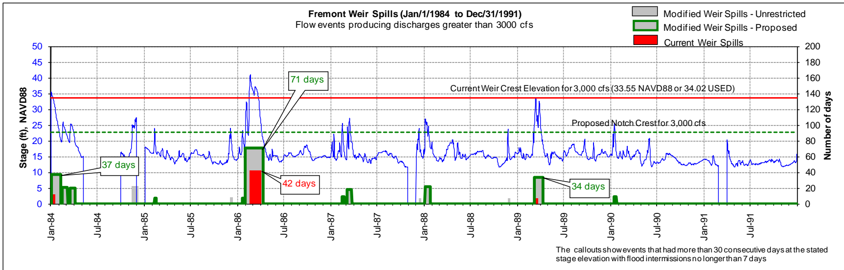
1 2 Figure 4-267. Events producing discharges greater than 3000 cfs for more than 30 days (1984-1991)
