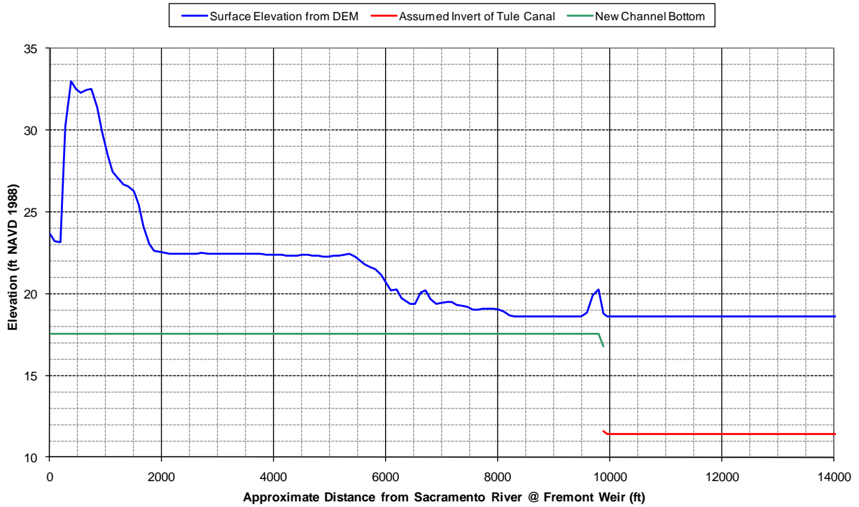
1 2 Figure 4-20. Yolo Bypass Profile from Sacramento River at Fremont Weir to Tule Canal
