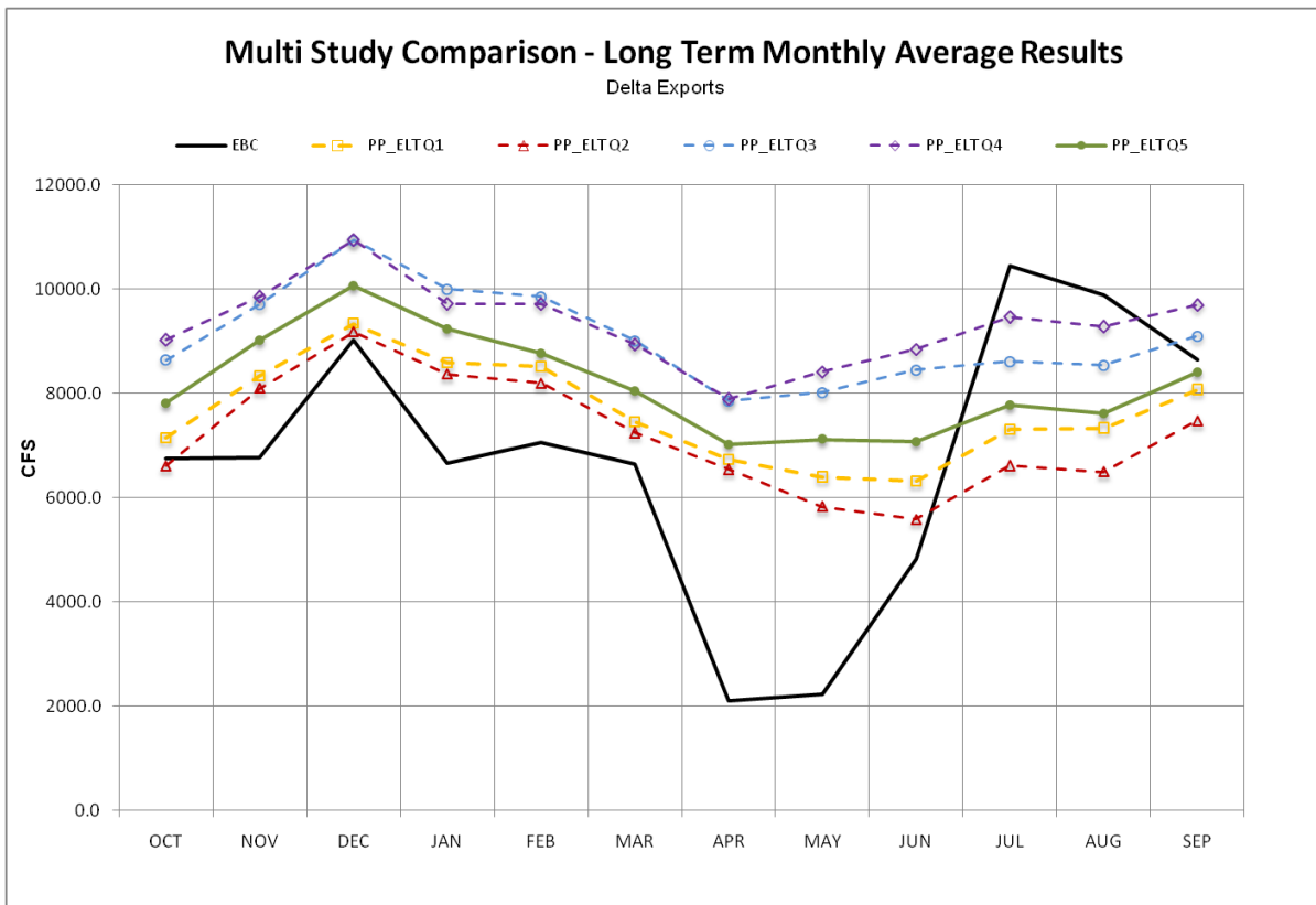
4 5 Figure 3-14. Seasonal Export uncertainty for the Alternative 1 Early Long-Term scenario
