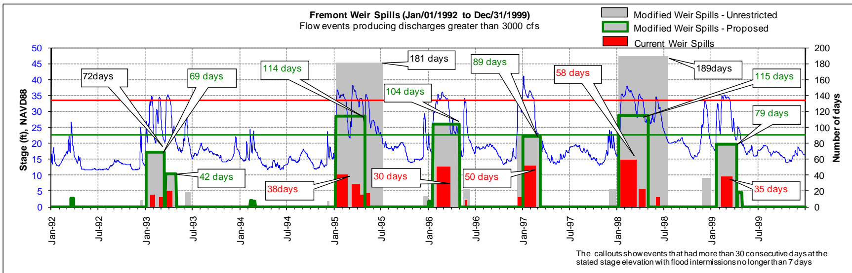
3 4 Figure 4-278. Events producing discharges greater than 3000 cfs for more than 30 days (1992-1999)
