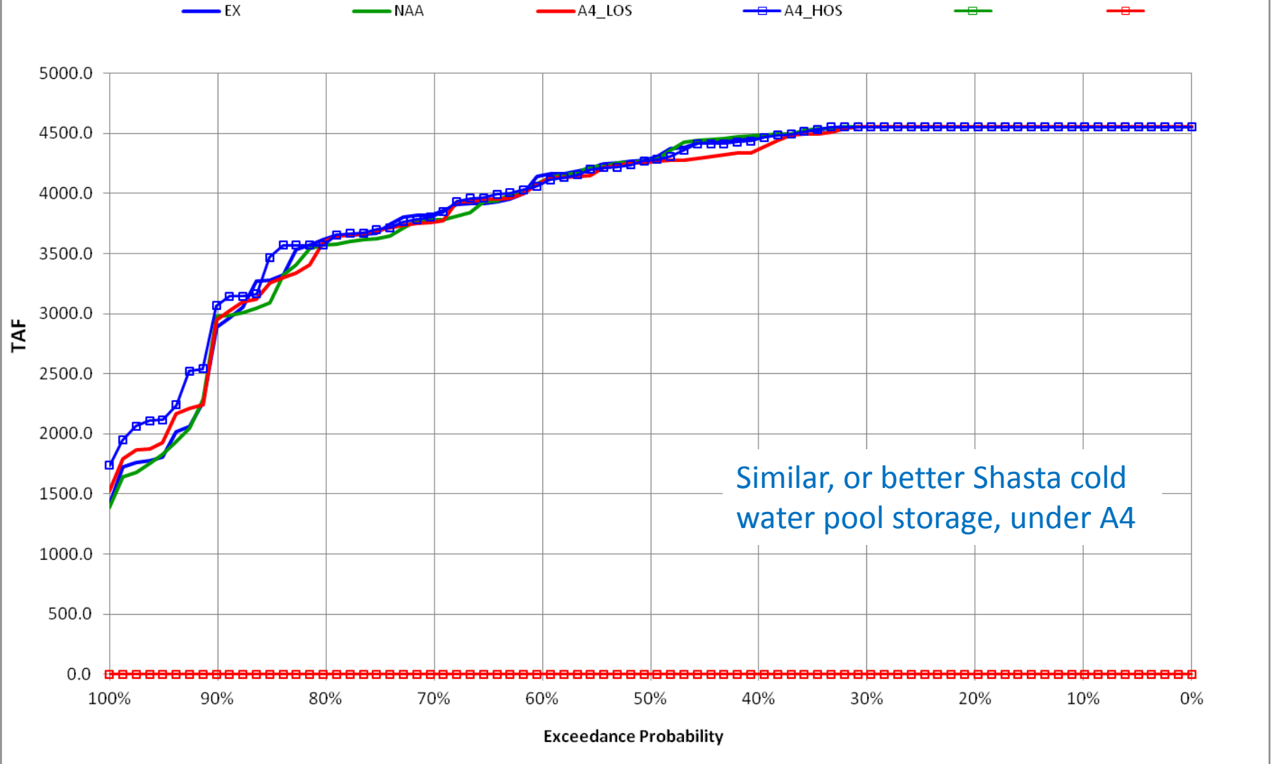
Results Exceedance Probability Shasta MAY
