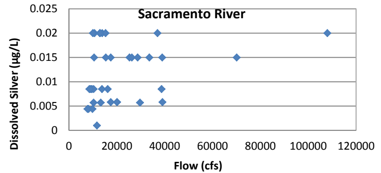
1 Figure 1. Association of dissolved trace metals with Sacramento River flow at Freeport, 1992-2010
