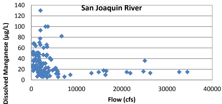
6 Figure 3. Association of dissolved trace metals with San Joaquin River flow at Vernalis, 1992- 7 2001.
