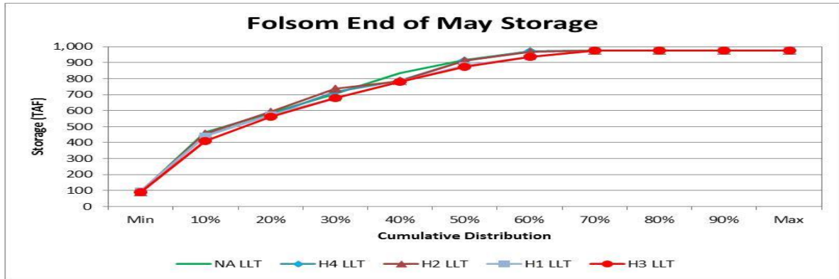
4 5 Figure 6b. Folsom Reservoir End-of-May Storage for H1 through H4 for WY 1922–2003
