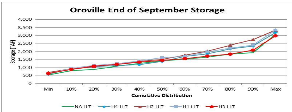
7 8 Figure 5c. Oroville Reservoir End-of-September Storage for H1 through H4 for WY 1922–2003
