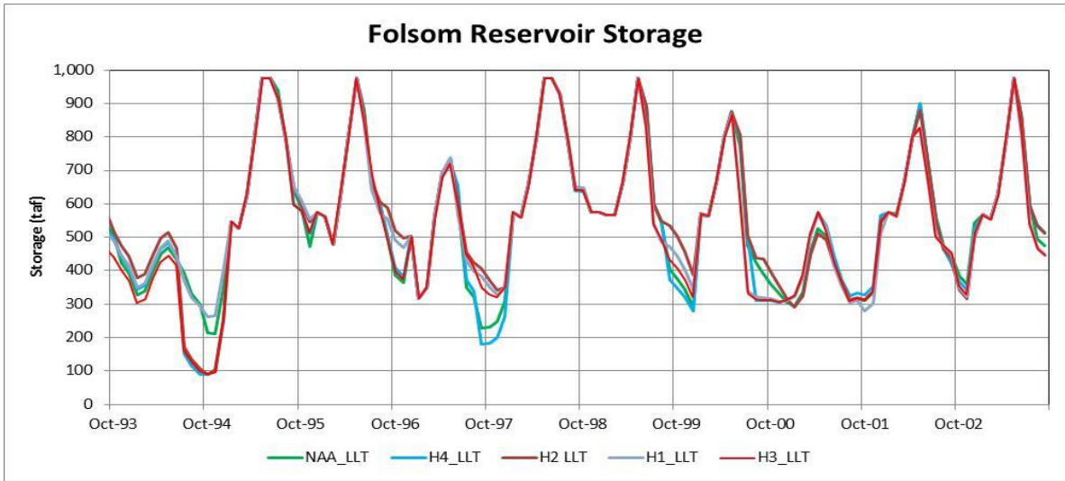
1 2 Figure 6a. CALSIM-Simulated Folsom Reservoir Storage (taf) for H1 through H4 for WY 1994–2003
