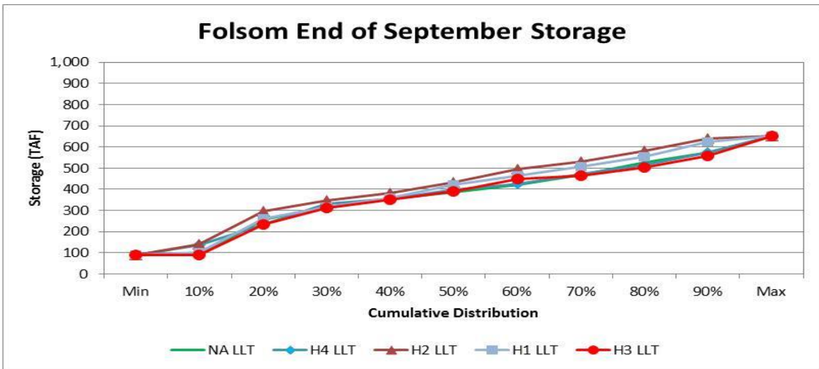
7 8 Figure 6c. Folsom Reservoir End-of-September Storage for H1 through H4 for WY 1922–2003
