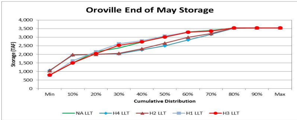
4 5 Figure 5b. Oroville Reservoir End-of-May Storage for H1 through H4 for WY 1922–2003
