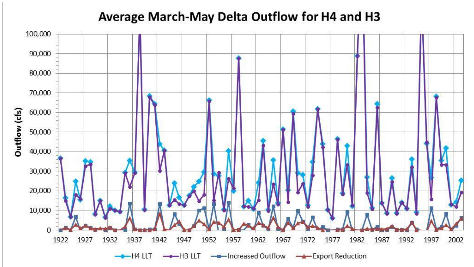
Figure 1. CALSIM-Simulated Average March-May Delta Outflow for H3 and H4 Cases for WY 1922-2003 at the LLT Timeframe (2060)
