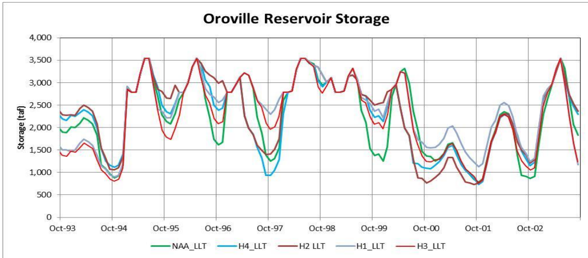
1 2 Figure 5a. CALSIM-Simulated Oroville Reservoir Storage (taf) for H1 through H4 for WY 1994–2003
