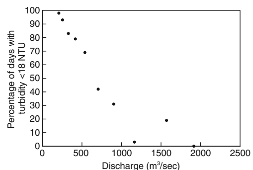
Fig. 4 Relationship of the percentage of days with turbidity <18 NTU with discharge (m 3 /s) at Rio Vista
