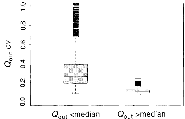
FIG. 8. Coefficient of variation (cv, expressed as a fraction) in daily Q_{out} (net Delta outflow) estimated by propagating uncorrelated fluctuations of 10% in each of Q_{tot} , Q_{prec} , Q_{depl} , and Q_{exp} ( Q_{tot} , total Delta inflow; Q_{prec} , runoff within the Delta; Q_{depl} , depletion [consumption within the Delta]; Q_{exp} , exports). Values for each term were taken from the DAYFLOW data set for 1956–1991. Median Q_{out} during this period was 356 m^3/s . The center horizontal line in each box is the median. The lower and upper edges of each box, called hinges , mark the first and third quartiles. The whiskers , dashed lines emanating from each box, show the range of values falling within 1.5 times the interquartile distance from the nearest hinge. The remaining horizontal lines mark outside values that fall beyond the whiskers.
