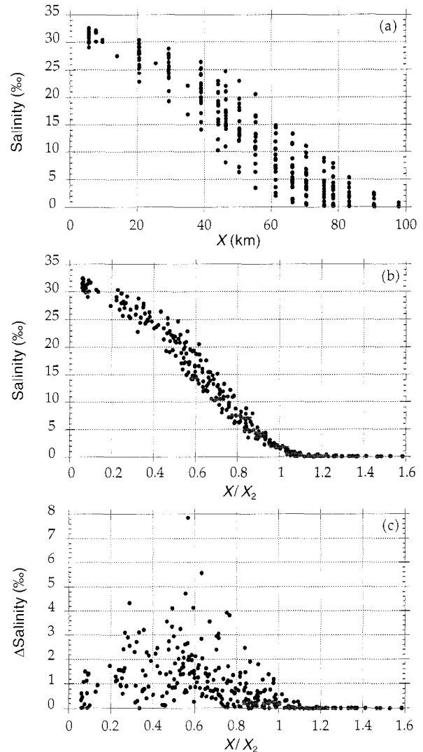
FIG. 2. (a) Vertically averaged salinity vs. distance from the Golden Gate ( X ) along the axis of the estuary, based on salinity profiles collected from January 1990 through February 1992; (b) the same data as in (a), but distances from the Golden Gate are scaled by X_2 ; (c) bottom minus top salinity values for each vertical profile vs. distance from the Golden Gate, again scaled by X_2 .
