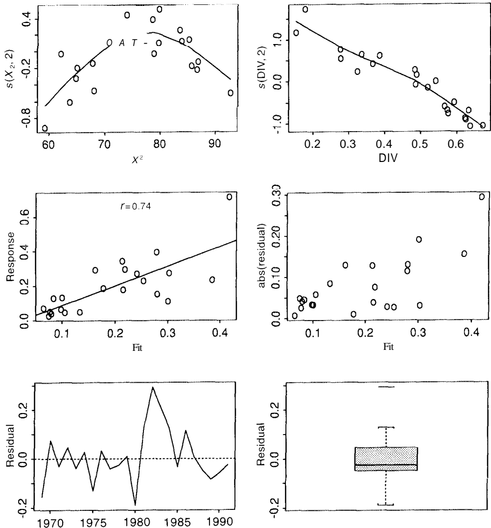
FIG. 7. Diagnostics for generalized additive model of striped bass survival index with link function g = \log and variance function V = I : top panels , partial residual plots for X_2 and DIV (Freshwater diversion). [ s(X_2, 2) and s(DIV, 2) refer to smoothing splines with two degrees of freedom]; middle panels , response and absolute value (abs) of residuals vs. fitted values from the survival model; bottom panels , time and box plots of residuals (see Fig. 8 caption for a description of box plot).
