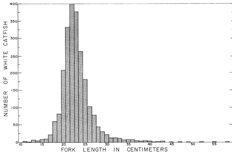
FIGURE 7. Length frequency of all white catfish taken with gill nets.
