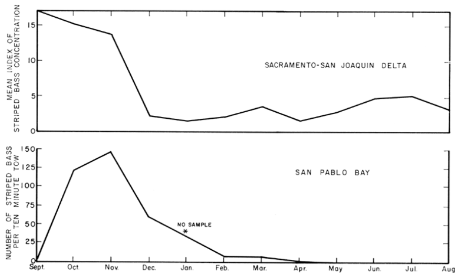
FIGURE 4. Comparison of the monthly mean index of concentration (see text, p. 44) in the Delta and the monthly average otter trawl catches in San Pablo Bay (Ganssle, 1966) of the 1963 year-class striped bass, September 1963 to August 1964.
