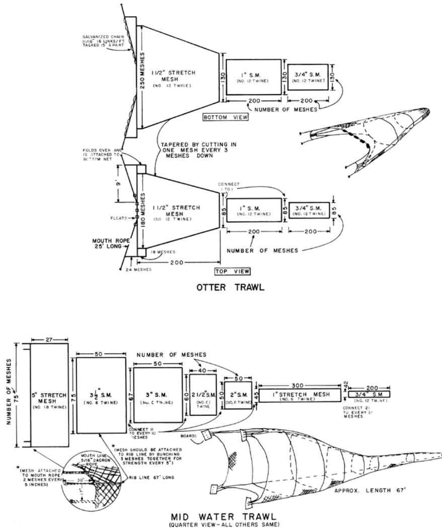
FIGURE 2. Diagram showing construction of otter trawl and midwater trawl used in this study.
