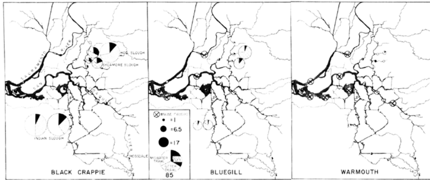
FIGURE 3. Distribution of black crappie, bluegill, and warmouth in the Sacramento-San Joaquin Delta. The area of each circle is proportional to the sum of the mean catches of the otter trawl, midwater trawl, and gill net.
