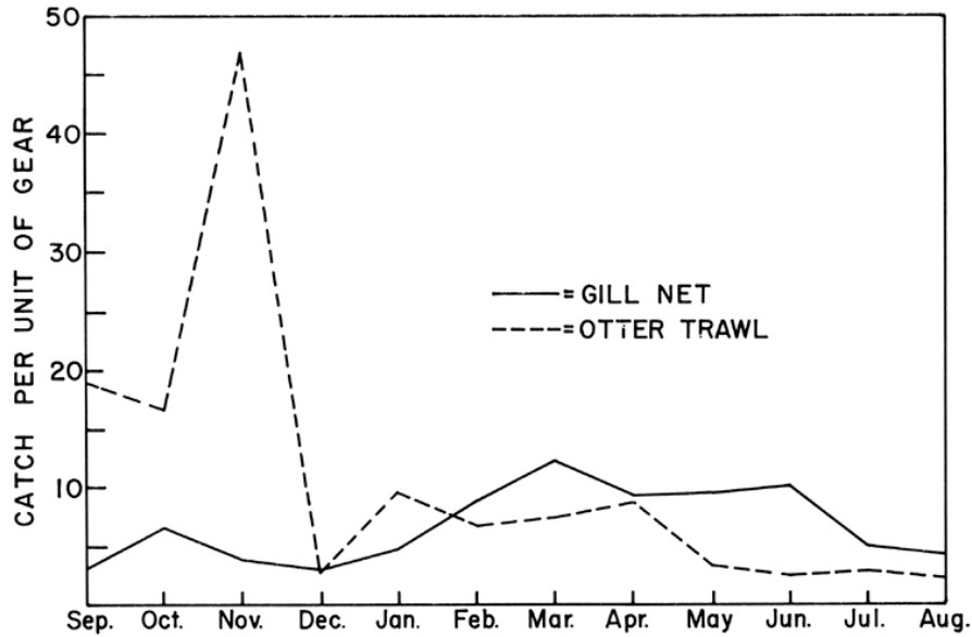
FIGURE 6. Mean monthly catch of juvenile and adult white catfish taken with otter trawl and gill net.
