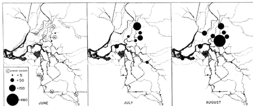
FIGURE 5. Concentrations of American shad of the 1964 year-class in the Sacramento-San Joaquin Delta between June 1964 and August 1964. The area of each circle represents the mean number of shad caught in a 10-minute tow with the midwater trawl.
