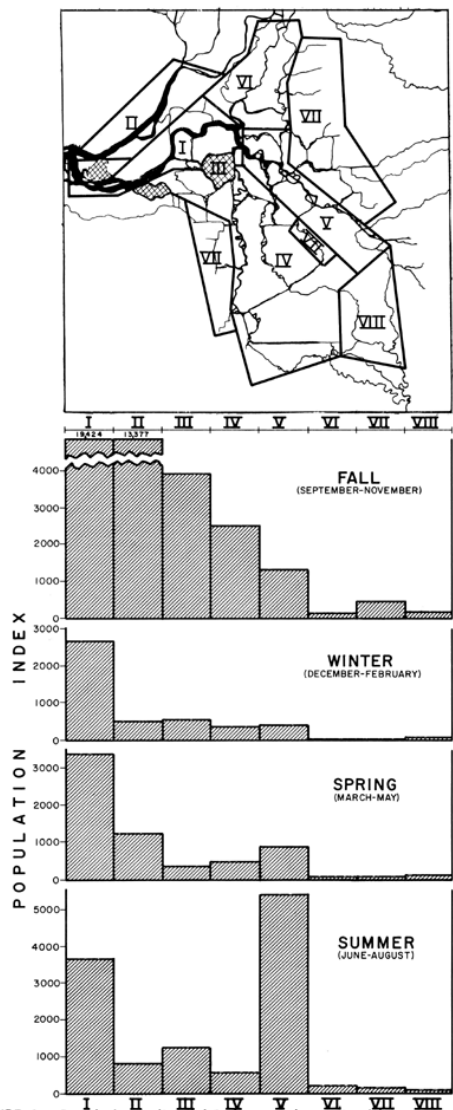
FIGURE 8. Population indices of 1963 year-class striped bass, 1963-1964.
