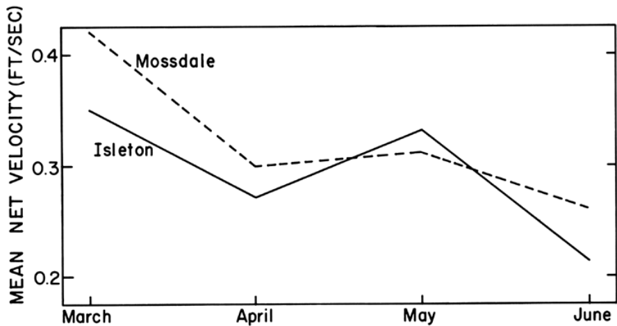
FIGURE 6. Comparison of mean net velocity of flow in the Sacramento River at Isleton and in the San Joaquin River at Mosssdale, based on monthly net flows estimated by the California Dept. of Water Resources.
