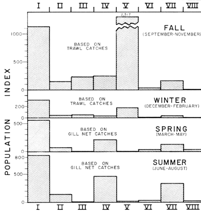
FIGURE 7. Population indices of 1962 year-class striped bass, 1963-1964
