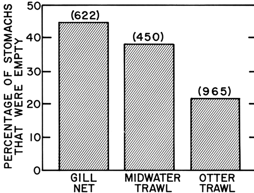
FIGURE 2. Percentage of juvenile bass stomachs that were empty compared to method by which the bass were collected. Numbers of stomachs examined are in parentheses.
