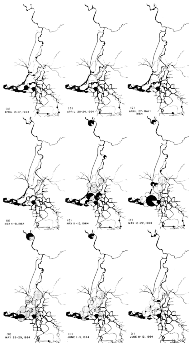
FIGURE 3. Weekly mean eggs and larvae per tow in 1964. For scale and legend see Figure 2.
