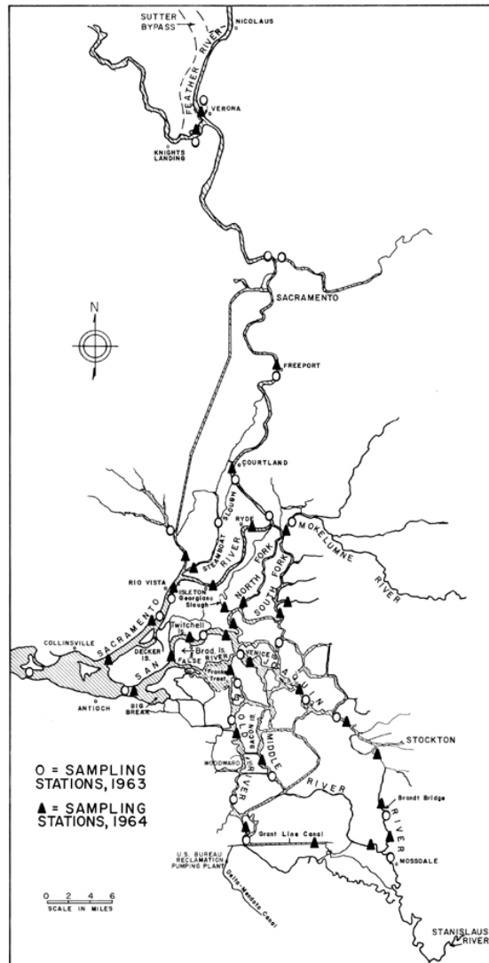
FIGURE 1. Striped bass egg and larva sampling stations.
