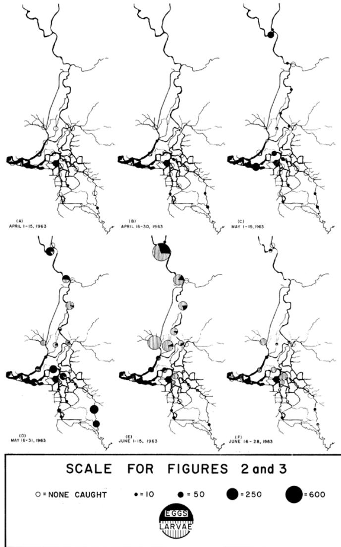
FIGURE 2. Semi-monthly mean eggs and larvae per tow in 1963.
