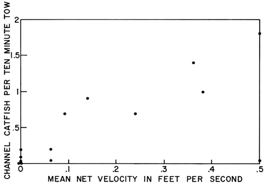
FIGURE 2. Comparison of the mean annual catch of channel catfish taken by otter trawl with the mean annual net velocity of flow at our sampling stations. Radtke (see p. 24) describes net velocity of flow.
