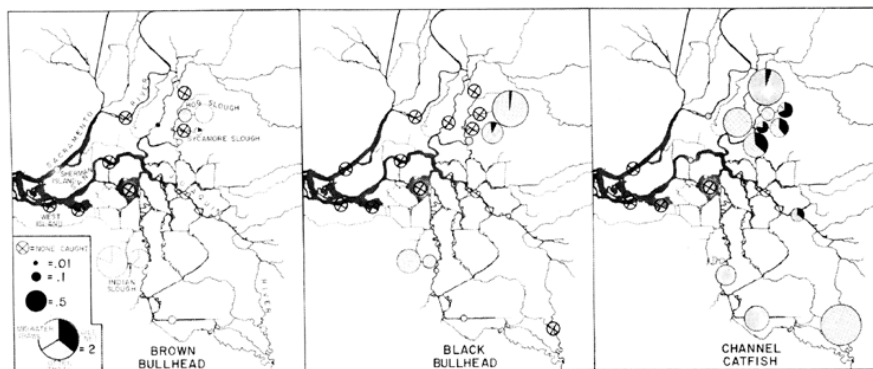
FIGURE 1. Distribution of brown bullheads, black bullheads, and channel catfish. The area of each circle is proportional to the sum of the mean catch of fish taken with the otter trawl, midwater trawl, and gill net.
