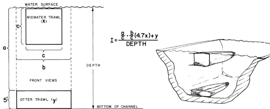
FIGURE 2. Index of concentration "I" where:
