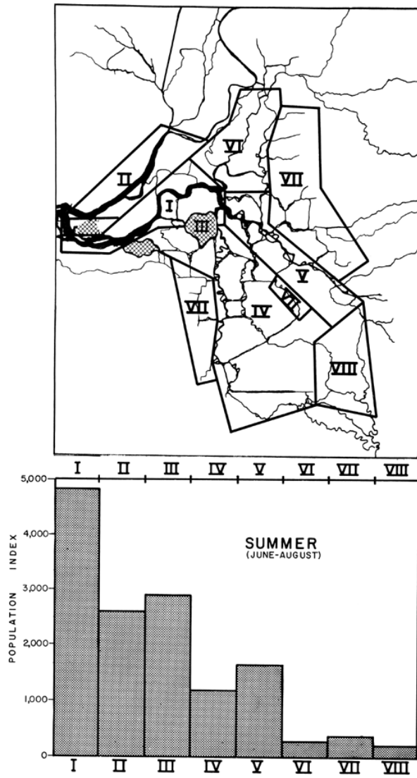
FIGURE 9. Population indices of 1964 year-class striped bass, summer 1964.
