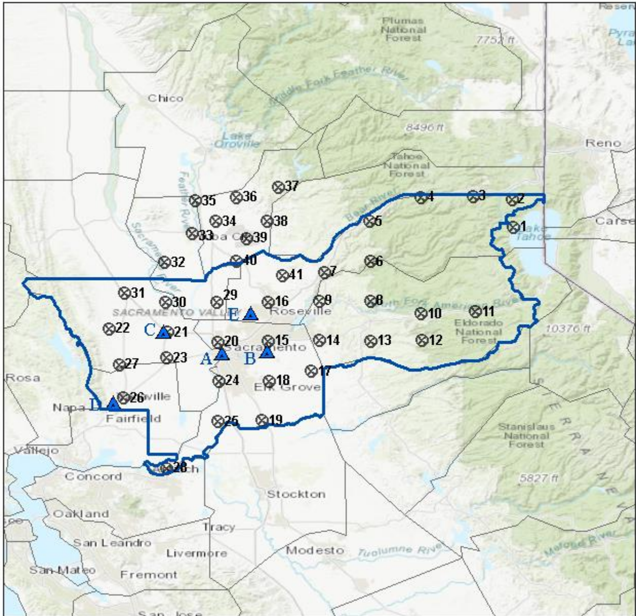
Figure 3. Locations of five strategic area Projects A-E used in the screening modeling, along with the 41 hypothetical projects used in the minor project analysis with outline of the SFNA boundary.
