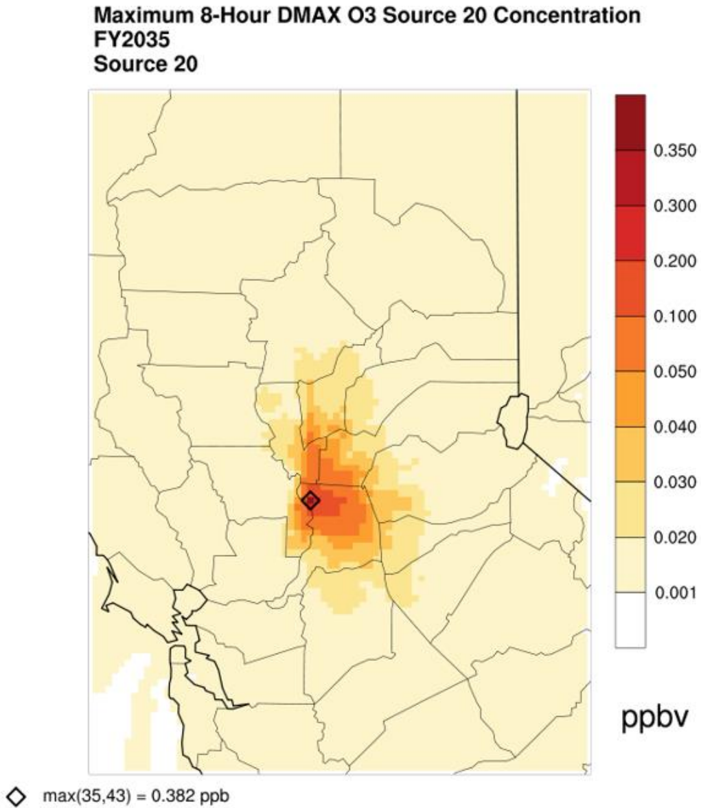
Figure B-5. Map of the incremental highest MDA8 ozone concentrations (ppb) due to emissions from hypothetical source 20.
