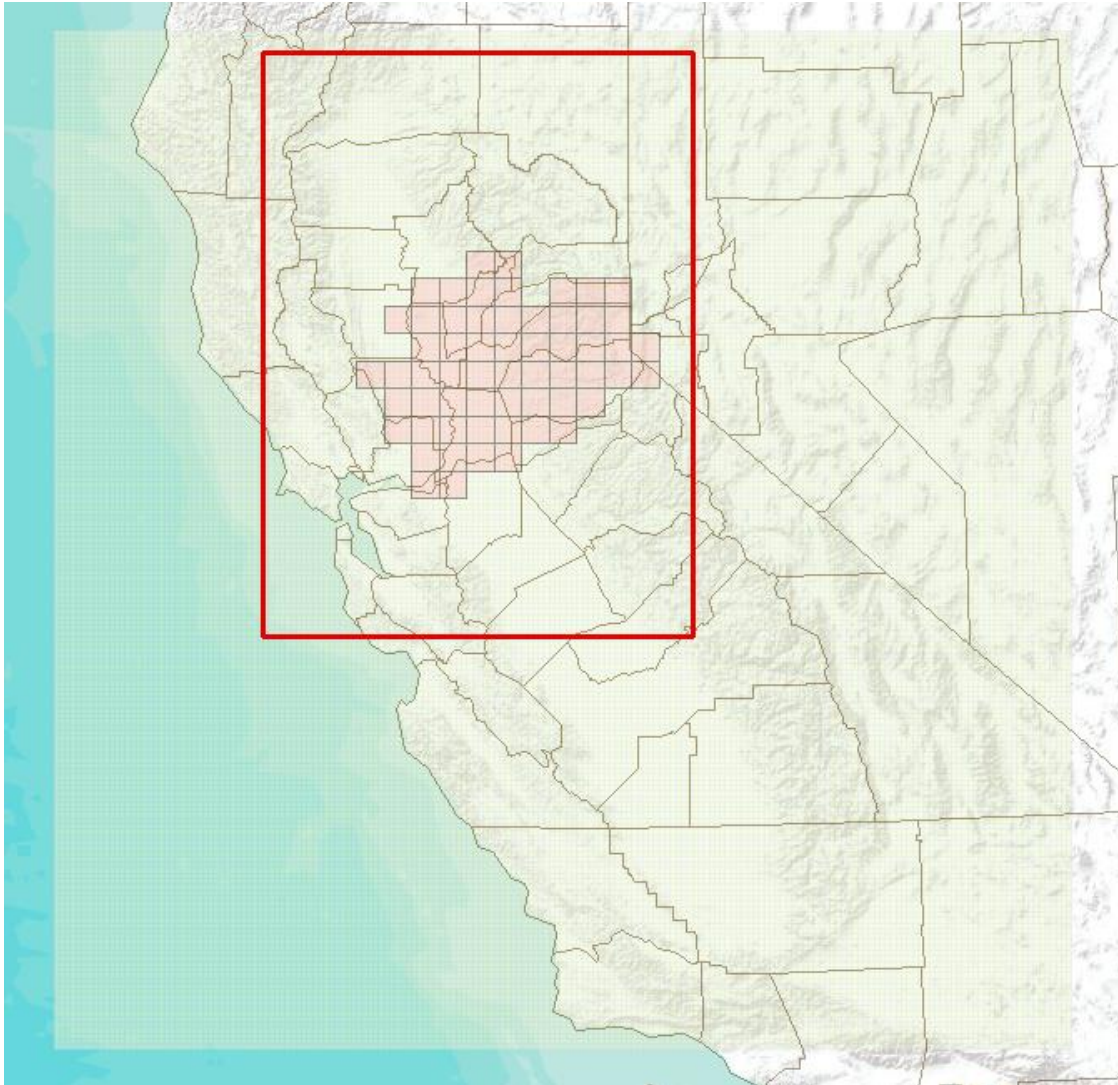
Figure B-2. Sac Metro Air District CAMx 4-km domain (red box) used in the screening analysis embedded in the 4-km CCOS domain (4-km grid cell hatched area covering northern California).
