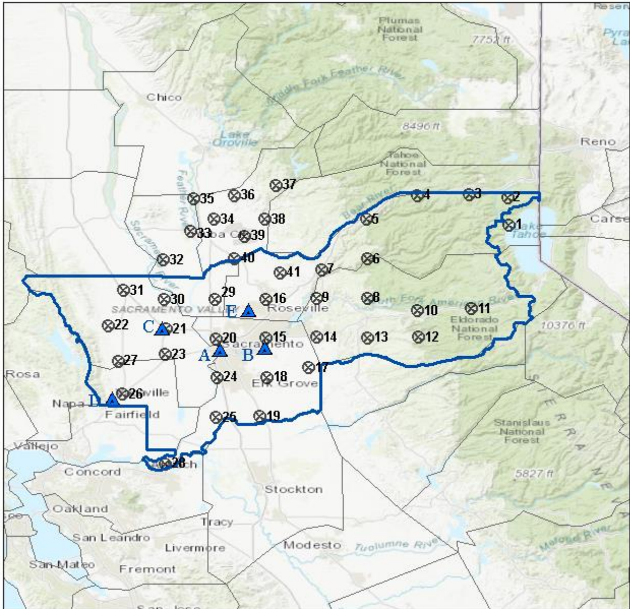
Figure C-1. Locations of five projects A-E used in the strategic area screening modeling, along with the 41 hypothetical Projects used in the minor project analysis and boundary of the SFNA.
