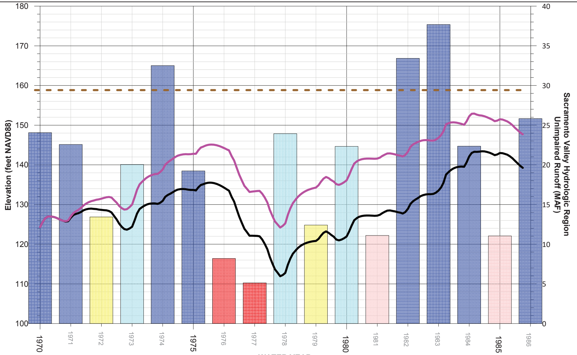
FIGURE 10-8B Simulated Groundwater Elevations Versus Time at the Orchards Southeast of Funks Creek Sites Reservoir Project EIR/EIS
