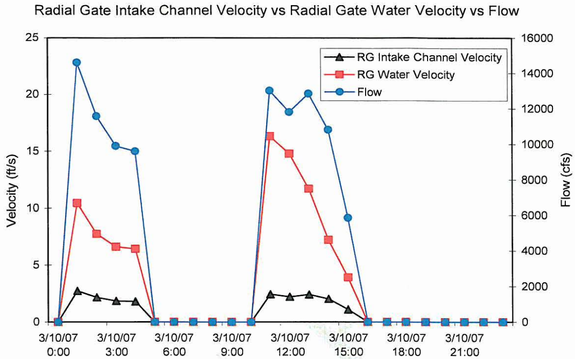
Figure 8. Flow (cfs) and velocity (ft/s) through the radial gates for a 24 hour period in 2007. The radial gates were open from 01:00 to 04:00 and from 11:00 to 15:00.
