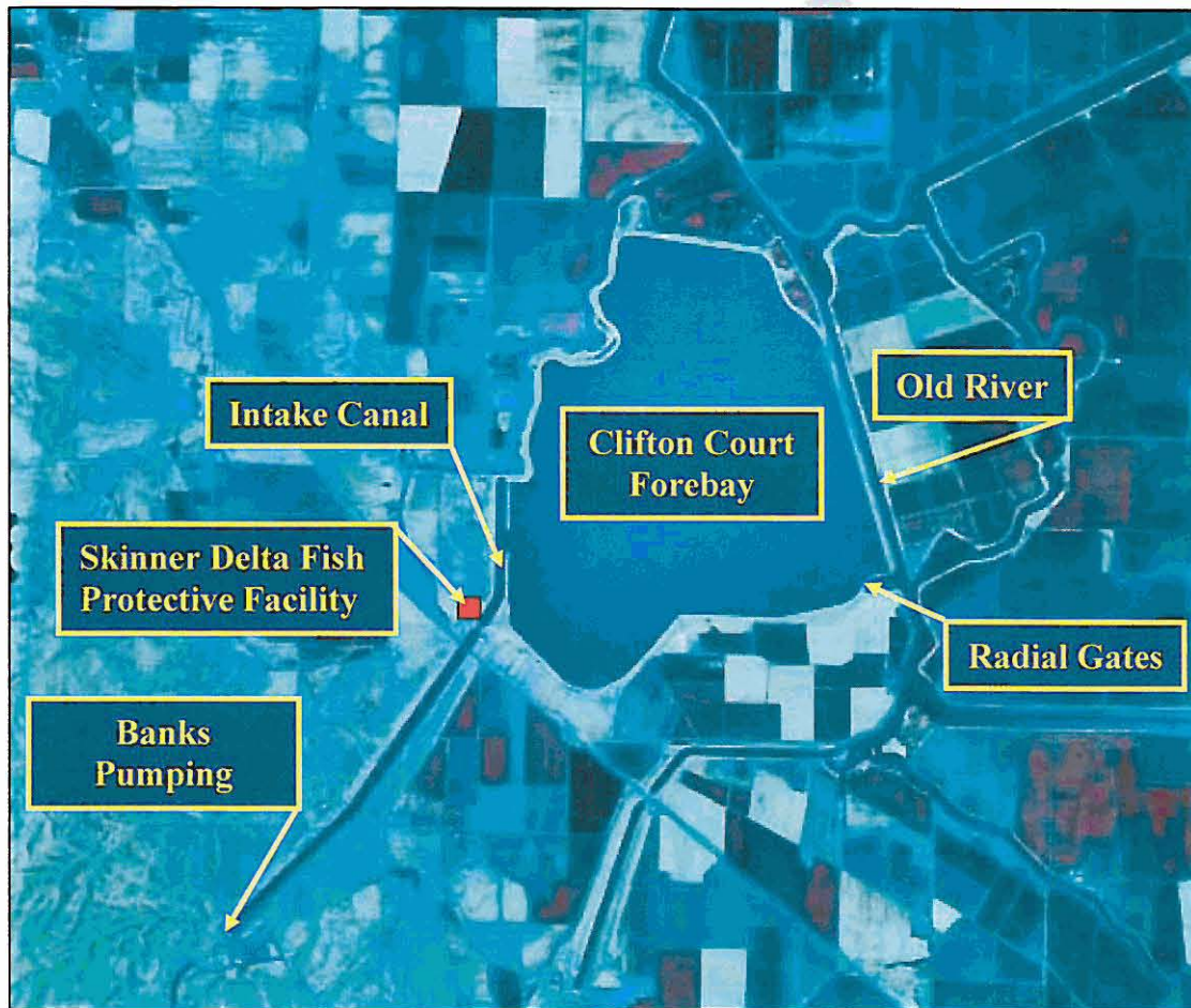
Figure 2. Aerial photograph of Clifton Court Forebay with the locations of Old River, radial gates, intake canal, Banks Pumping Plant, and the John E. Skinner Delta Fish Protective Facility. (National High Altitude Photography courtesy of the United States Geological Survey)
