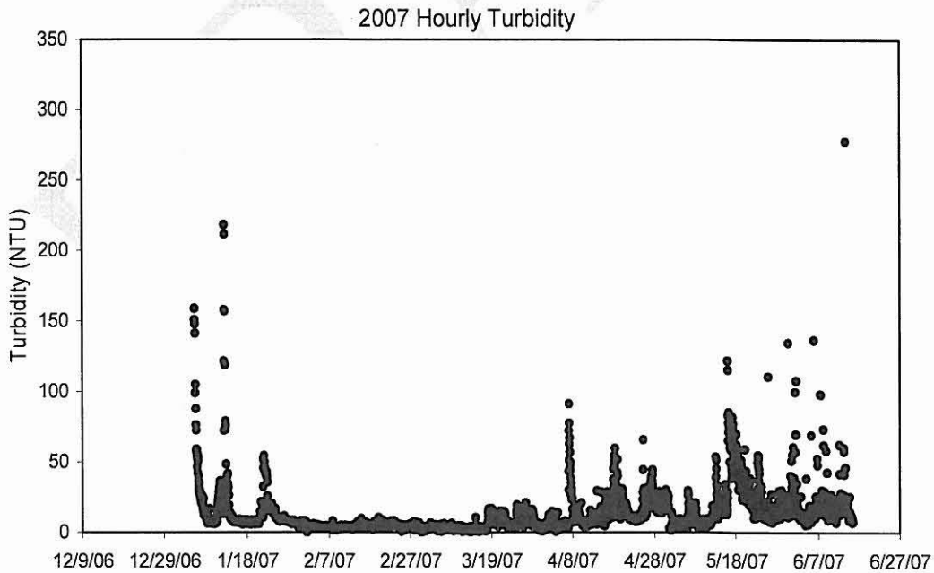
Figure 31. 2007 turbidity measured hourly via a HACH Hydrolab deployed at the SFPP trashboom.
