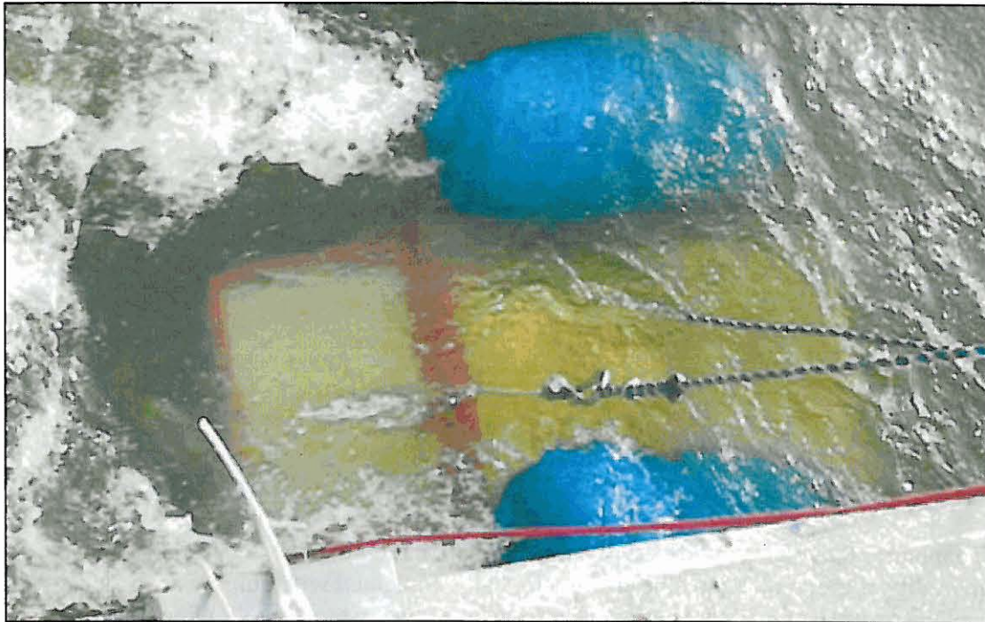
Figure 17. Release of tagged steelhead immediately upstream of the radial gates using the live-car. Two blue floats were attached to the live-car and used to float the live-car into position directly upstream of the radial gates.
