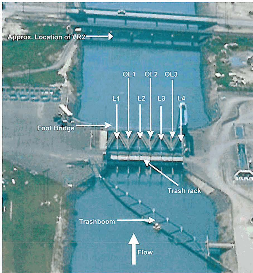
Figure 20. Acoustic tag range testing positions within the SFPF louvers. The acoustic tag (VEMCO, model V8SC) was lowered into the water at the trashboom, at the trash rack, inside the louver bays (L1, L2, L3, L4), outside the louver bays (OL1, OL2, OL3), and at the foot bridge.
