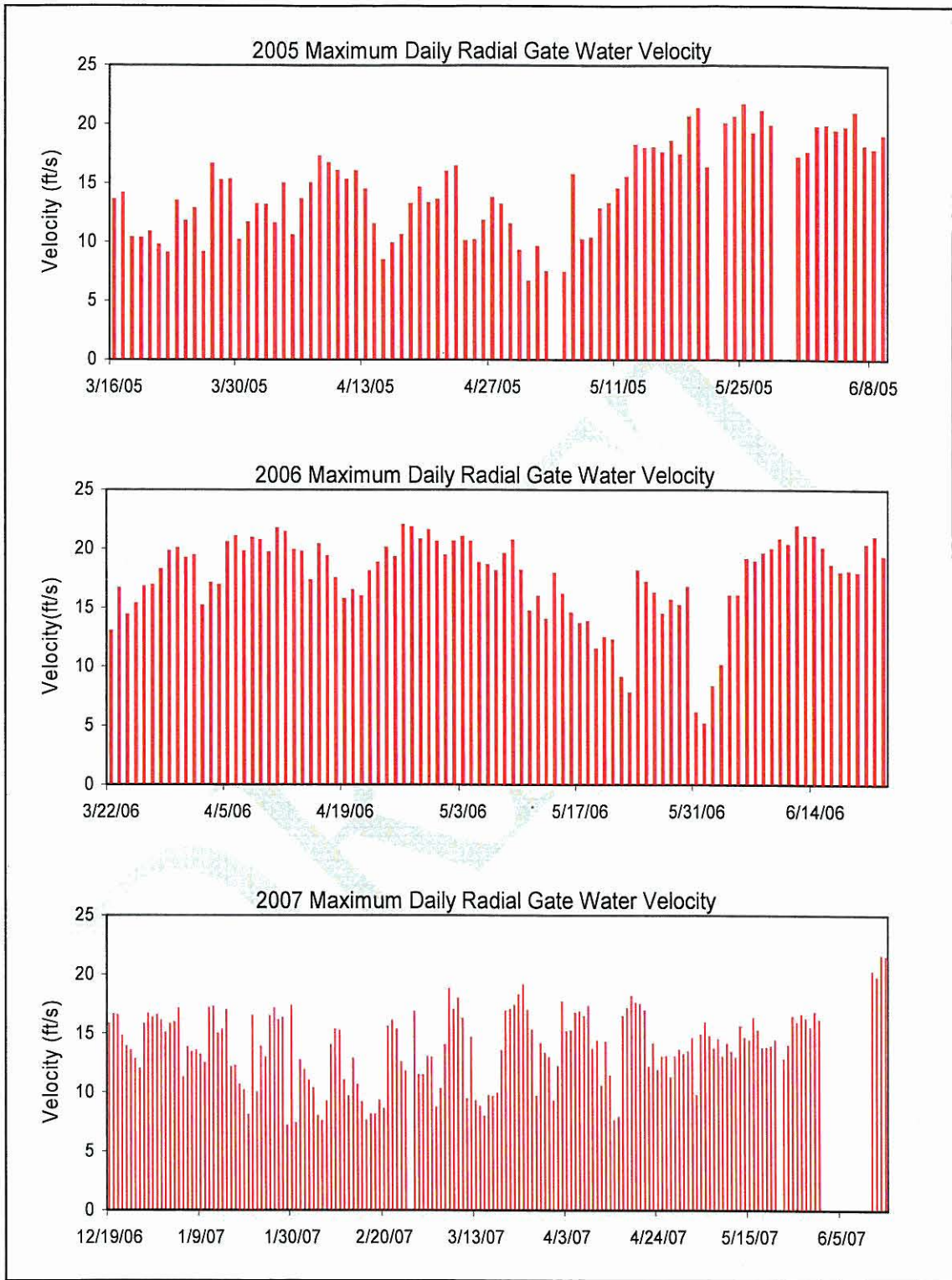
Figure 7. Estimated maximum daily water velocity (ft/s) at the radial gates during 2005 and 2006 pilot studies and the 2007 full-scale study.
