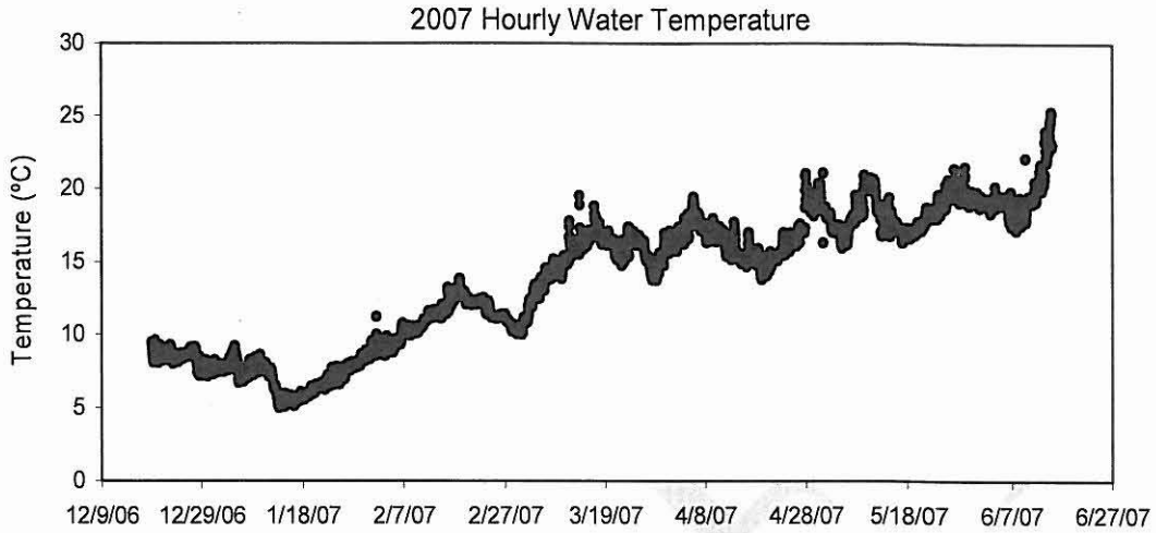
Figure 30. 2007 water temperatures measured hourly via a HACH Hydrolab at the SFPP trashboom and a HOBO temperature logger in the intake canal.
