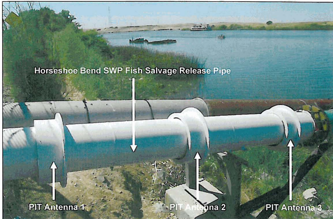
Figure 37. PIT antennas installed around the release pipe at the Horseshoe Bend, SFPF salvage release site.
