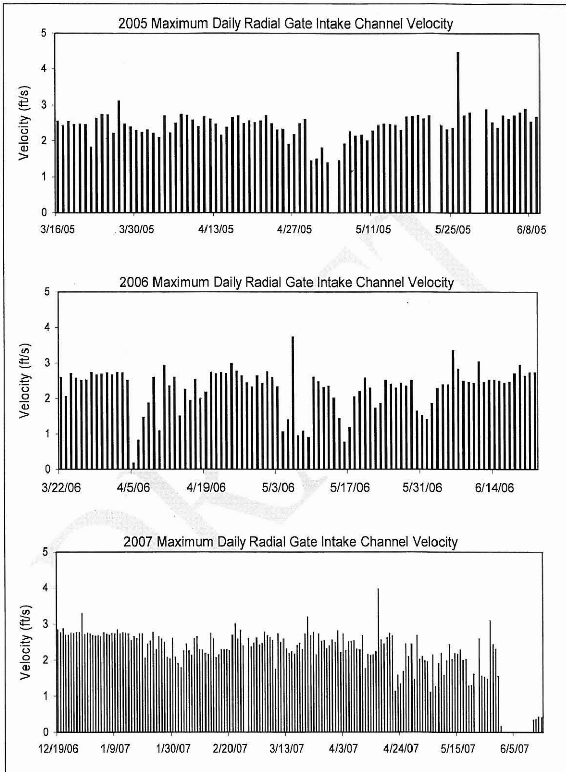
Figure 6. Calculated maximum daily intake channel velocities (ft/s) directly upstream of the radial gates during the 2005 and 2006 pilot studies and the 2007 full-scale study.
