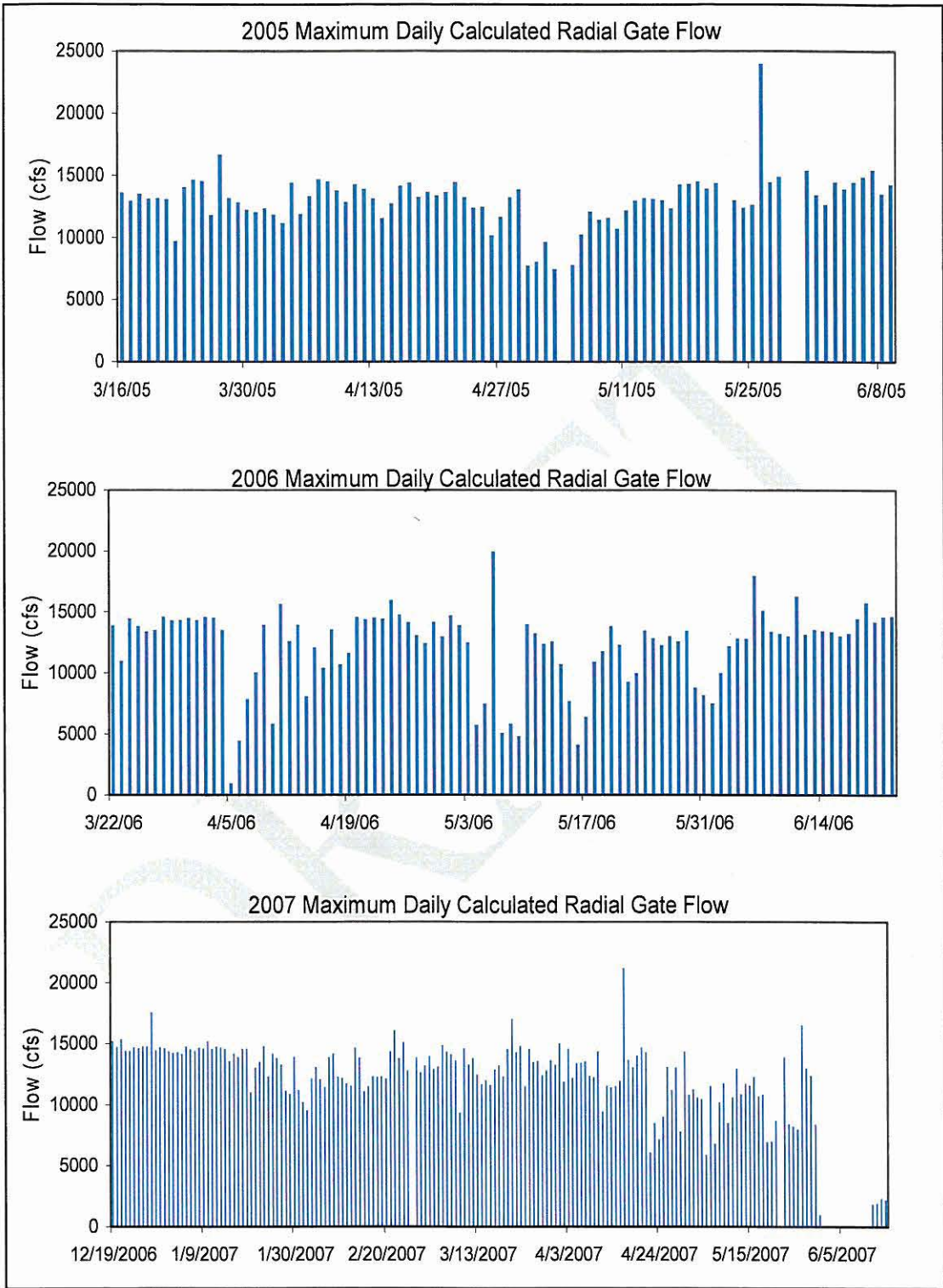
Figure 5. Calculated maximum daily flow (cfs) at the radial gates during the 2005 and 2006 pilot studies and the 2007 full-scale study.
