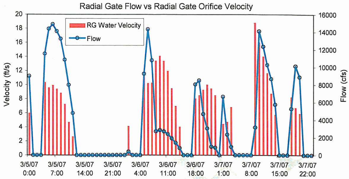
Figure 10. Radial gate flow (cfs) versus radial gate water velocity (ft/s) for a 36 hour period during 2007.
