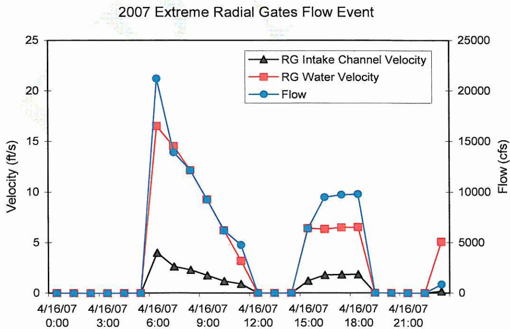
Figure 9. Radial gate extreme flow event April 16, 2007.
