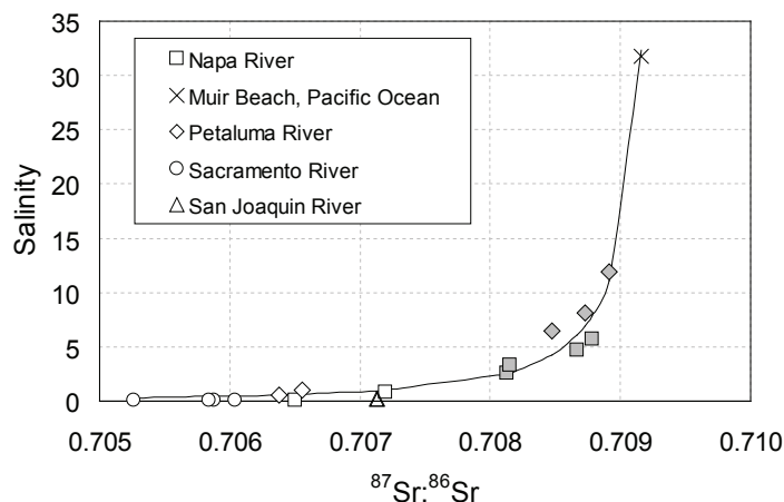
Figure 2 Plot of ^{87}\text{Sr}:^{86}\text{Sr} versus salinity for water samples. The curve is defined by y = 0.000013/(1+2.82*x+1.98*x^2) ( r^2 = 0.98 , P < 0.001 ). We characterized the open symbols as a freshwater group and the filled symbols as a brackish group.
