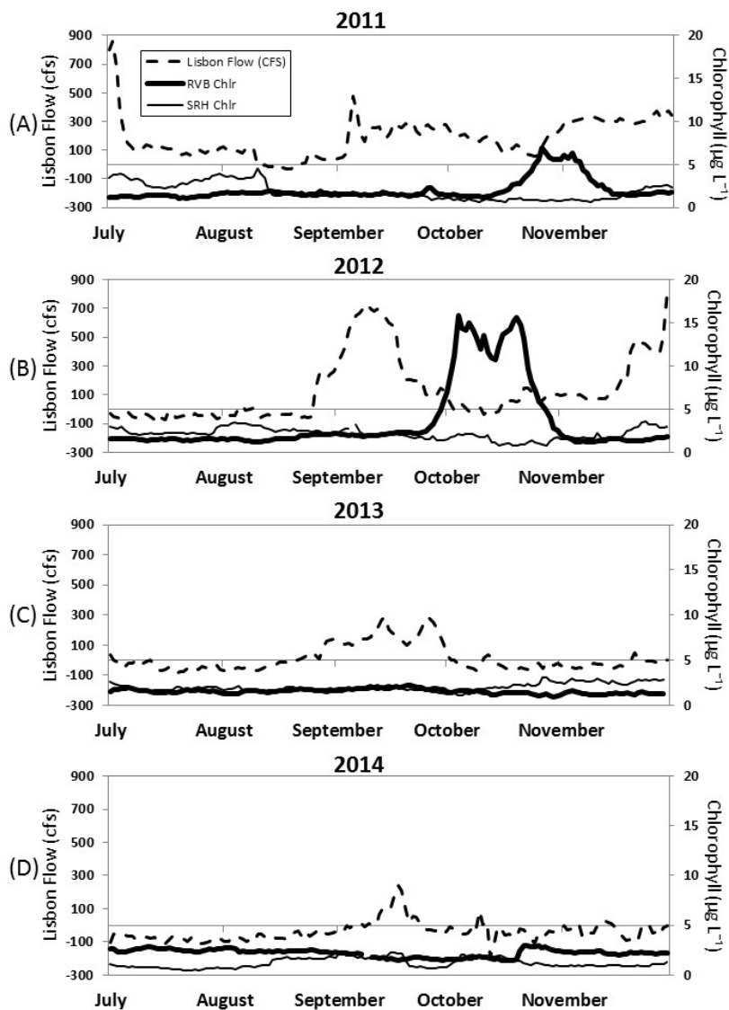
Figure 4 2011–2014 Daily average continuous chlorophyll ( \mu\text{g L}^{-1} ) from Sacramento River at Hood (SRH), Sacramento River at Rio Vista Bridge (RVB) and Lisbon (LIS) mean daily flow (cfs)
