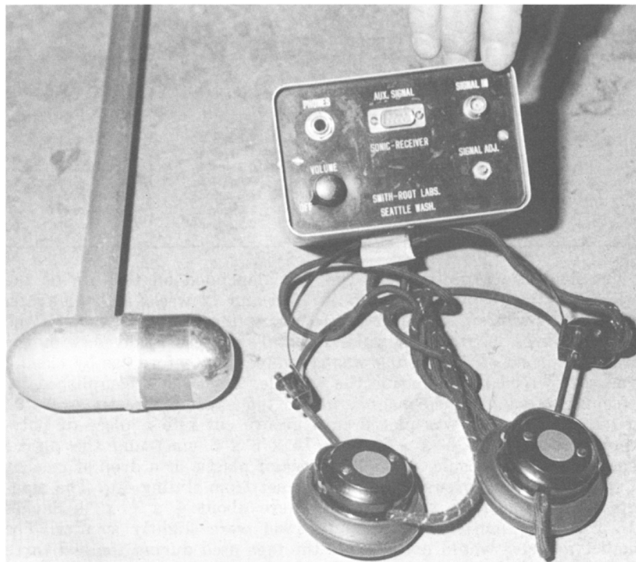
FIGURE 8. Portable probe (or hydrophone) and receiver for tracking sonic tags. Photograph by John A. Shaver.
