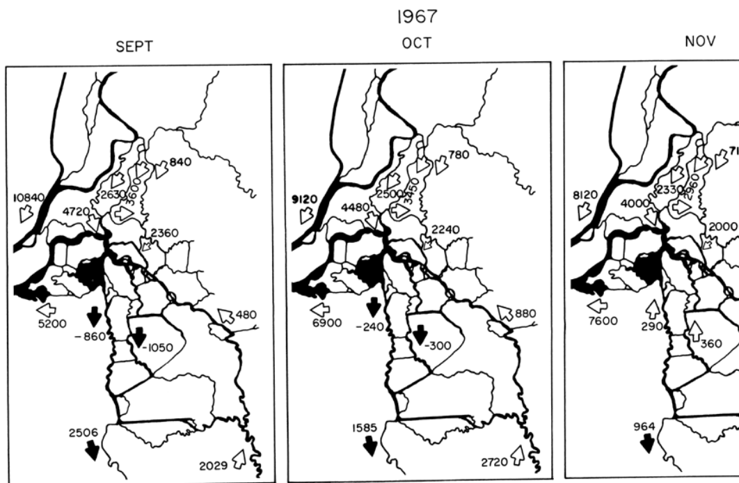
FIGURE 6. Rate (cfs) and direction of mean monthly net flows in the Sacramento-San Joaquin Delta. Fall of 1967. Open arrows indicate direction, solid arrows indicate reversed flows.
