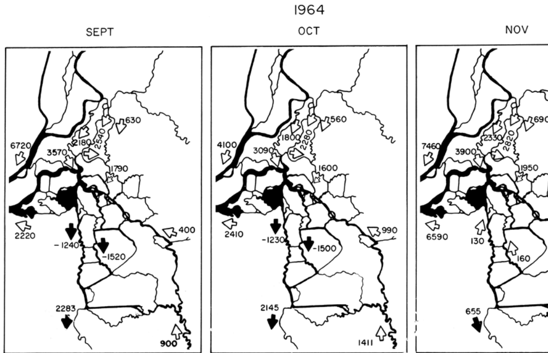
FIGURE 3. Rate (cfs) and direction of mean monthly net flows in the Sacramento-San Joaquin Delta, Fall of 1964. Open arrows indicate direction, solid arrows indicate reversed flows.
