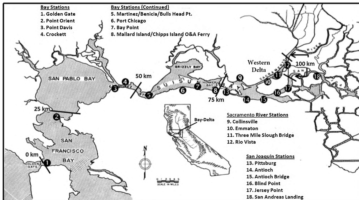
Fig. 1. Key salinity stations are identified in Suisun Bay and the western Delta; salinity data from these and other locations were used to develop a long-term record of X2, the position of two parts per thousand bottom salinity in the estuary; the X2 position is reported as the distance in kilometers from Golden Gate along the axis of the estuary, following the original definition of the term (Jassby et al. 1995); the Sacramento and San Joaquin River branches are identified on the map
