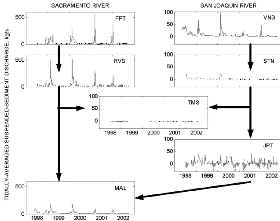
Figure 11. Tidally averaged suspended sediment flux. Arrows indicate downstream/down estuary flow paths for the (left) Sacramento and (right) San Joaquin rivers. The vertical scale for the Sacramento River flow path is larger than that for the San Joaquin River flow path and Three Mile Slough (TMS).
