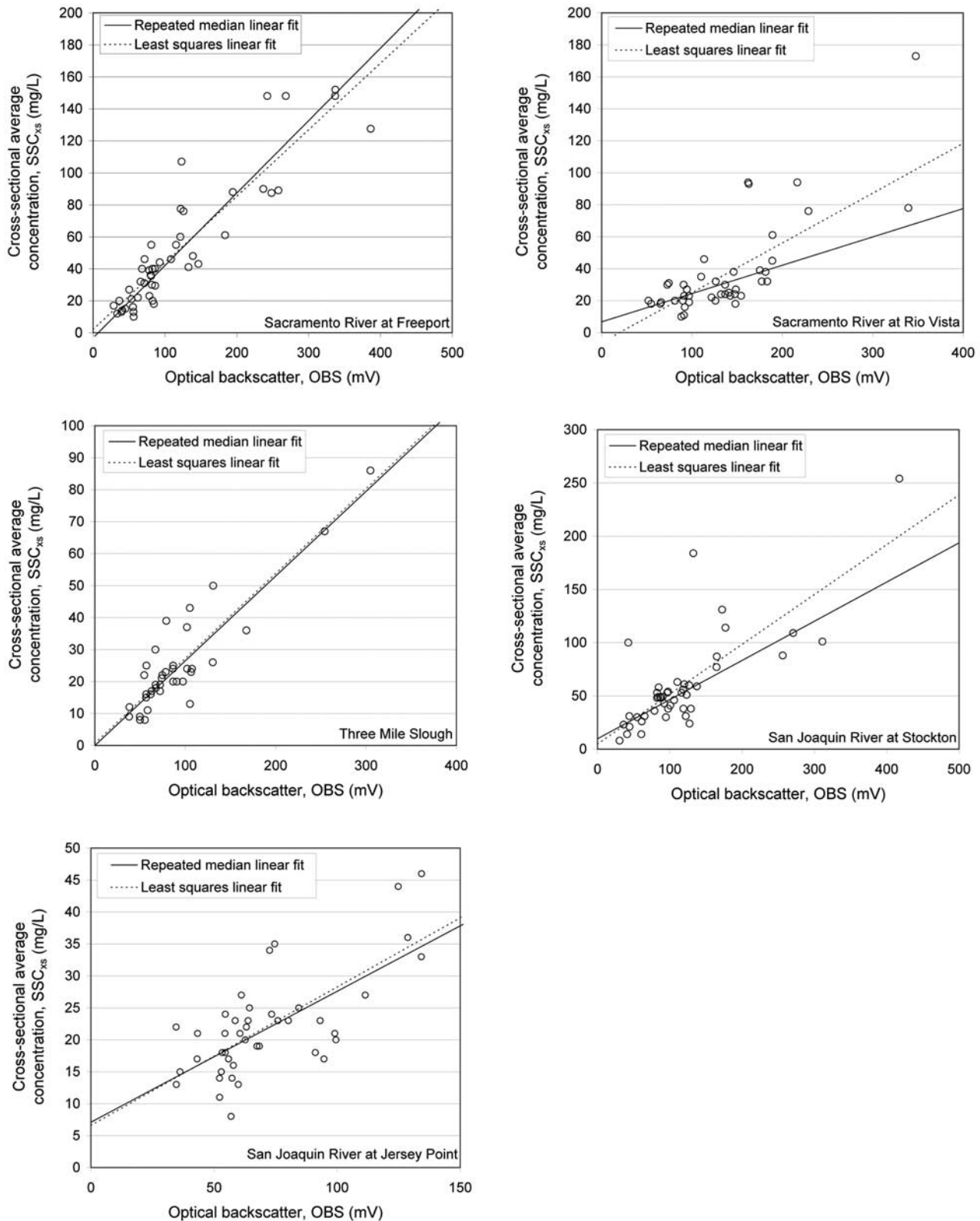
Figure 4. Relation between cross-sectional average concentration, SSC_{xs} , and near-bank optical backscatter, OBS, for the five delta sites.
