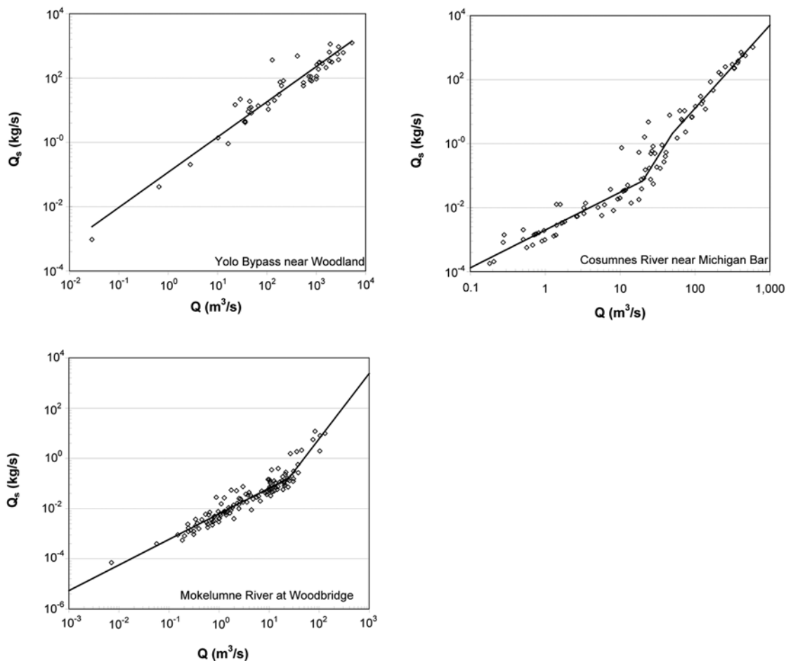
Figure 8. Suspended-sediment rating curves for the Yolo Bypass near Woodland, Cosumnes River near Michigan Bar, and Mokelumne River at Woodbridge.
