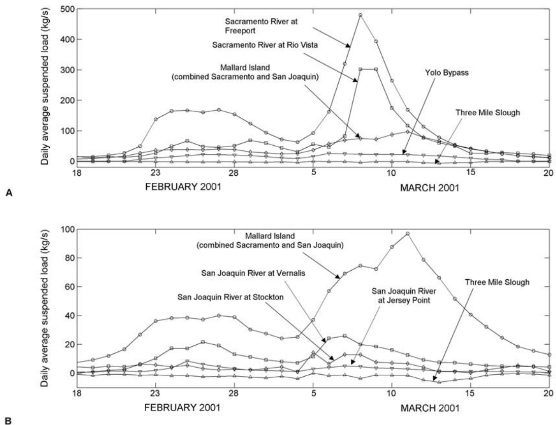
Figure 10. Movement of the main sediment pulse of water year 2001 down the (a) Sacramento and (b) San Joaquin rivers. Three Mile Slough flux is positive from the San Joaquin River to the Sacramento River.
