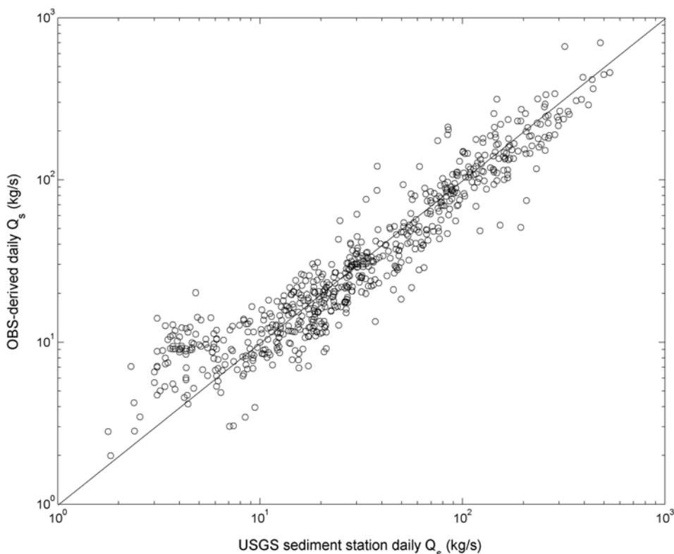
Figure 6. Comparison of OBS-derived and USGS sediment station daily suspended-sediment flux ( Q_s ) for the Sacramento River at Freeport for water years 1999–2002.
