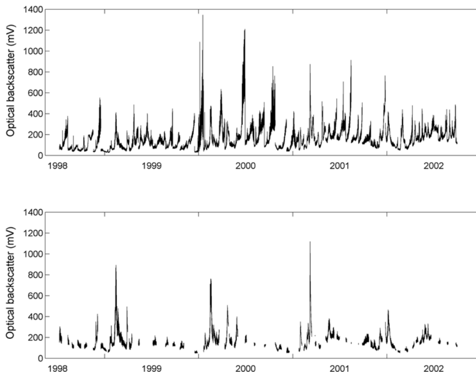
Figure 2. (top) Raw and (bottom) edited optical backscatter records for the Sacramento River at Rio Vista.
