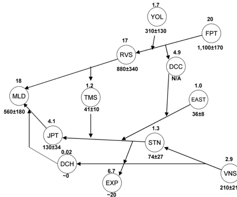
Figure 9. Average annual delta water and sediment budgets based on water years 1999–2002, except for TMS, which is based on water years 2001 and 2002 only. For each location the top number is annual water flux in billion m 3 , and the bottom number is annual suspended-sediment flux and the estimated error in thousand metric tons.
