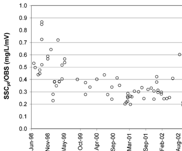
Figure 3. Ratio of point concentration to optical backscatter for Three Mile Slough, illustrating the drift in sensor voltage output with time.
