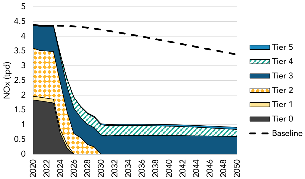
Figure 48 - South Coast NOx Emissions from CHC: MSS Scenario
