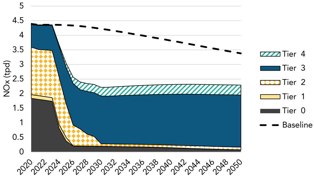
Figure 47 - South Coast NOx Emissions from CHC: Regulatory Proposal
