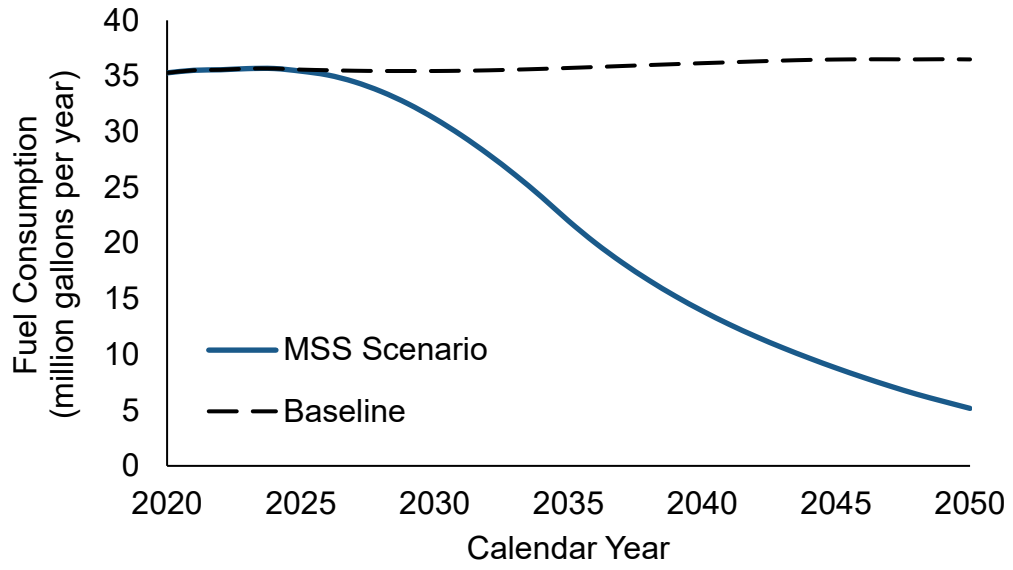
Figure 20 - Statewide Fuel Consumption for On-Road Motorcycles – MSS Scenario
