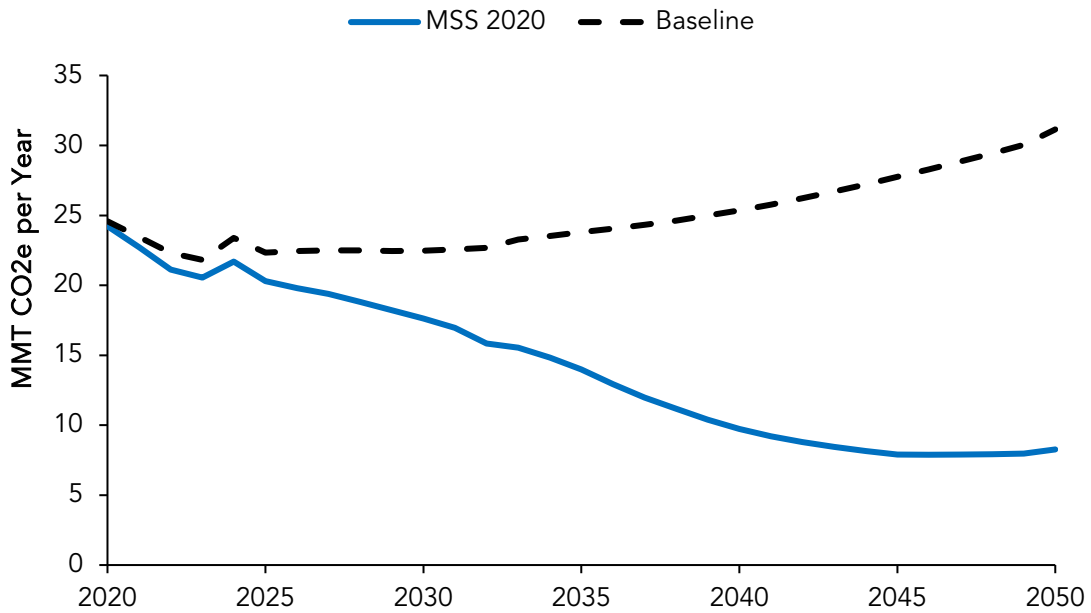
Figure 27 - Statewide Well-To-Wheel GHG Emissions from Heavy-Duty Vehicles
