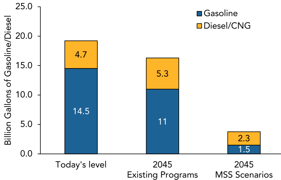
Figure 6 - Impact of the 2020 Strategy Scenario on Mobile Source Liquid Fuel Consumption in 2045
