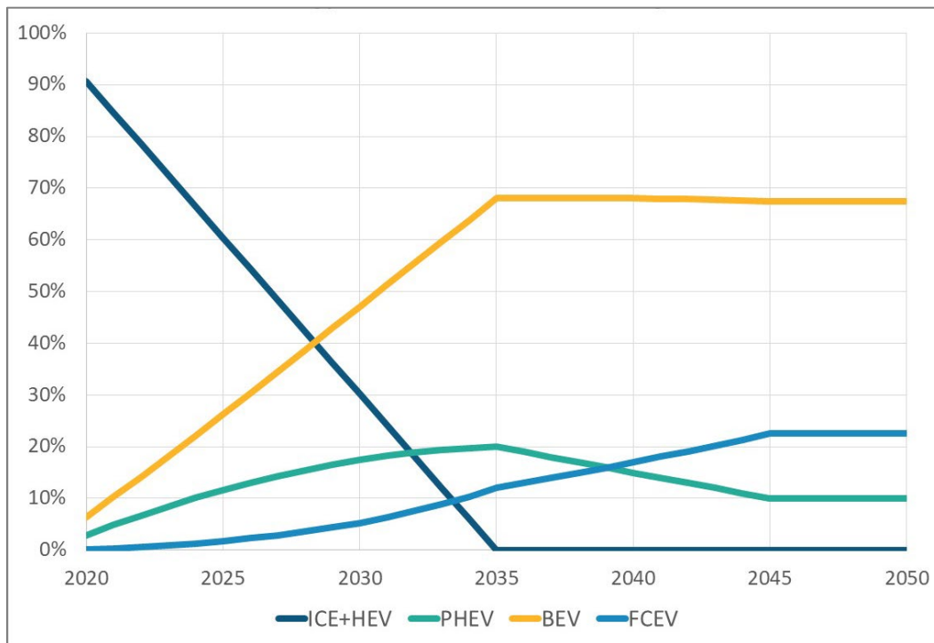
Figure 13 – Light-Duty Vehicle Sales Fractions by Technology Type
