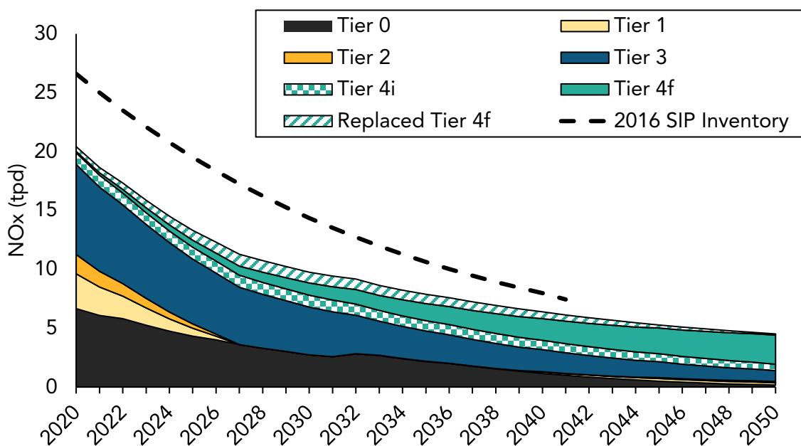
Figure 46 - San Joaquin Valley NOx Emissions from Farm Tractors
