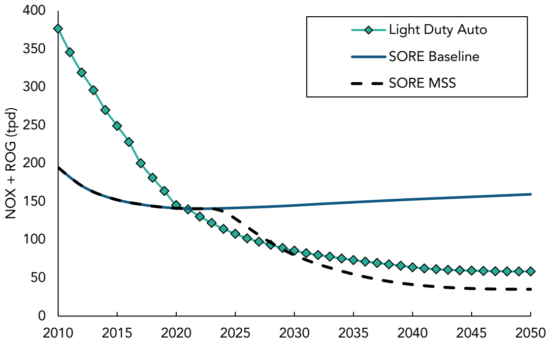
Figure 39 - Statewide Smog-Forming Emission Projections from SORE
