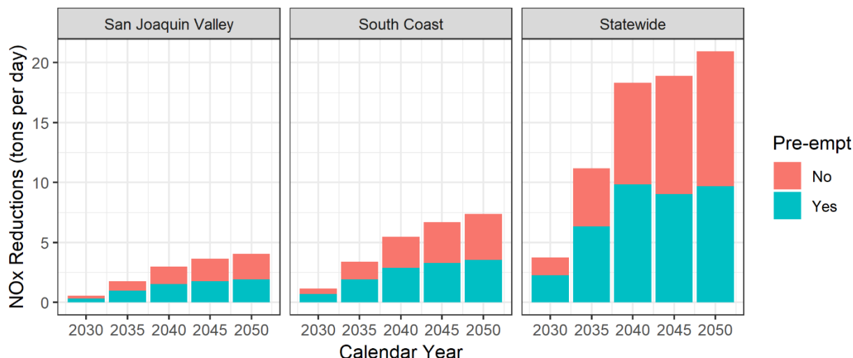
Figure 51 - Off-Road NOx Emissions Benefits from Tier 5
