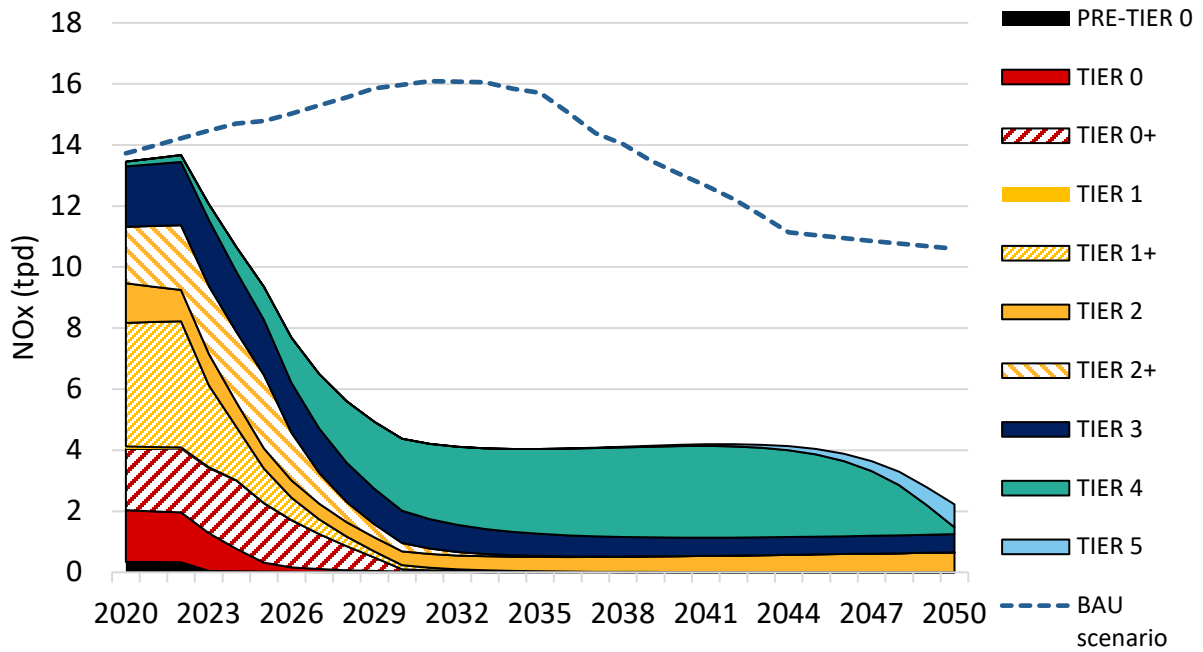
Figure 30 - South Coast Air Basin NOx Emissions from Locomotives: MSS Scenario
