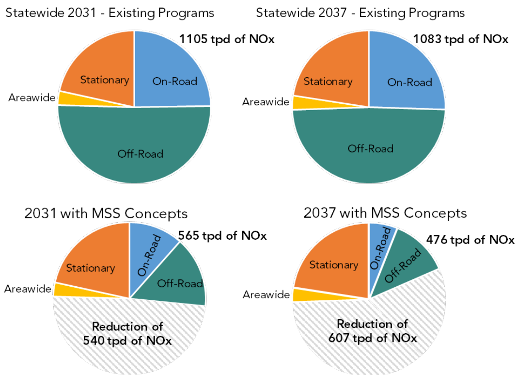
Figure 5 - Impact of the 2020 Strategy Scenario on Statewide NOx Emissions in 2031 and 2037
