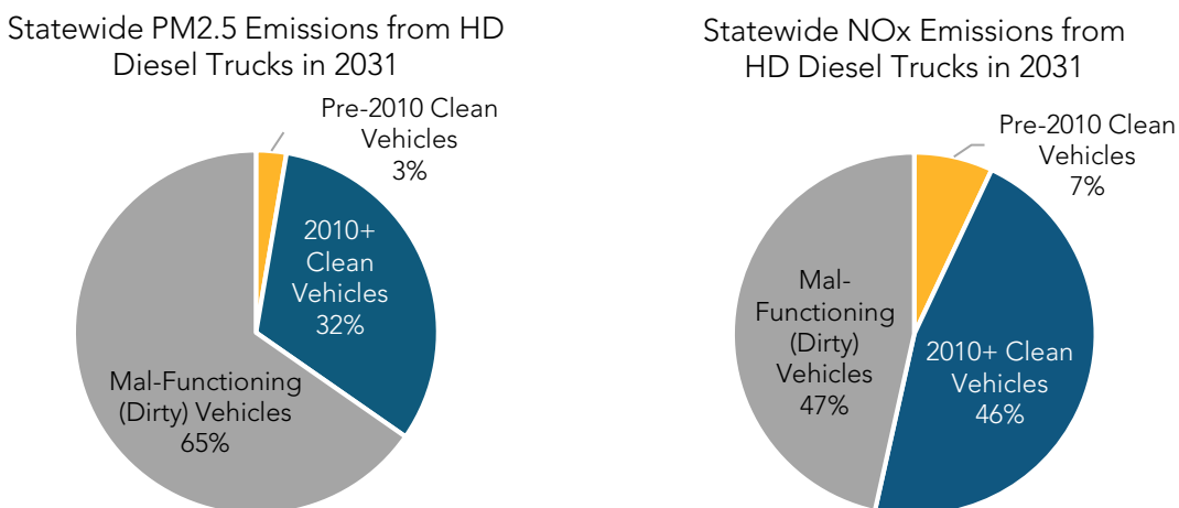
Figure 4 – NOx and PM2.5 Emission Contributions from Malfunctioning Heavy-Duty Diesel Trucks in California
