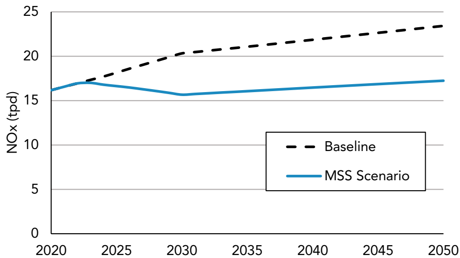
Figure 36 - South Coast NOx Emissions from Aircraft: MSS Scenario
