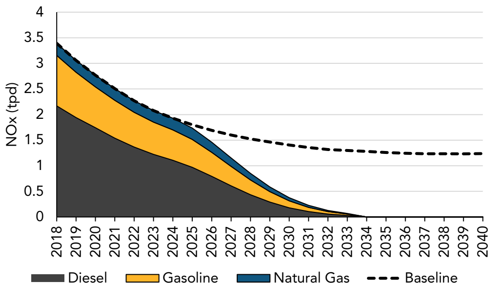
Figure 40 - Statewide NOx Emissions from GSE: MSS Scenario
