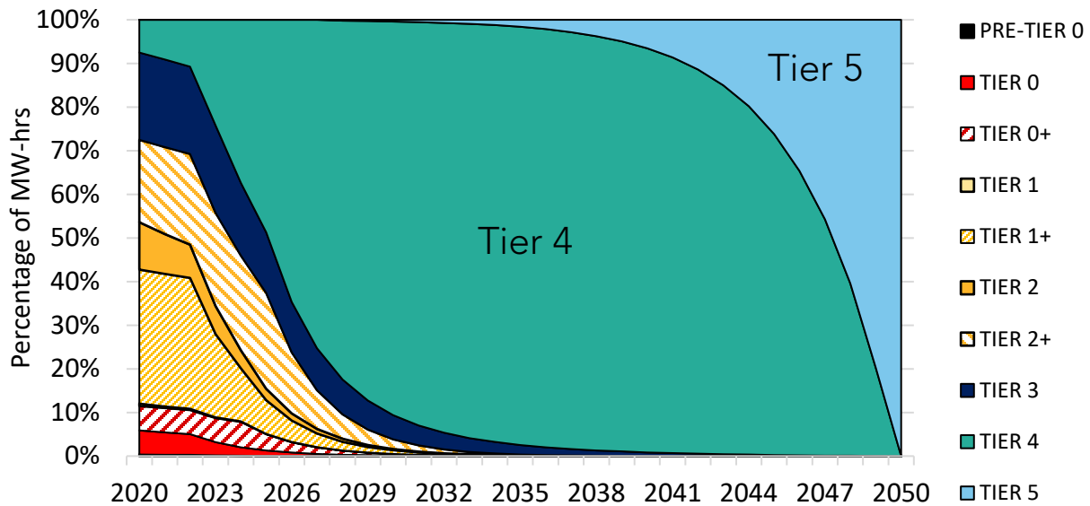
Figure 31 - South Coast Air Basin Locomotive Energy Use: MSS Scenario
