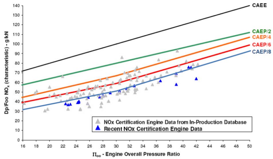
Figure 33 - Comparison of CAEP NOx standards and engine NOx emissions 198
