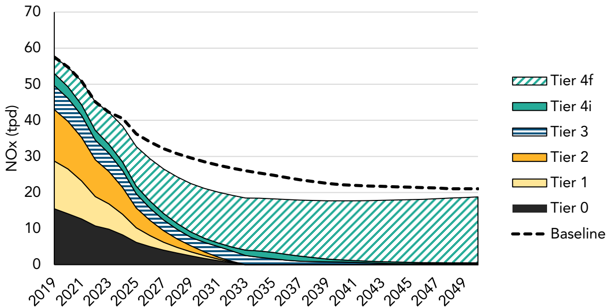
Figure 45 - Statewide NOx Emissions from In-Use Off-Road: MSS Scenario
