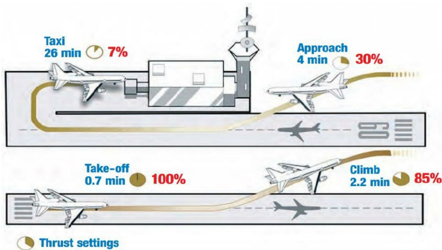
Figure 35- Duration and Thrust Settings within each Segment of the LTO Cycle
