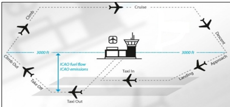
Figure 35- Duration and Thrust Settings within each Segment of the LTO Cycle
