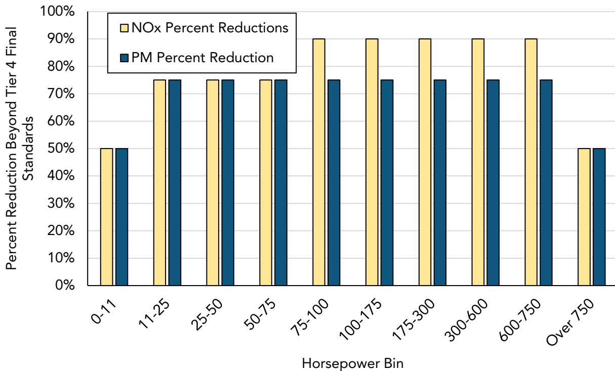
Figure 50 - Potential NOx and PM Emission Standard Reductions from Tier V Standards
