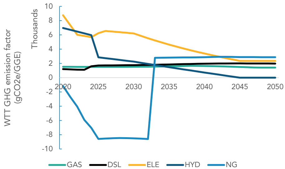
Figure 55 - WTT GHG EFs by Fuel Type 248
