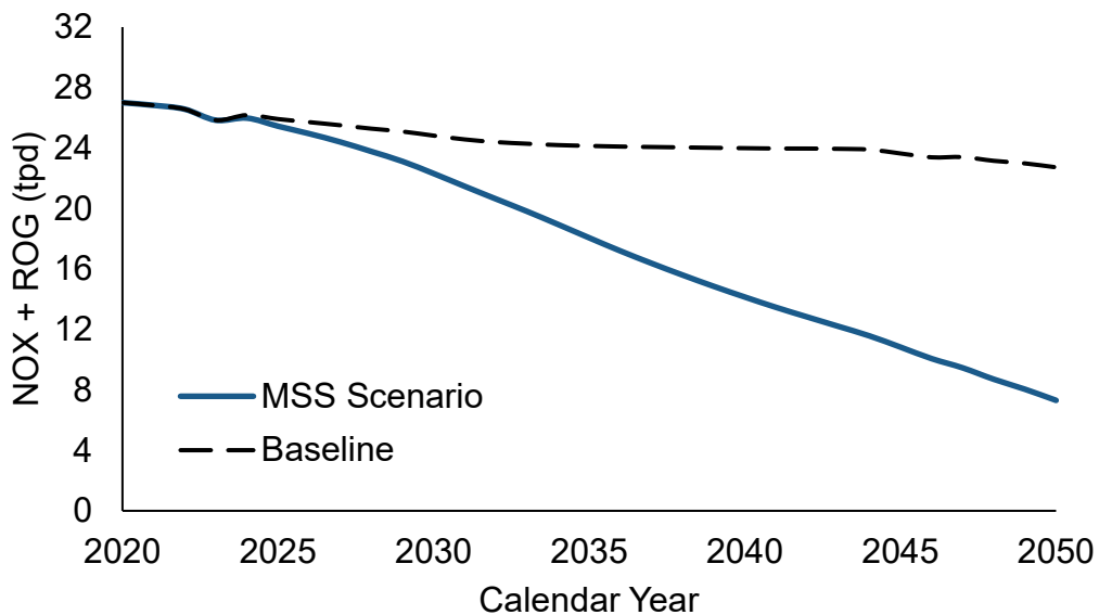
Figure 19 - Statewide Smog-Forming Projections for On-Road Motorcycles – MSS Scenario
