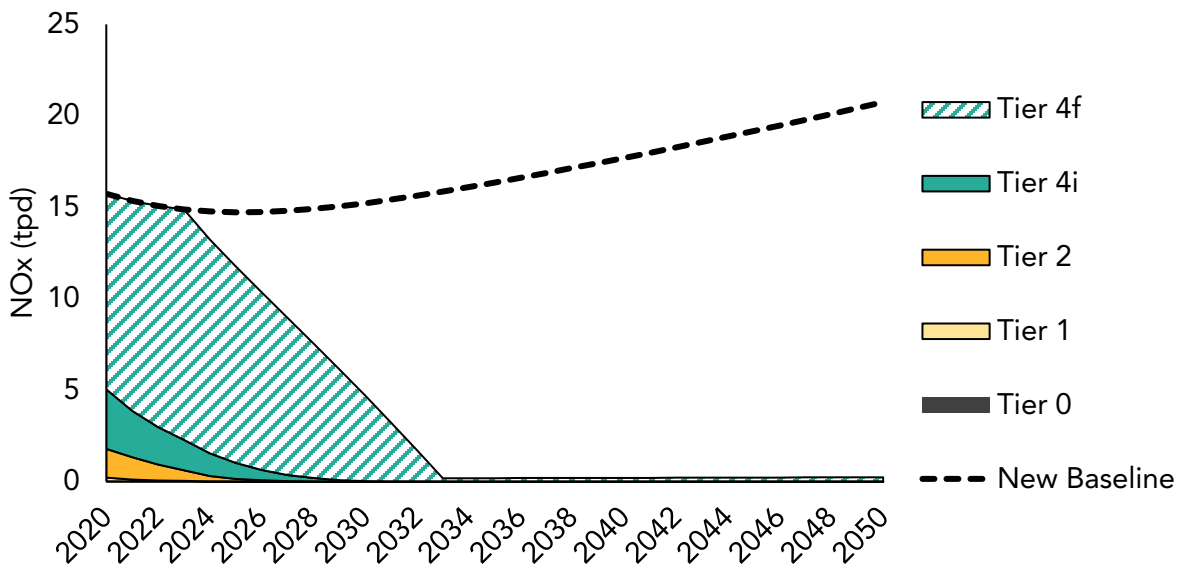
Figure 42 - Statewide NOx Emissions from TRU: MSS Scenario
