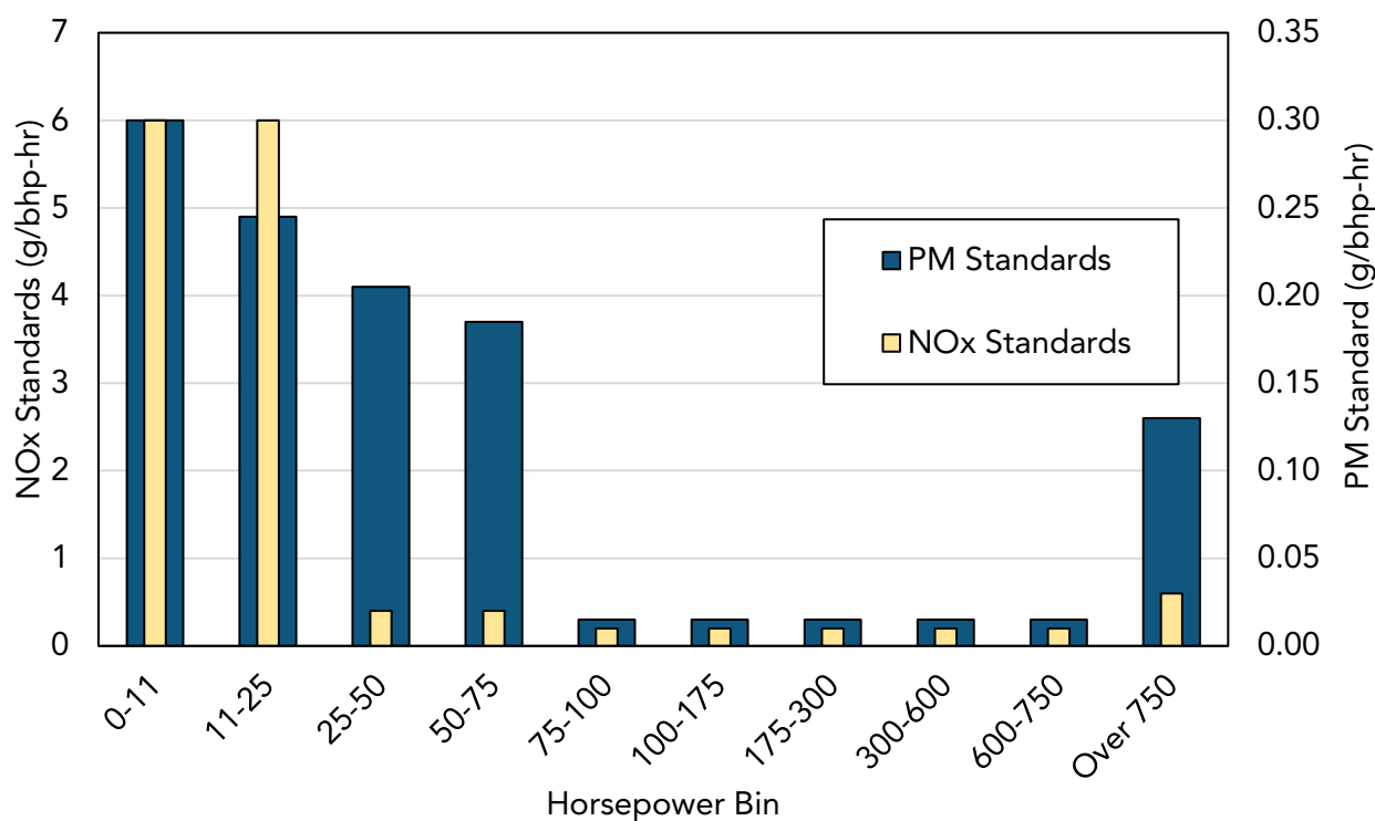
Figure 49 - Tier 4 Final Off-Road Diesel Standards for NOx and PM 213
