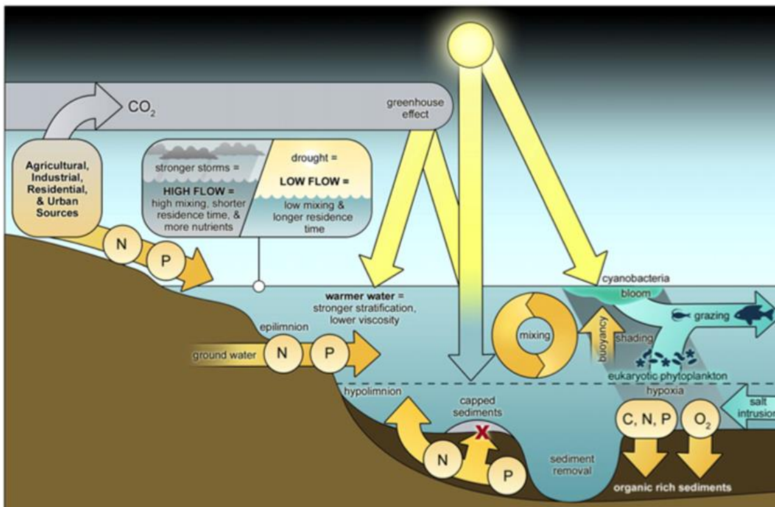
Figure 3.1. Conceptual model of factors affecting cyanobacteria blooms including warmer water, drought and decreased flow, decreased mixing, increased residence time, and increased N and P inputs from agricultural, industrial and urban sources. From Paerl et al. 2011.
