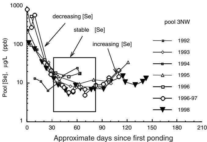
Figure 37.2 Typical ephemeral-pool-selenium concentration pattern following initial ponding, site 3NW.
