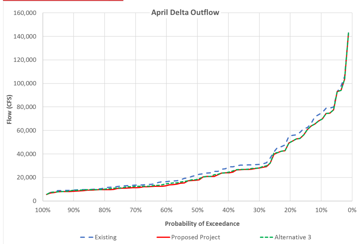
Figure 11: Probability of exceedance of Delta outflow in April
