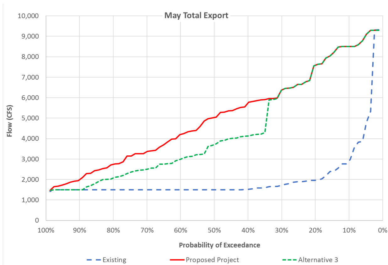
Figure 16: Probability of exceedance of total exports in May
