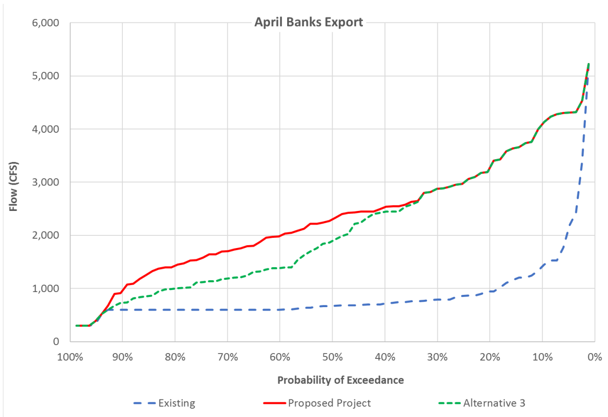
Figure 19: Probability of exceedance of Banks export in April
