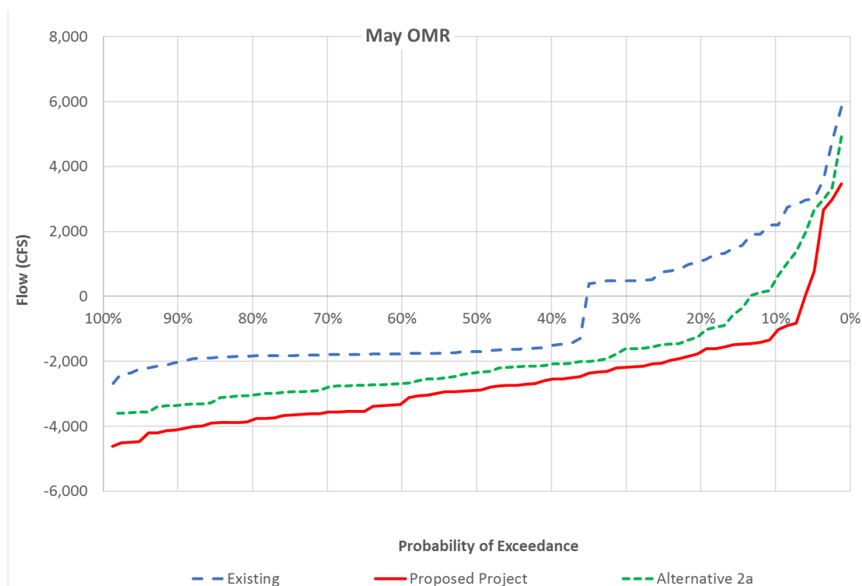
Figure 4: Probability of exceedance of OMR flow in May
