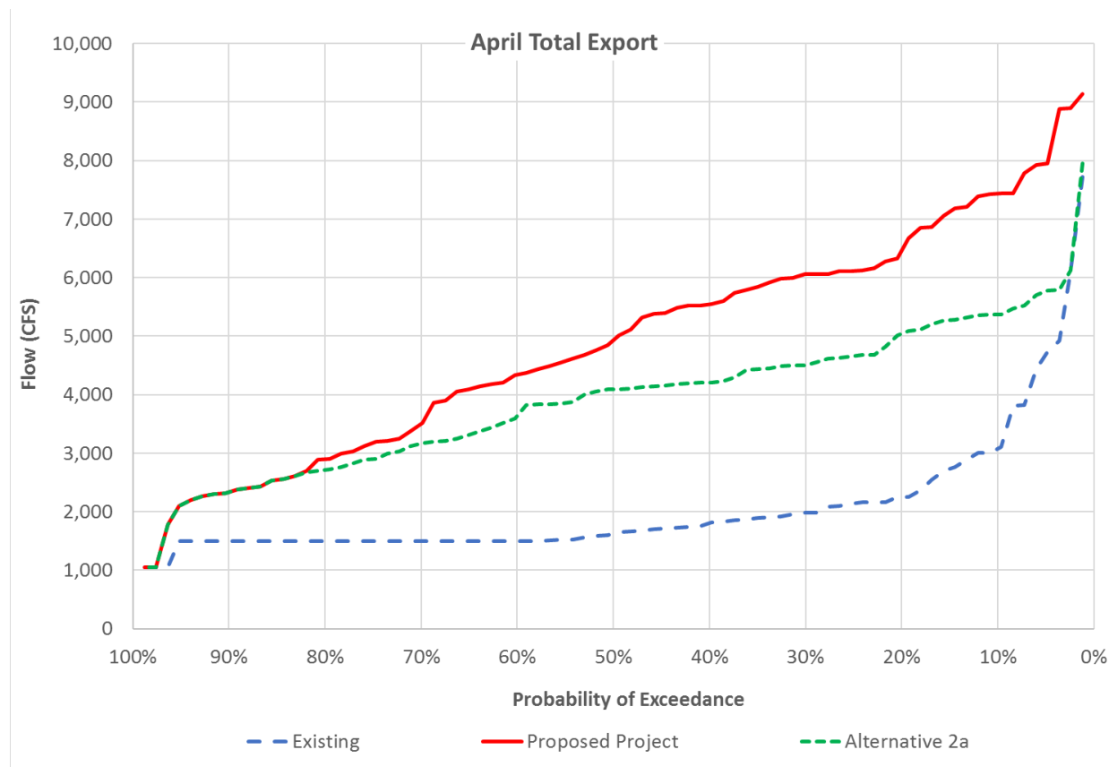
Figure 4: Probability of exceedance of total exports in April
