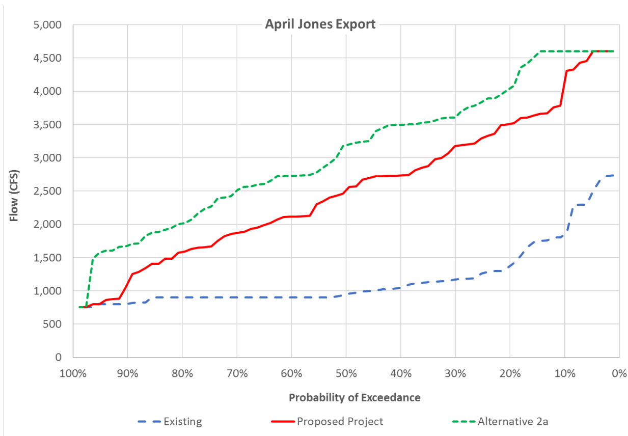
Figure 6: Probability of exceedance of Jones export in April
