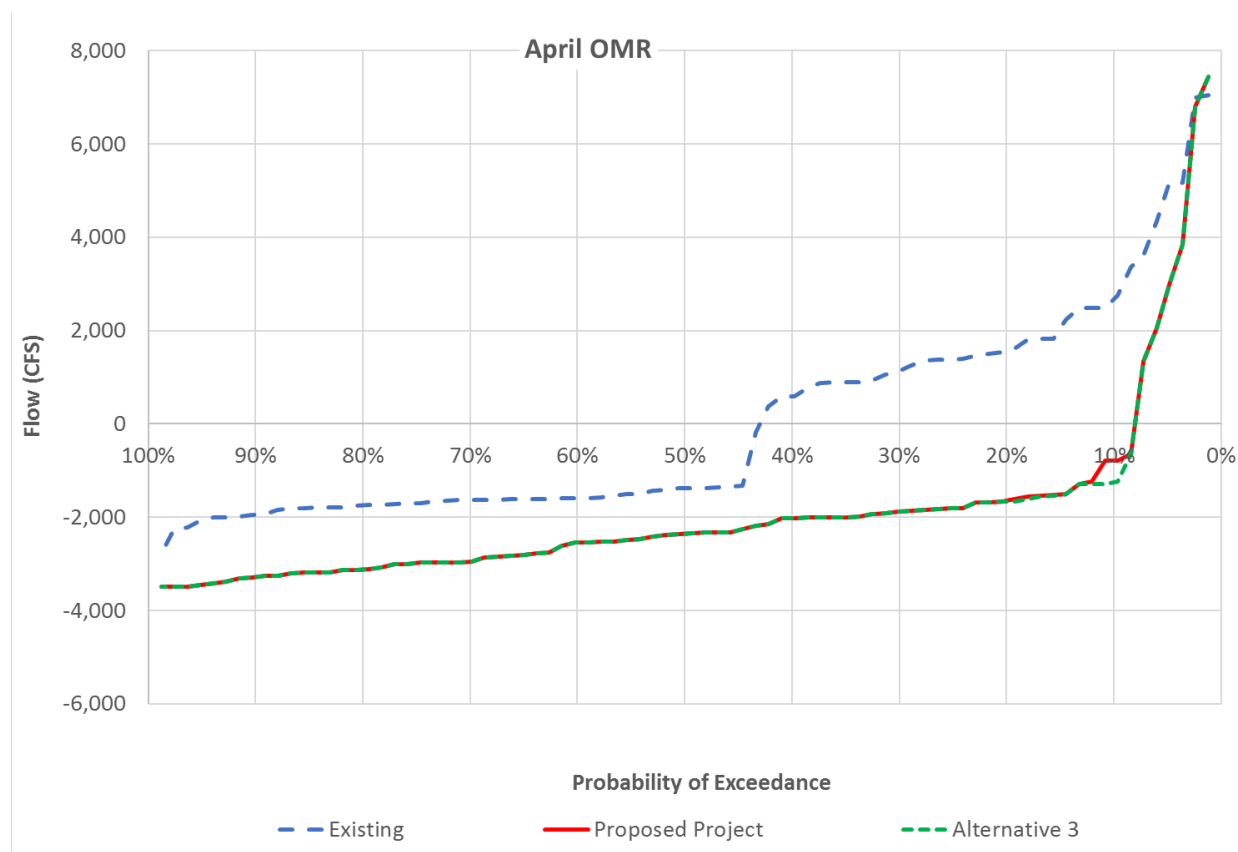
Figure 13: Probability of exceedance of OMR flow in April
