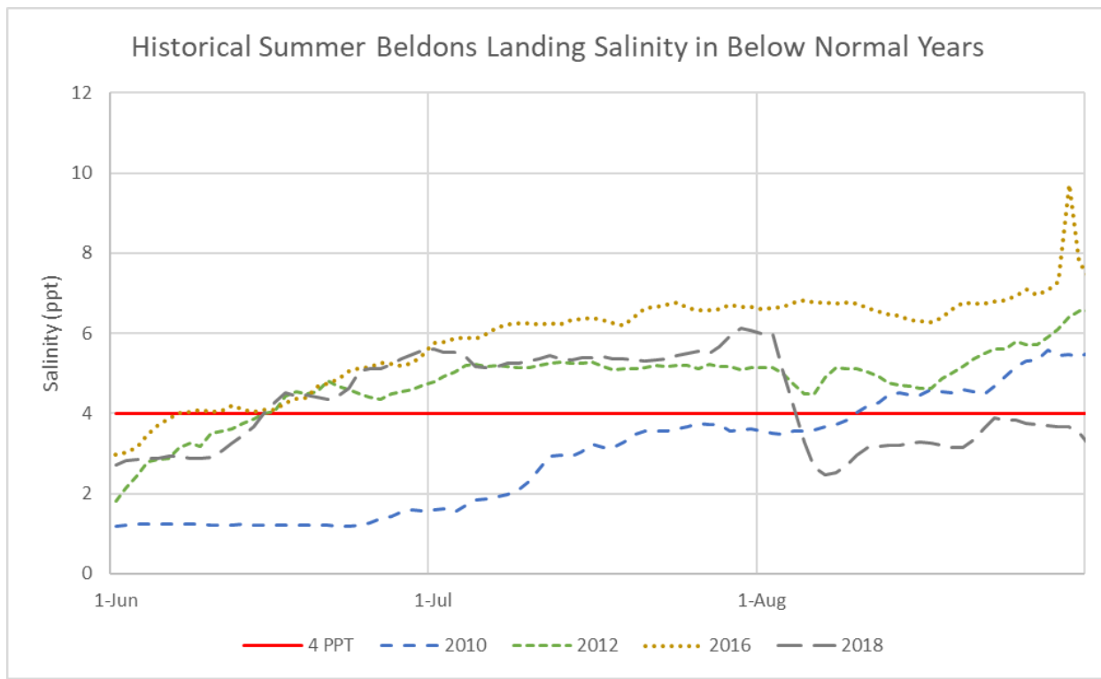
Figure 13. Historical daily average salinity at Beldons Landing in parts per thousand (ppt) in below normal years 2010, 2012, 2016, and 2018
