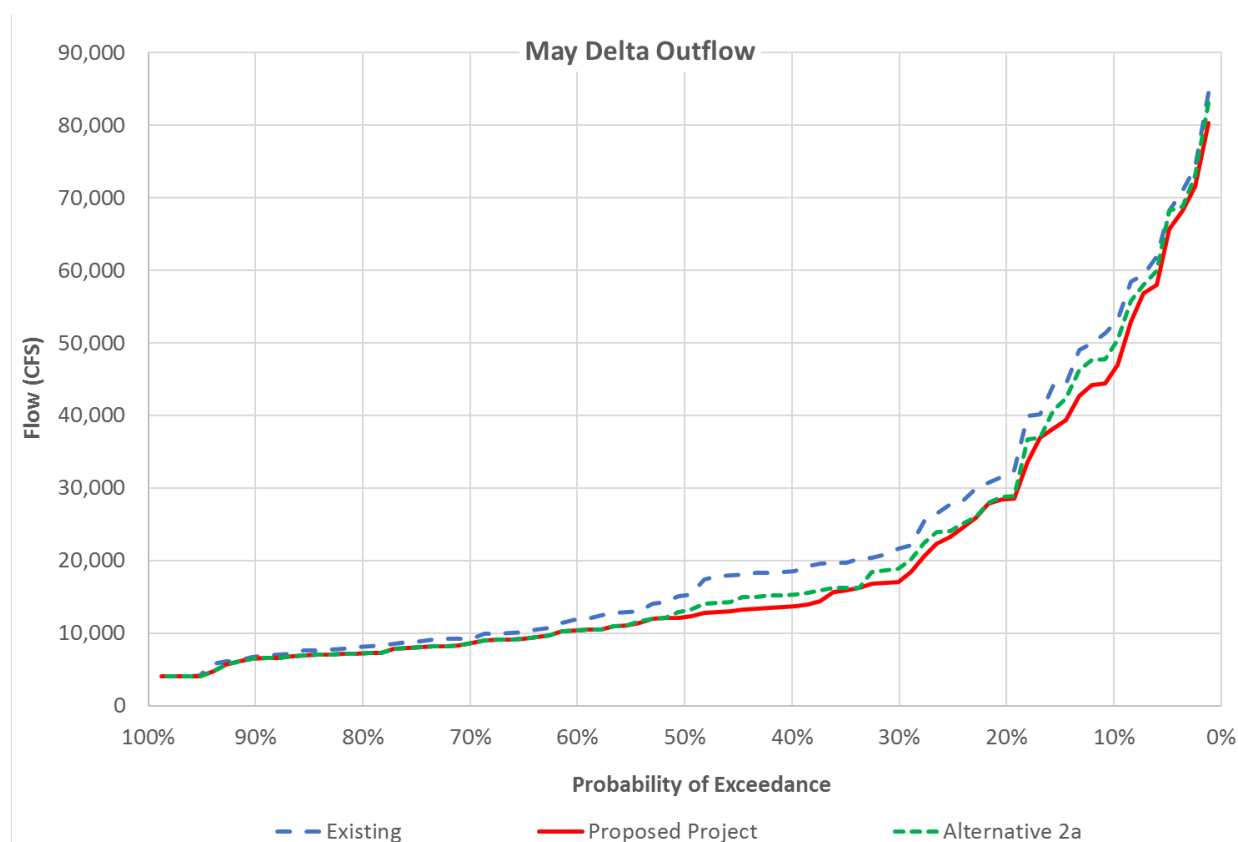
Figure 2: Probability of exceedance of Delta outflow in May
