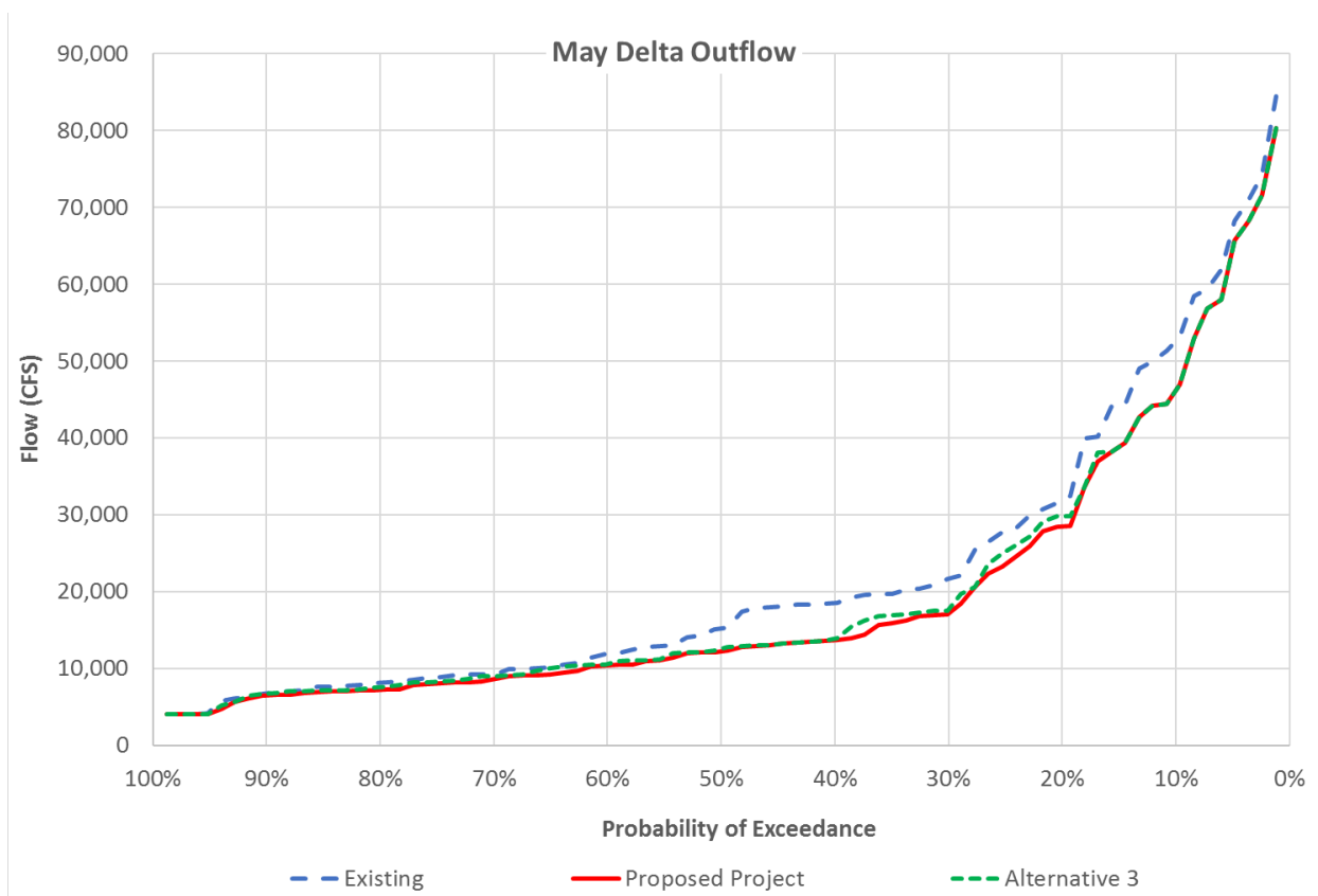
Figure 12: Probability of exceedance of Delta outflow in May
