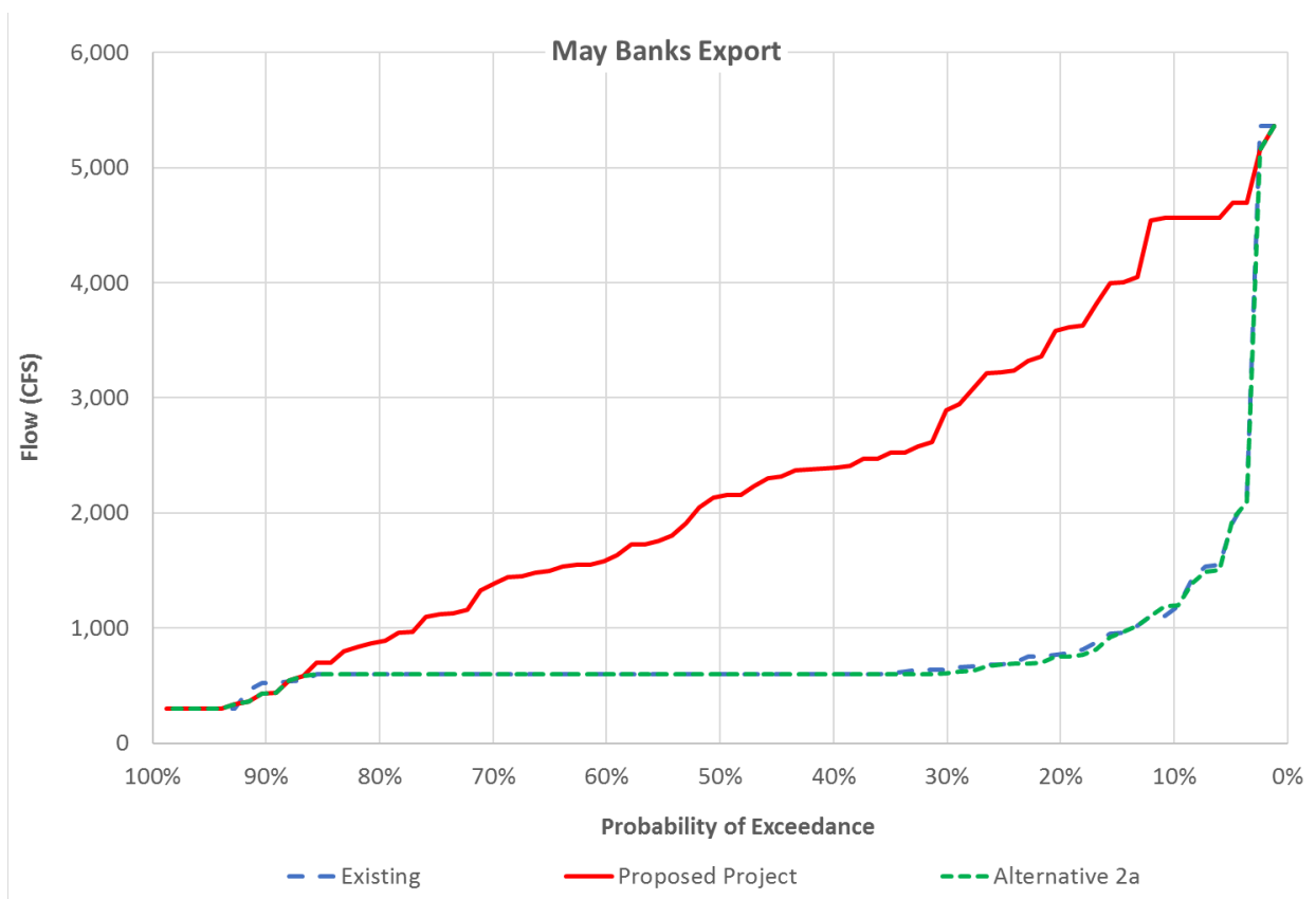
Figure 9: Probability of exceedance of Banks export in May
