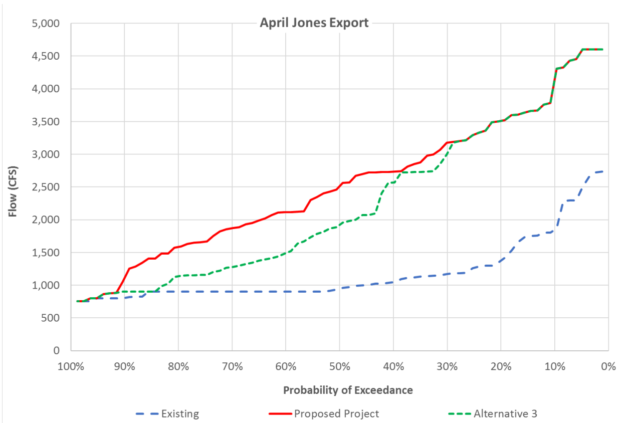
Figure 17: Probability of exceedance of Jones export in April
