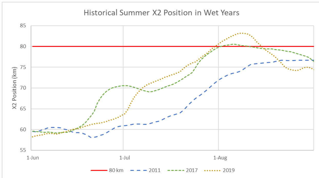
Figure 11. Historical summer 14-day running average X2 position in wet years
