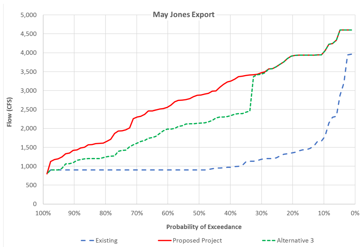
Figure 18: Probability of exceedance of Jones export in May
