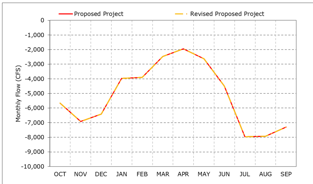
Figure 1 Combined Old and Middle River Monthly Flow for the Proposed Project and Revised Proposed Project
