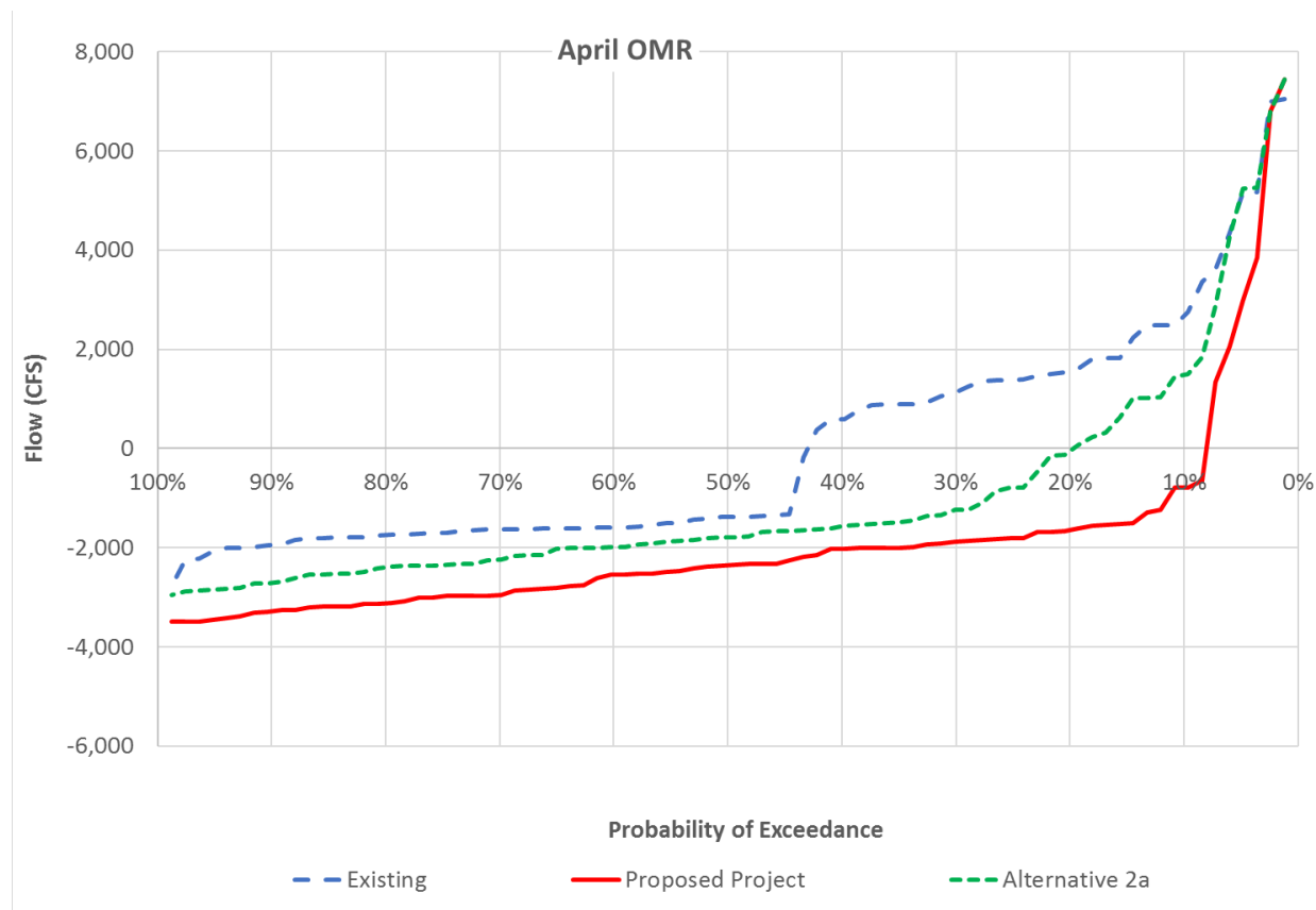
Figure 3: Probability of exceedance of OMR flow in April
