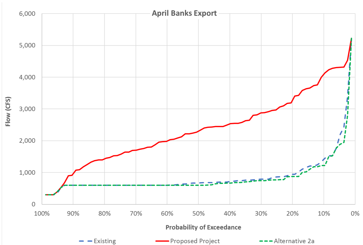
Figure 8: Probability of exceedance of Banks export in April
