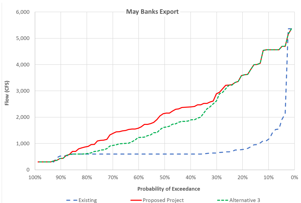
Figure 2010: Probability of exceedance of Banks export in May
