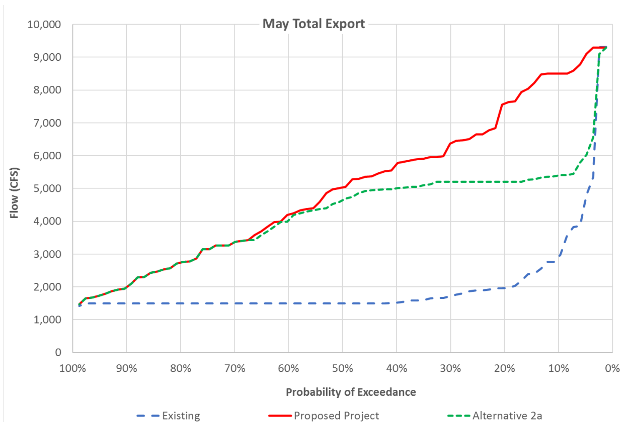
Figure 5: Probability of exceedance of total exports in May
