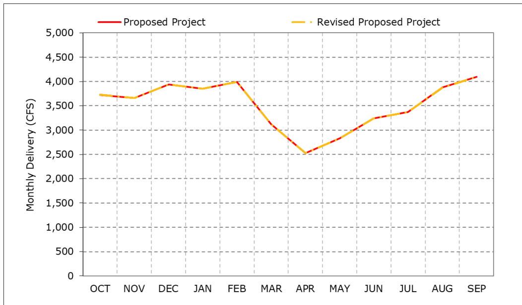
Figure 3 Jones Pumping Plant Monthly Exports for the Proposed Project and Revised Proposed Project
