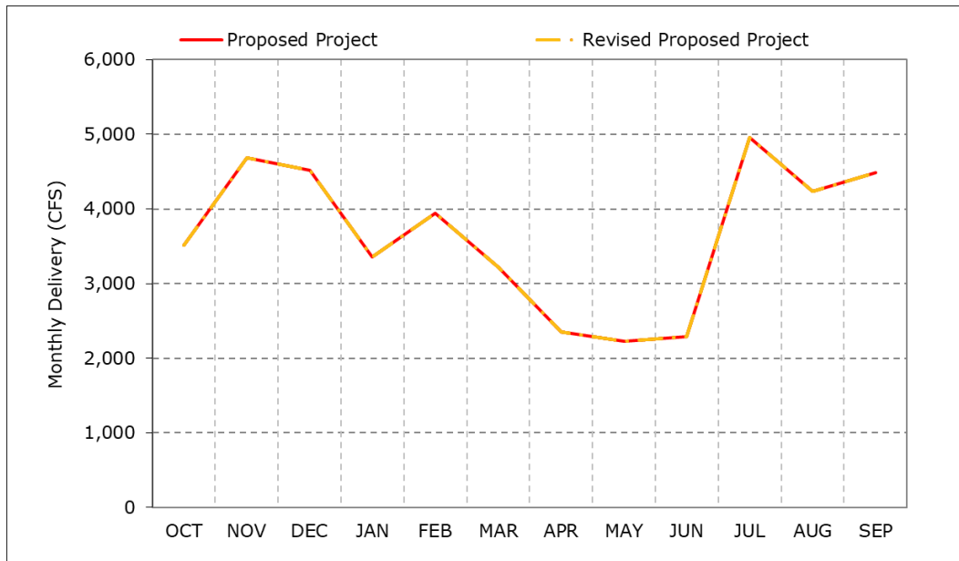
Figure 2 SWP Banks Pumping Plant Monthly Exports for the Proposed Project and Revised Proposed Project
