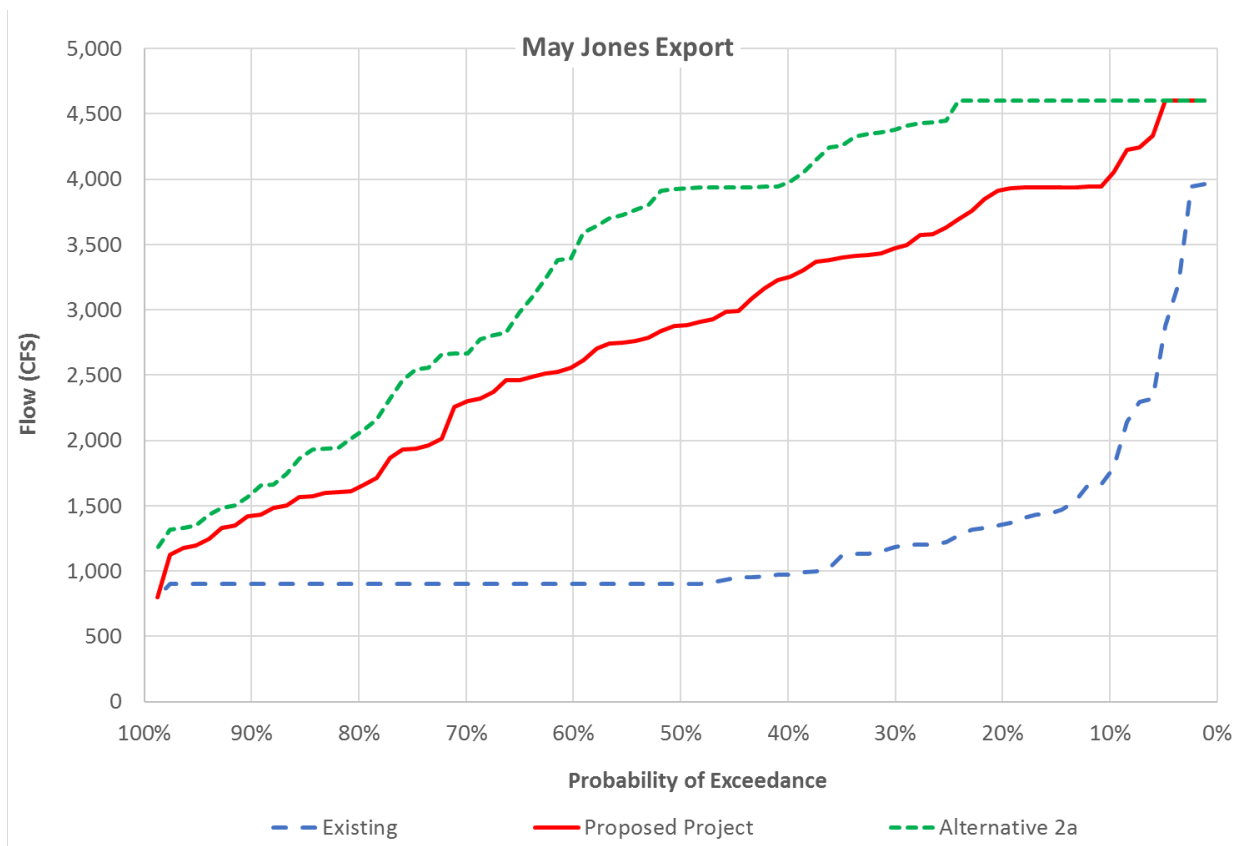
Figure 7: Probability of exceedance of Jones export in May
