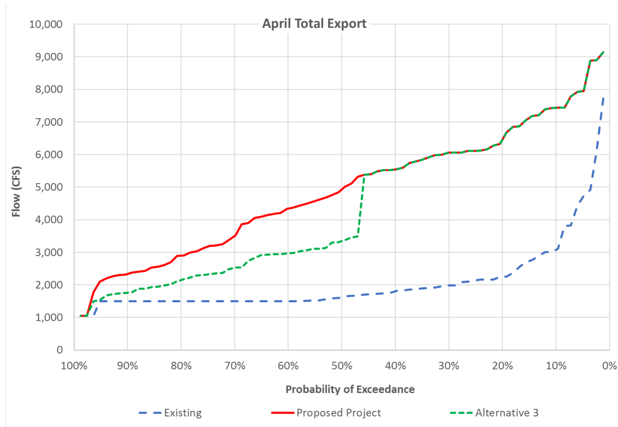
Figure 15: Probability of exceedance of total exports in April
