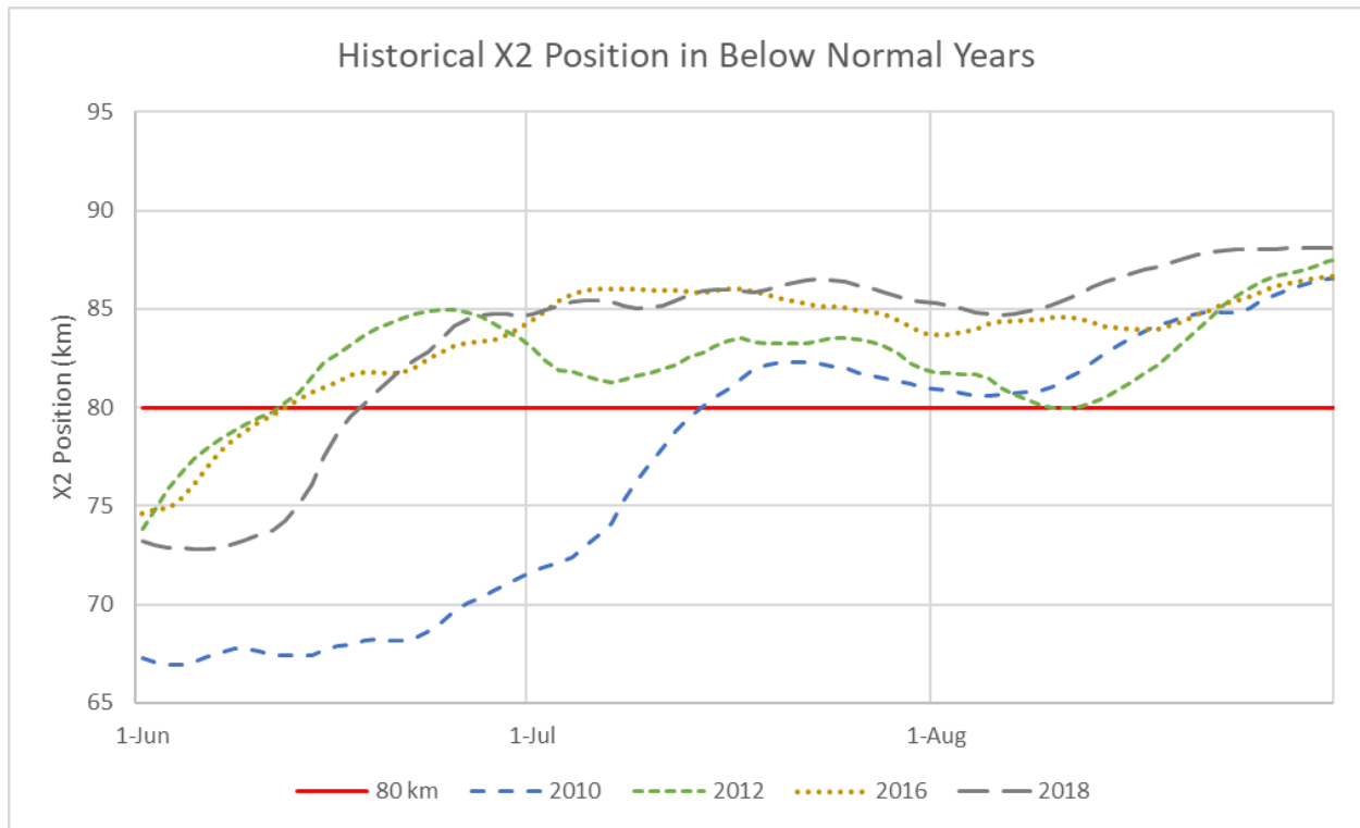
Figure 12. Historical summer 14-day running average X2 position in below normal years
