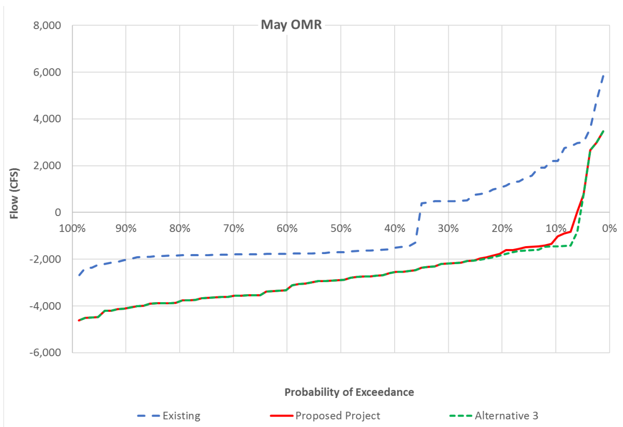
Figure 14: Probability of exceedance of OMR flow in May
