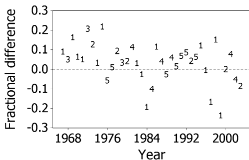
Fig. 4 Time series for the fractional difference of scenario A from empirical \chi^2 . Numbers represent water year types; 1 wet, 2 above normal, 3 below normal, 4 dry, 5 critical
