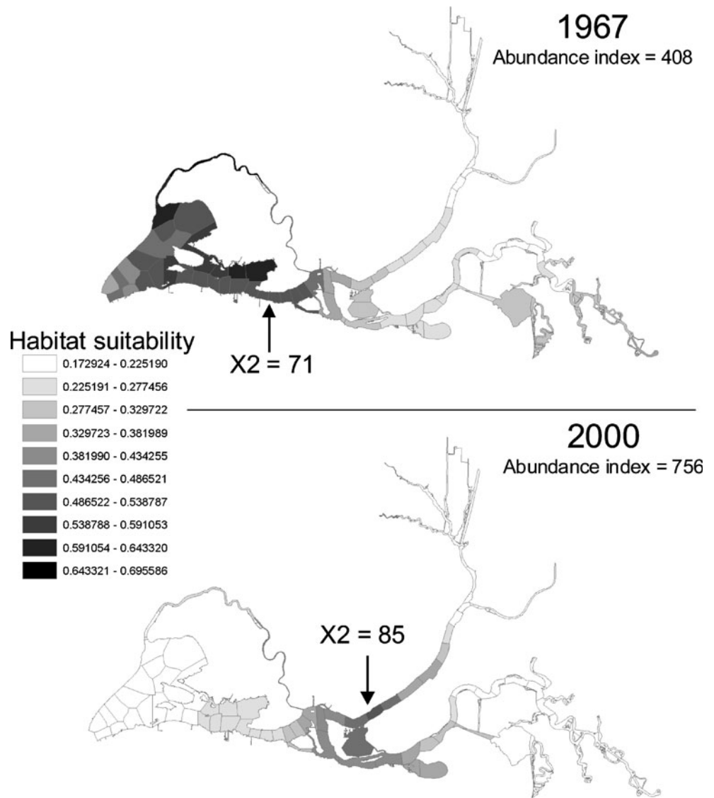
Fig. 3 Spatial distribution of habitat suitability, defined as the GAM probability of occurrence, for years in which \chi^2 was either below (1967) or above (2000) the confluence of the Sacramento and San Joaquin Rivers. Abundance index is from the fall midwater trawl survey
