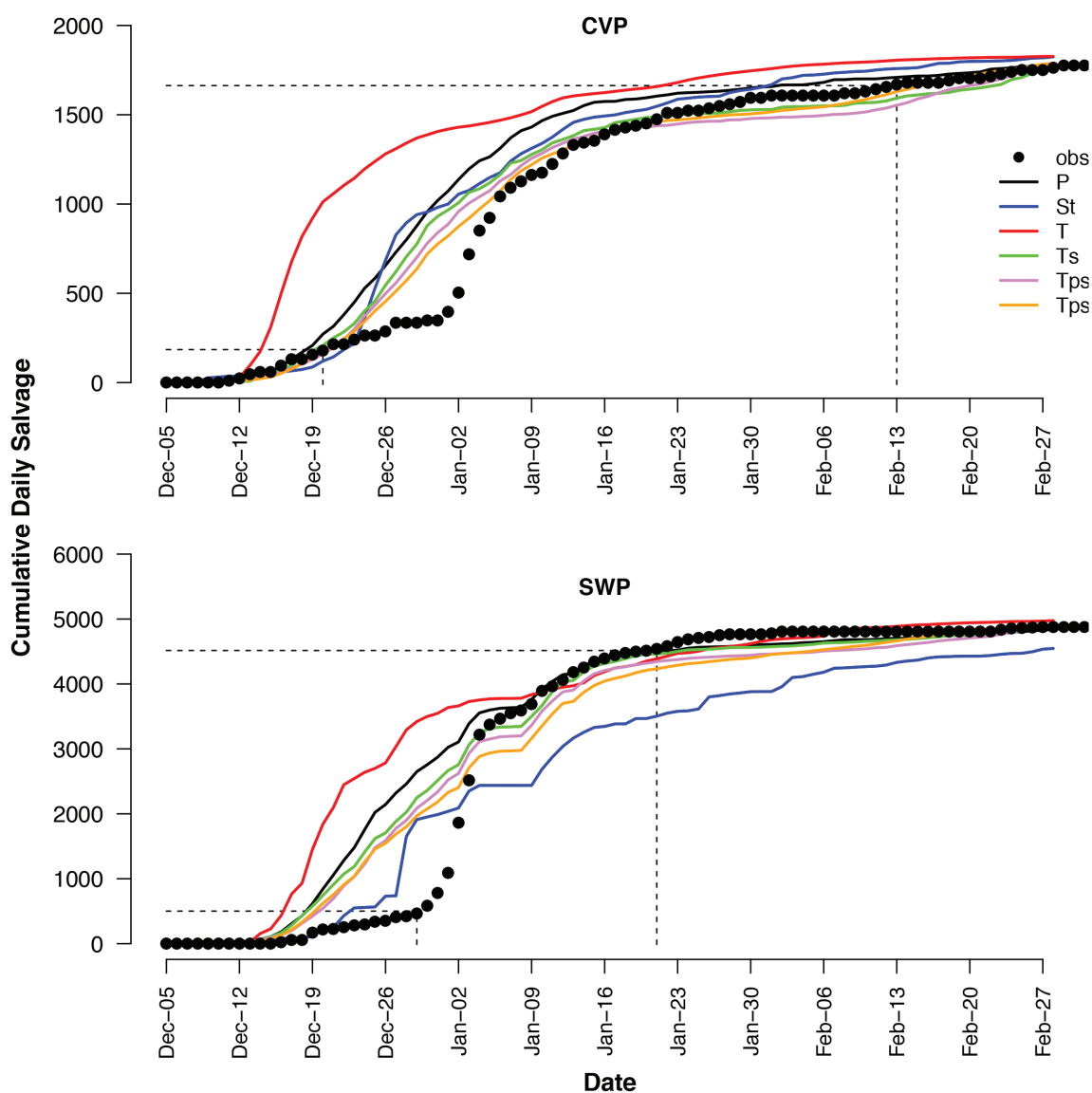
Figure A2 Comparisons of the fit of all behavior models to the observed cumulative daily salvage data at federal (CVP) and state (SWP) facilities. All models were fit using population model 2 (constant salvage expansion factors, and logistic daily variation in natural survival rate; see Table 2 in paper). The x-axis values at the intersection of the dashed horizontal lines and the salvage curves identify the date ranges when 80% of the salvage of adult Delta Smelt is collected. The plotted data range ends on February 28 to make it easier to see differences in timing of predicted salvage among models.
