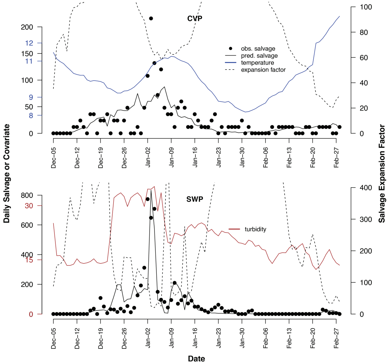
Figure A1 Fit of models that predict pre-screen loss as a function of both water temperature (Mallard) and turbidity (CCF). For clarity, these covariates are plotted on separate panels even though the same values apply to predictions at both the CVP and SWP. Also shown are salvage expansion factors, which are the inverse of salvage efficiencies. Results are based on the TpsHt behavior model and population model 5 (see Table 2 in paper). The plotted data range ends on February 28 to make it easier to compare observations and predictions and the relationship with covariates.
