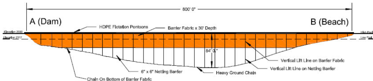
Figure 4. Cross-section View of the Intake Barrier Curtain Upstream of the Iron Gate Powerhouse Conduit Intake Near the Southeast Abutment of Iron Gate Dam.
