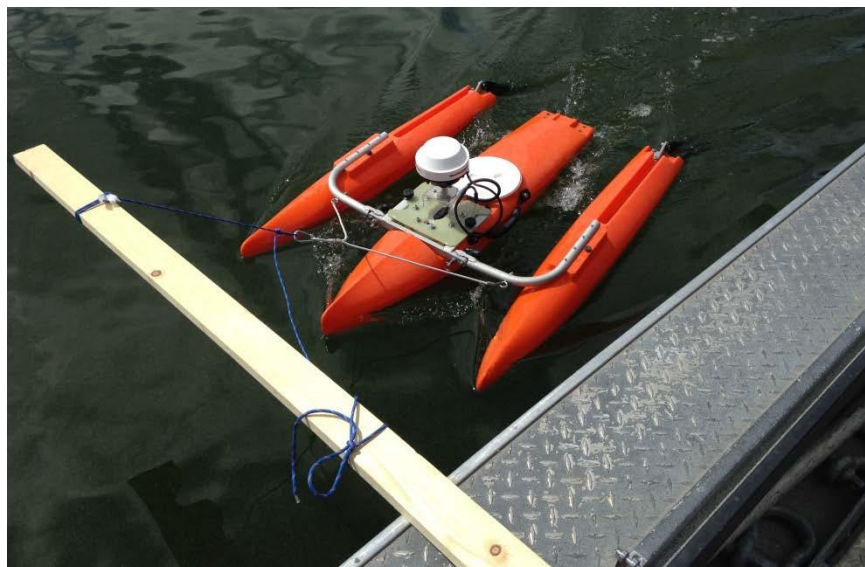
Figure 46. Acoustic Doppler Current Profiler Field Deployment.
