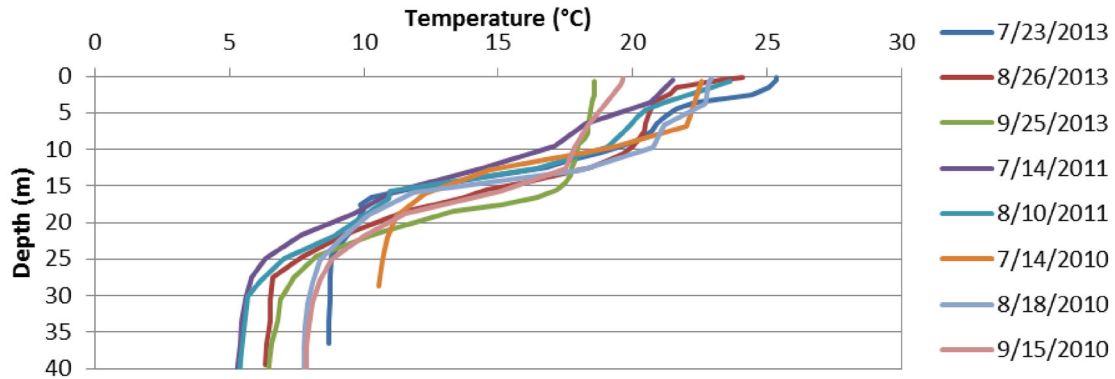
Figure 58. Vertical Temperature Profile Data at Iron Gate Reservoir Log Boom in 2010, 2011, and 2013.
