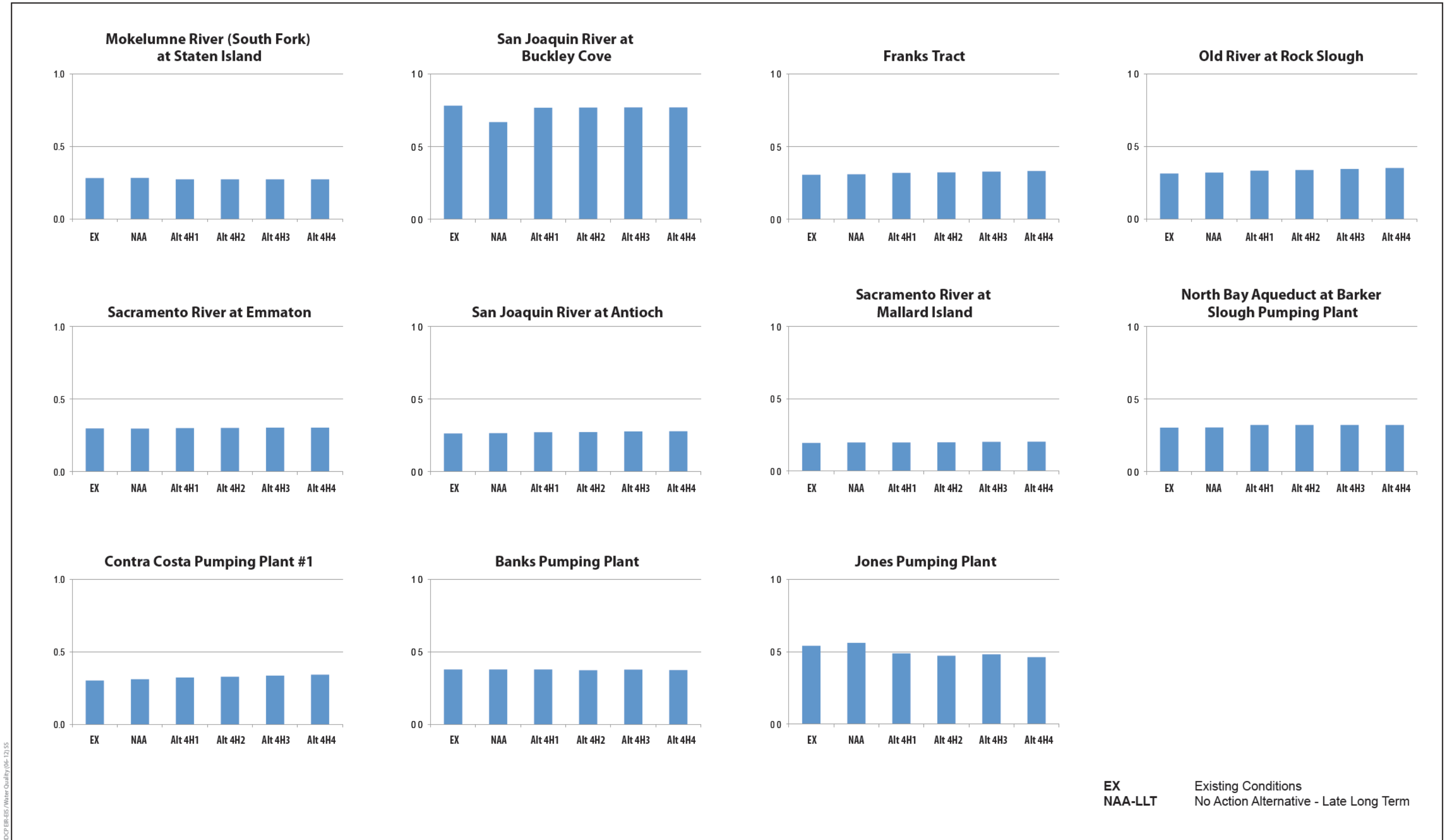
Figure 8-64a Tissue Advisory Level Exceedance Quotients for Selenium Concentrations in Fish Fillets for Drought Years
