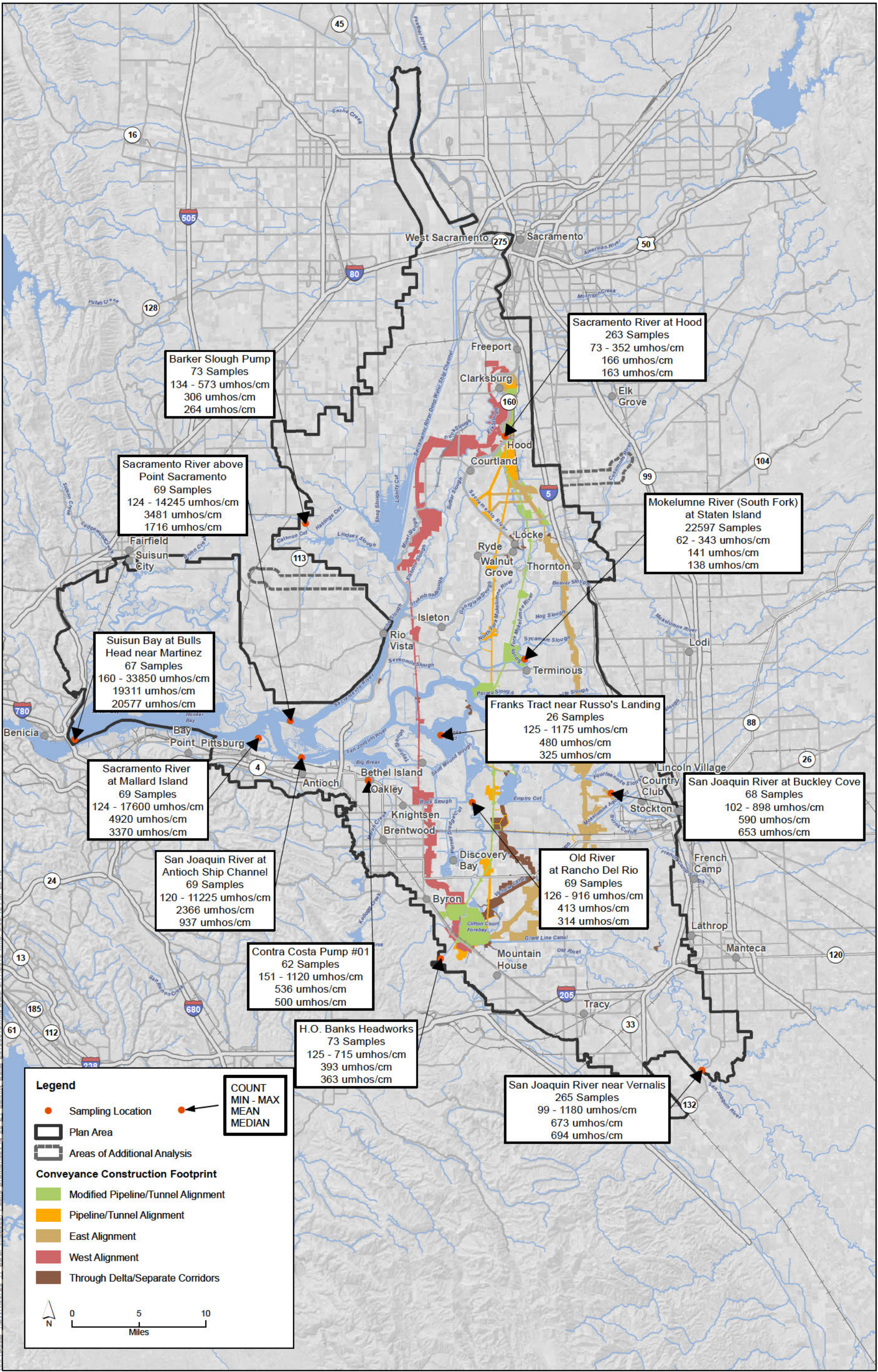
Figure 8-24 Spatial Summary of Salinity Data at Delta Stations (2001 - 2006)
