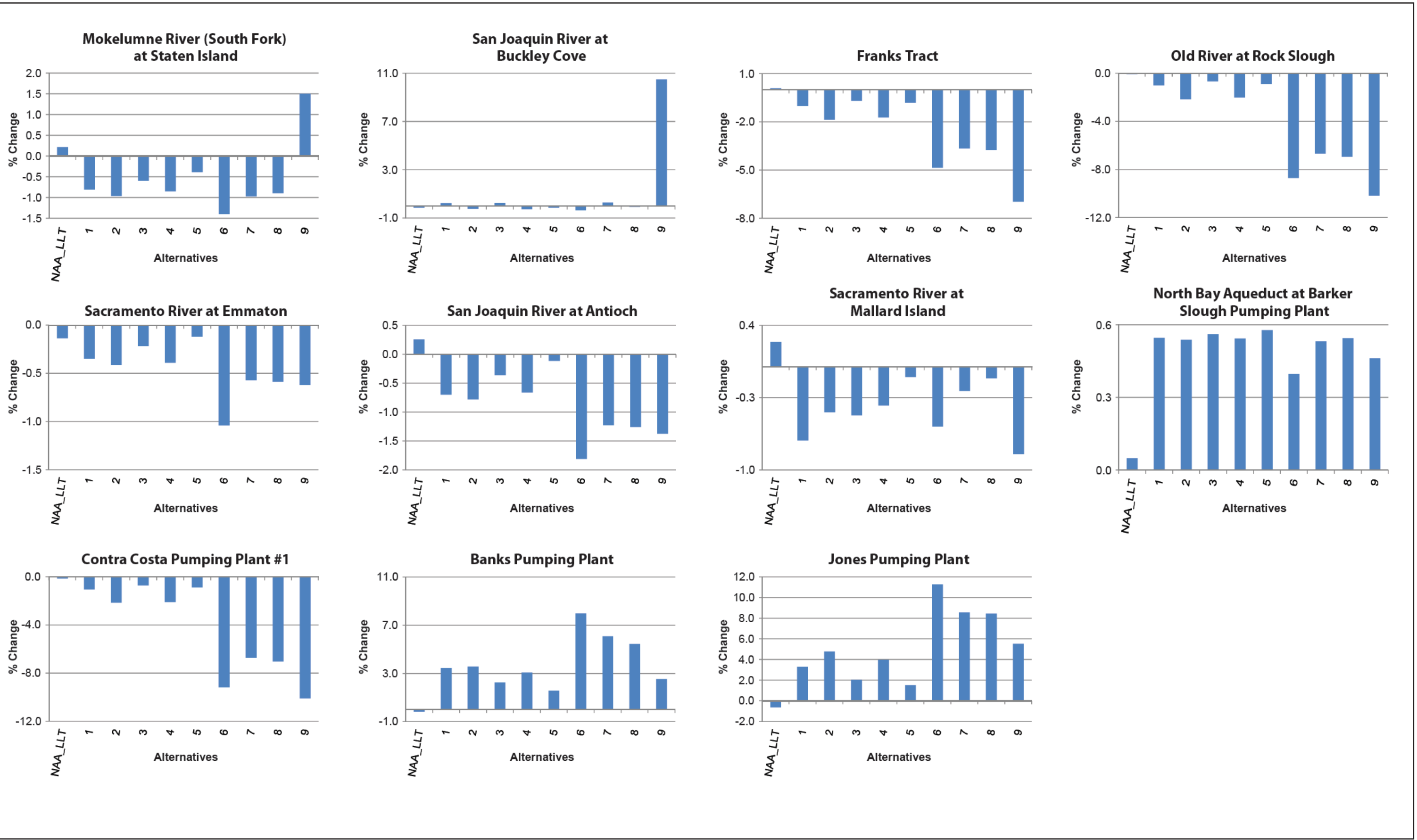
Figure 8-53a Percent Change in Available Assimilative Capacity for Mercury (Based on 25 ng/L Ecological Risk Benchmark) with Respect to Existing Conditions for All Years
