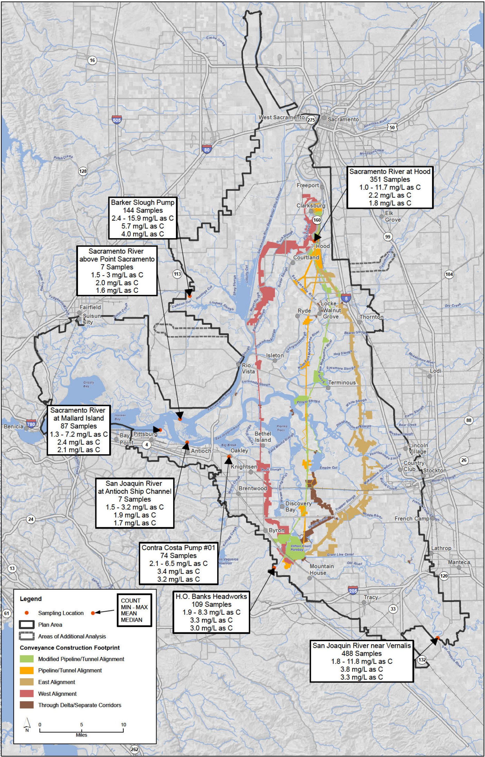
Figure 8-38 Spatial Summary of Dissolved Organic Carbon Data at Delta Stations (2001 - 2006)
