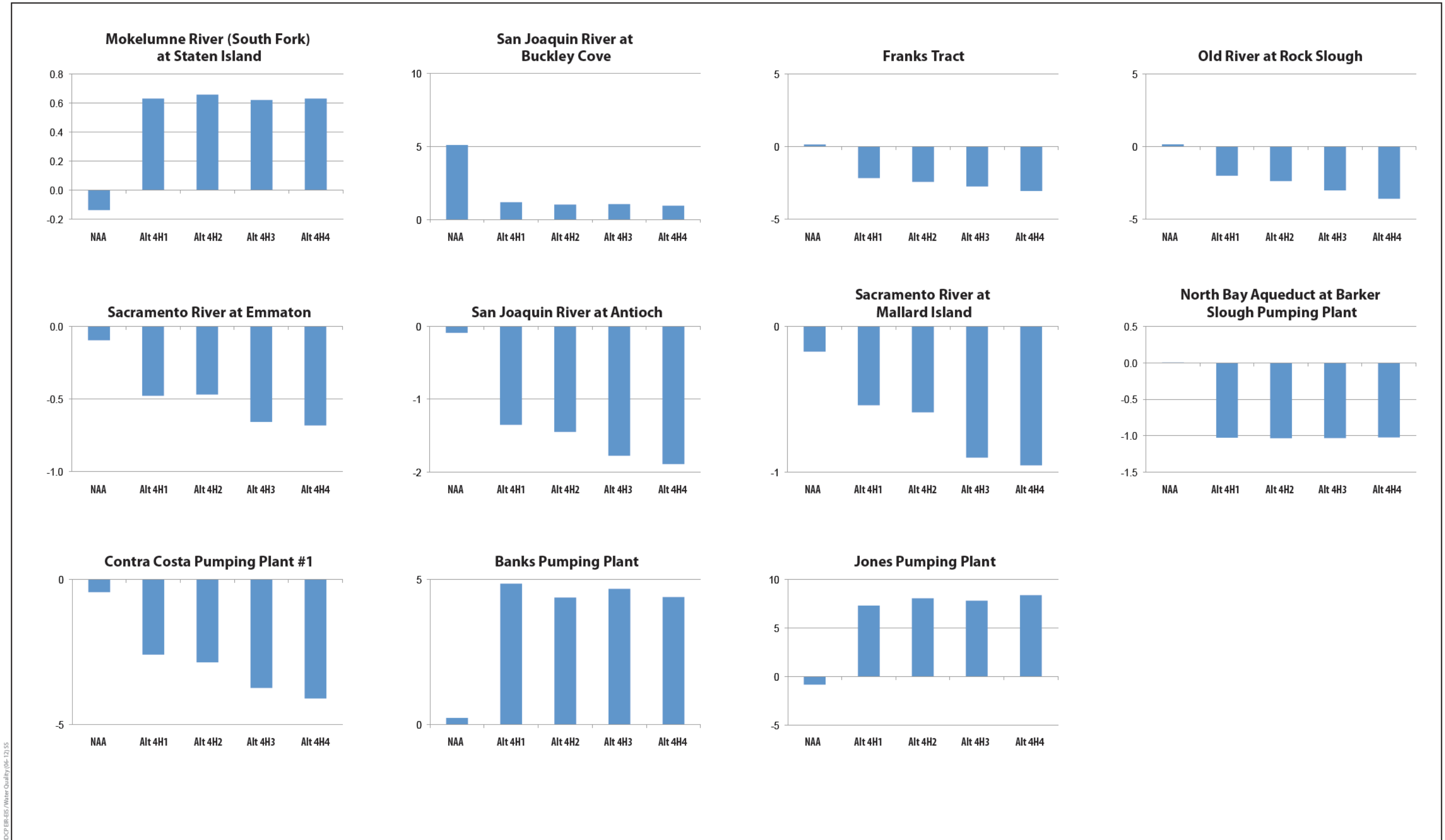
Figure 8-59b Percent Change in Available Assimilative Capacity for Selenium (Based on 2 µg/L Ecological Risk Benchmark) with Respect to Existing Conditions for All Years
