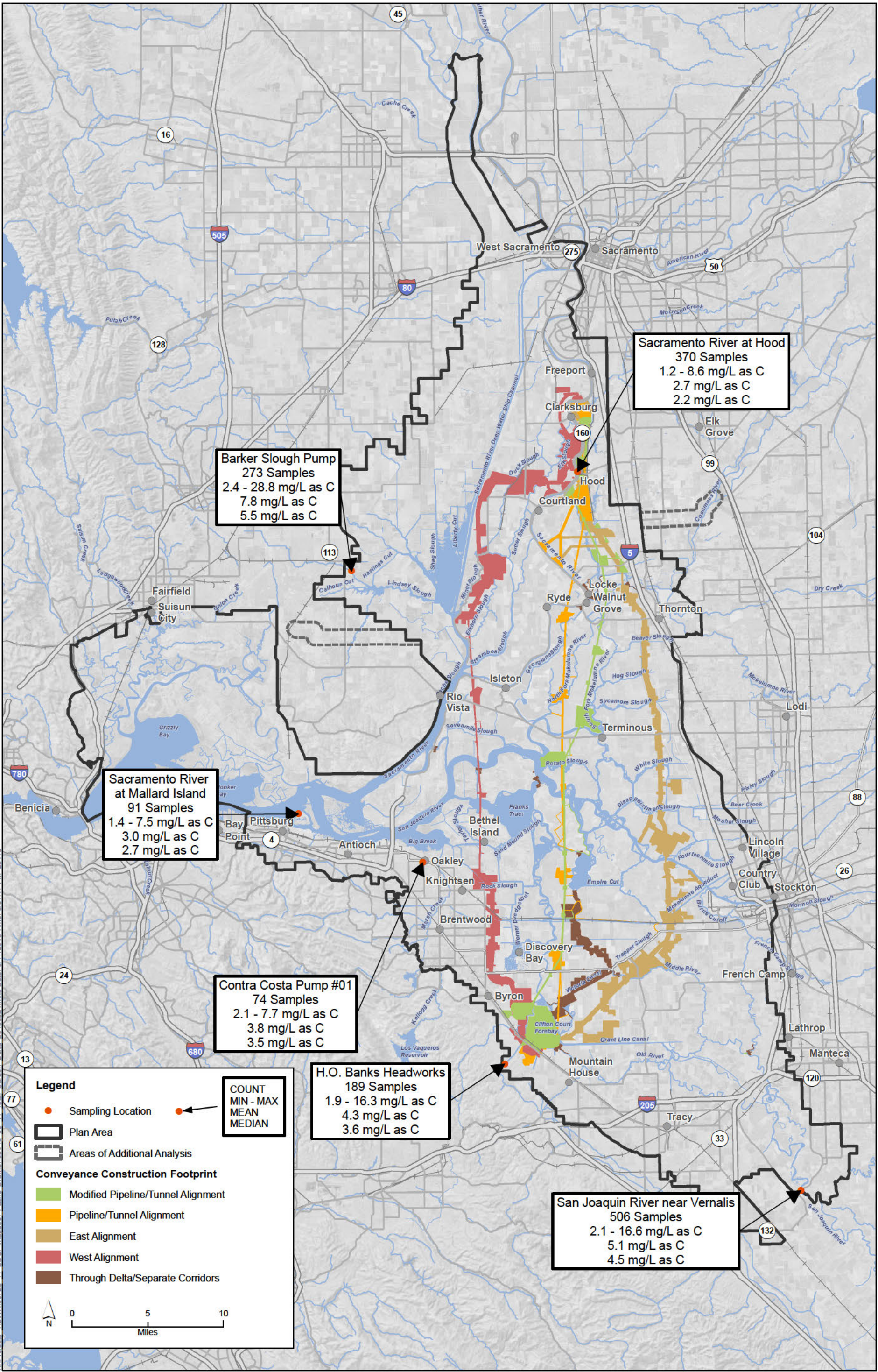
Figure 8-41 Spatial Summary of Total Organic Carbon Data at Delta Stations (2001 - 2006)
