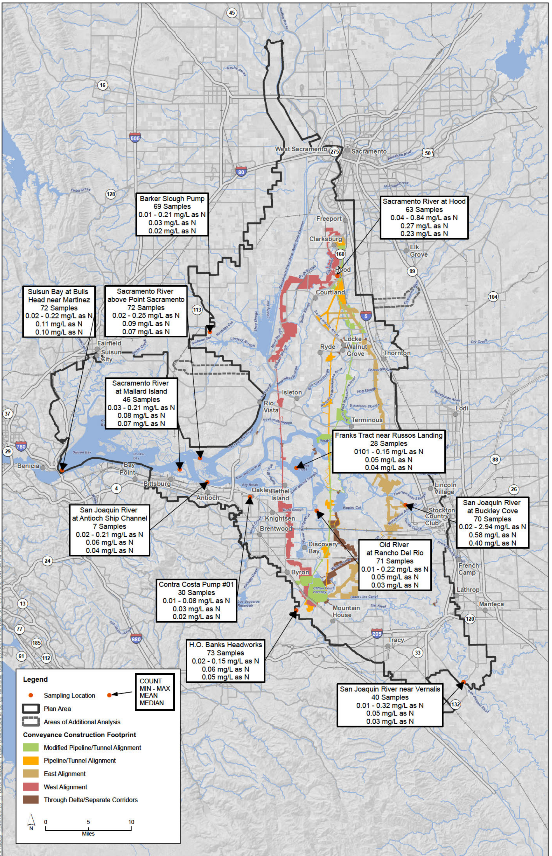
Figure 8-8 Spatial Summary of Ammonia Data at Delta Stations (2001 - 2006)
