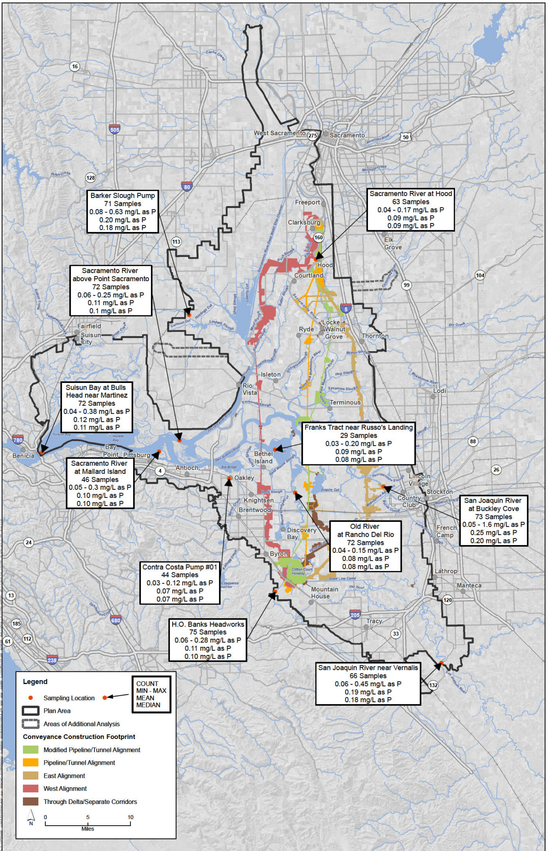
Figure 8-35 Spatial Summary of Total Phosphorus Data at Delta Stations (2001 - 2006)
