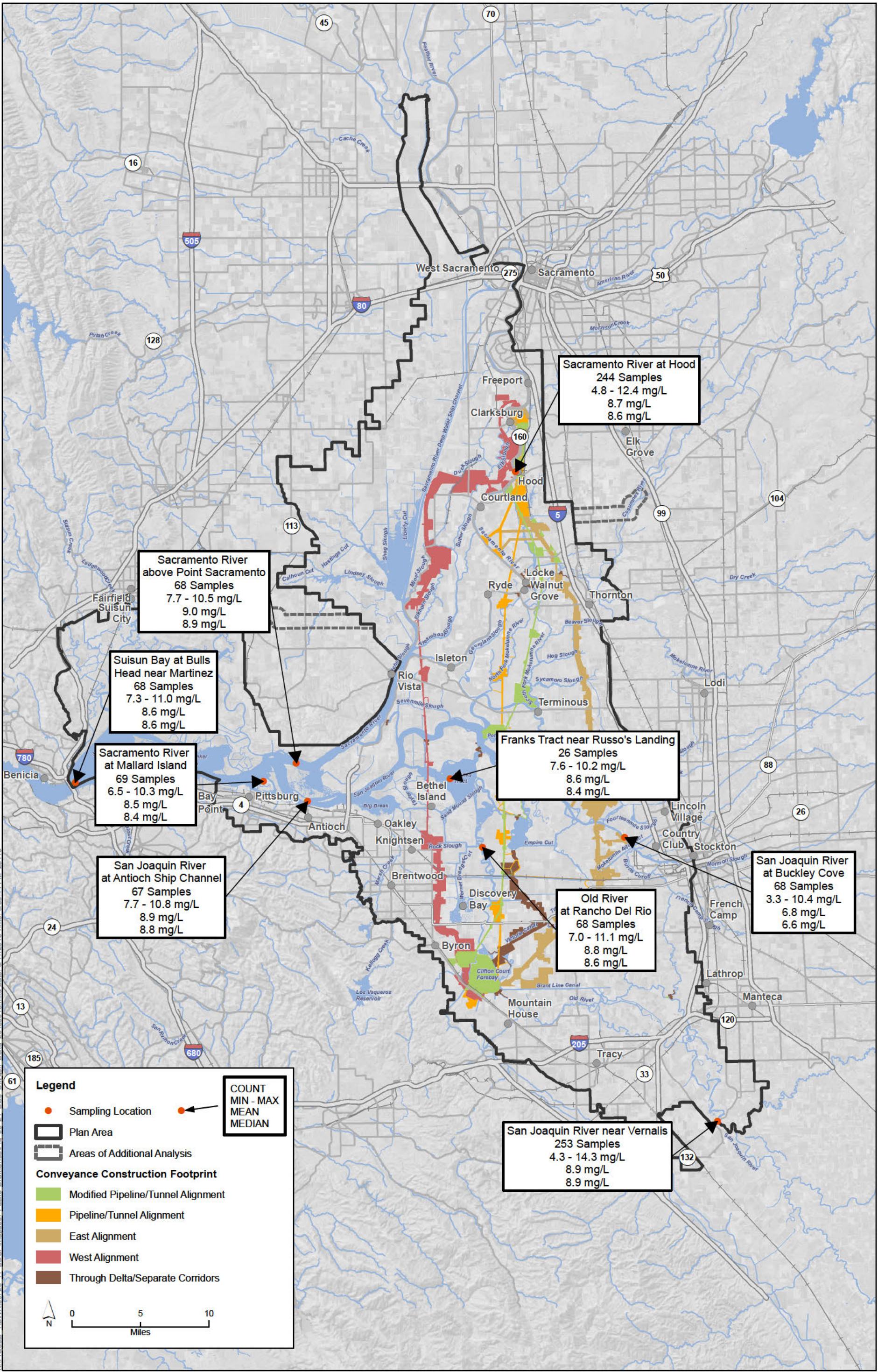
Figure 8-21 Spatial Summary of Dissolved Oxygen Data at Delta Stations (2001 - 2006)
