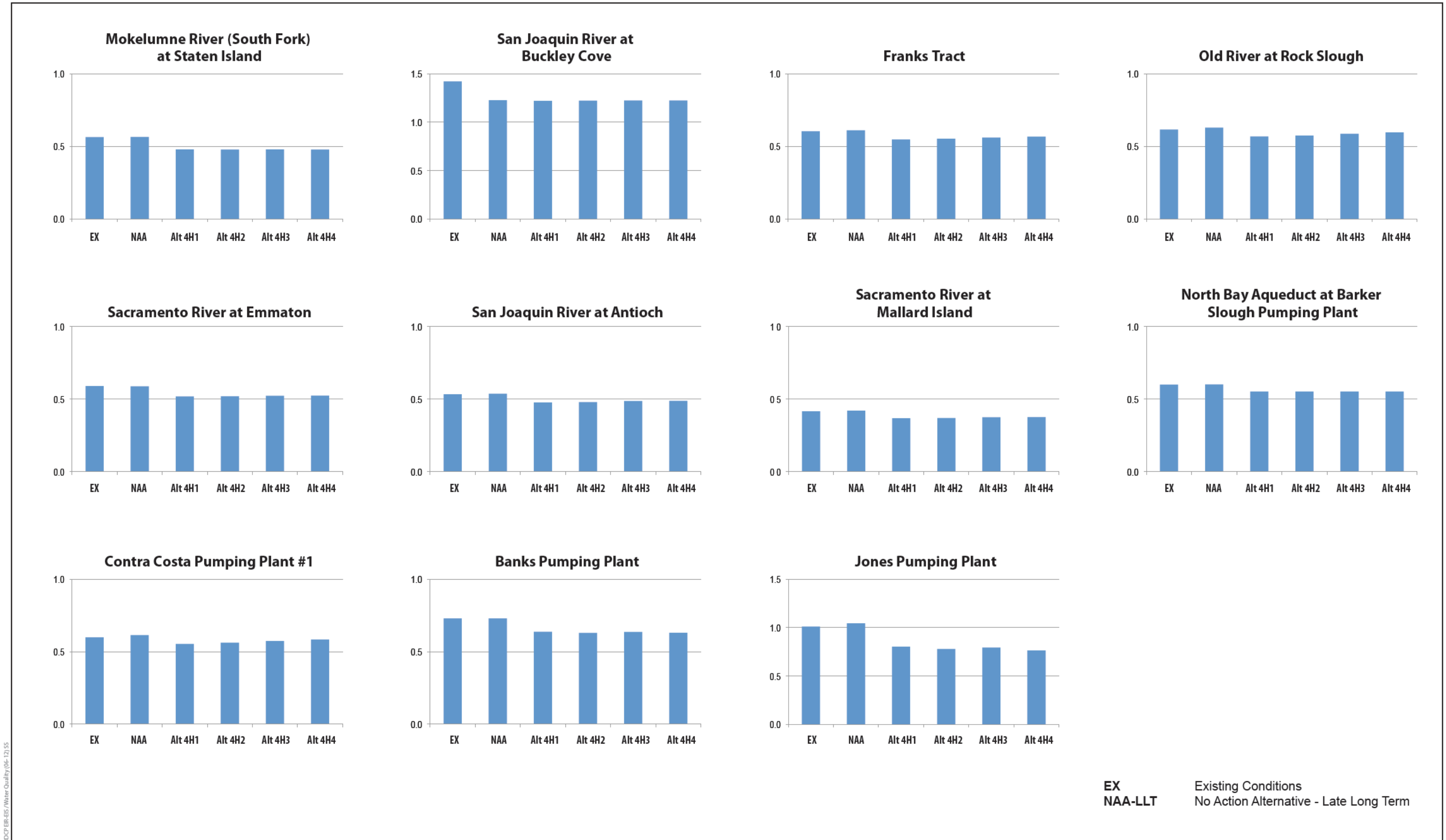
Figure 8-63b Level of Concern Exceedance Quotients for Selenium Concentrations in Bird Eggs (Fish Diet) for Drought Years
