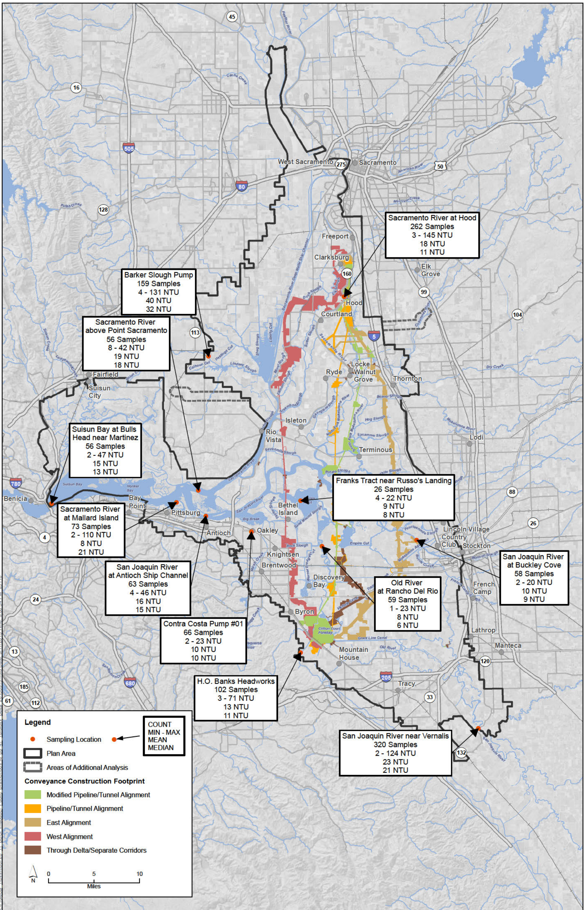
Figure 8-47 Spatial Summary of Turbidity Data at Delta Stations (2001 - 2006)
