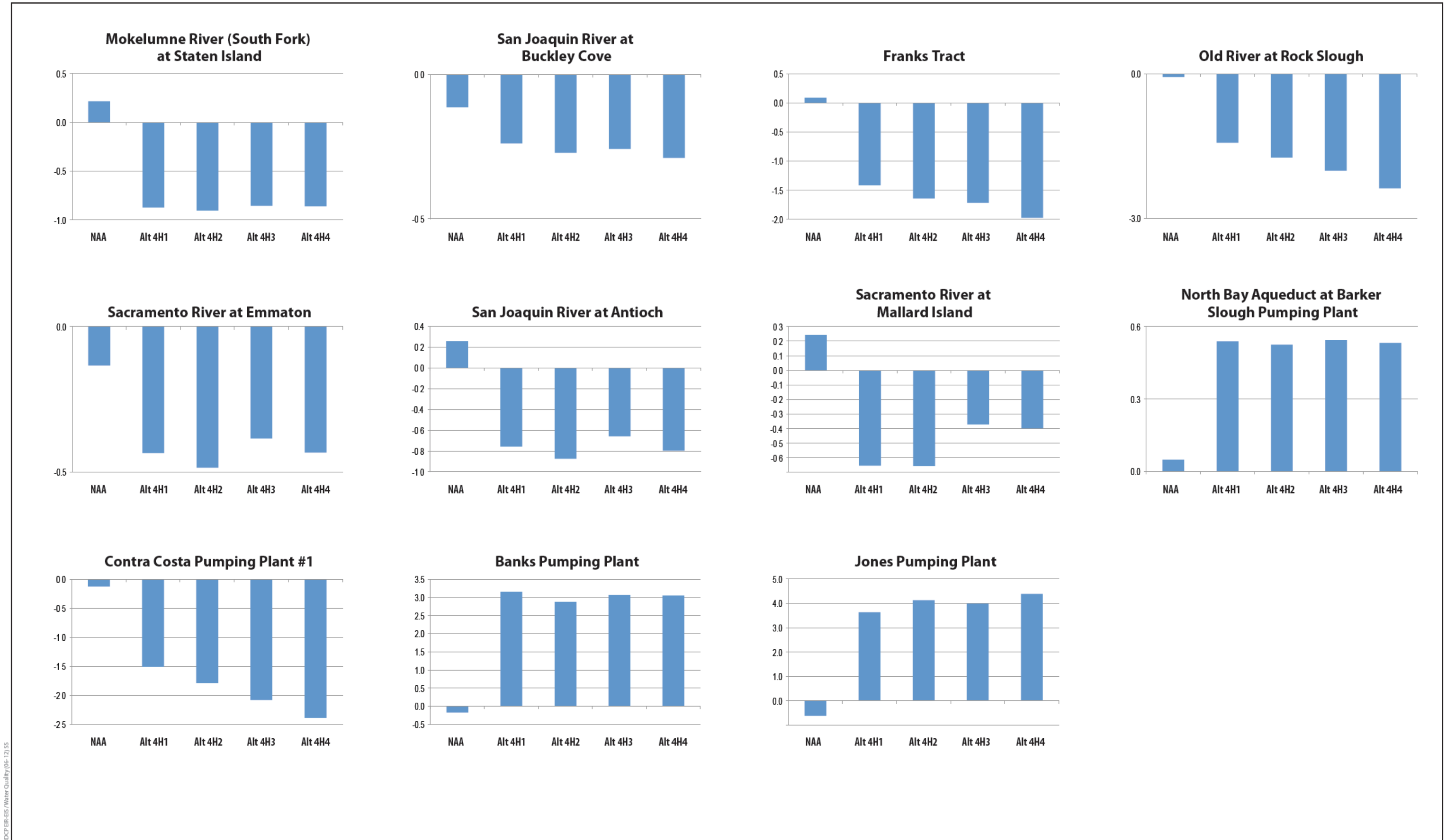
Figure 8-60b Percent Change in Available Assimilative Capacity for Selenium (Based on 2 µg/L Ecological Risk Benchmark) with Respect to No Action Alternative for All Years
