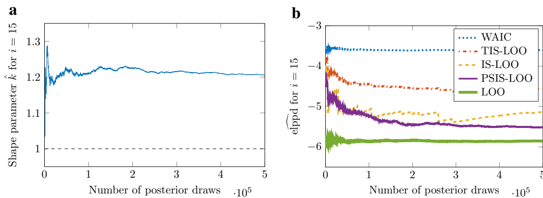
Fig. 9 Leukemia example: Distributions of a tail shape estimate and b LOO approximations for i = 15 . If we continue sampling, the tail shape estimate stays above 1 and \widehat{\text{elppd}}_i will not converge
