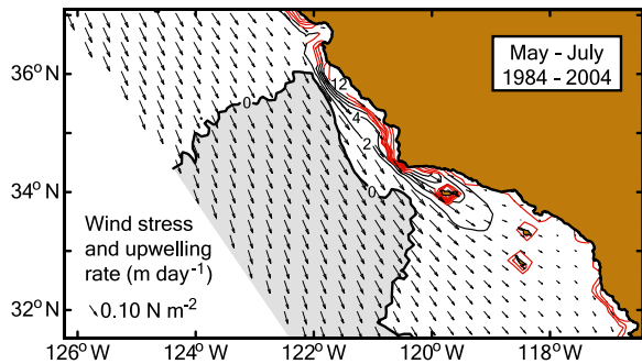
Fig. 3. Mean summertime (May–July) wind stress and upwelling rate from 1984 to 2004. Arrows indicate wind stress. Upwelling rates are denoted by contours at an interval of 2 m day -1 . Black contours indicate the region of curl-driven upwelling. Red contours denote coastal upwelling. Areas of anti-cyclonic curl (downwelling) are shaded. The years 1984–2004 correspond to the period during which nutrient, chlorophyll, and sardine production data were regularly collected.
