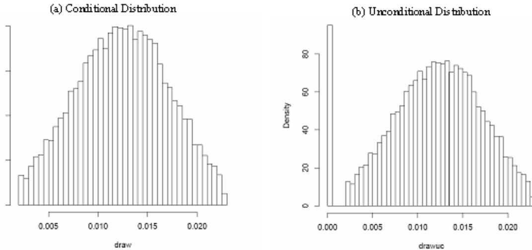
Figure G-9. Histogram of the Random Draw from the Distribution of the PM 2.5 Effect Specified by Expert I
