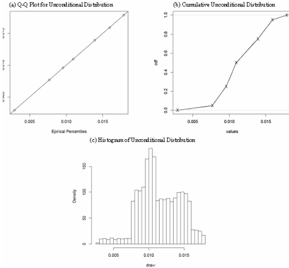
Figure G-6. Characteristics of the Random Draw from the Approximated Distribution of the PM 2.5 Effect Specified by Expert F (continued) (2) Results for the range >7-30 µg/m 3
