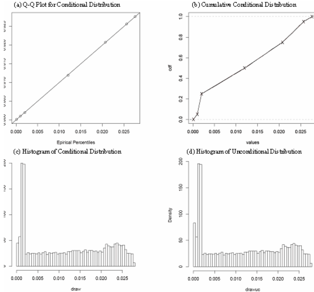
Figure G-2. Characteristics of the Random Draw from the Approximated Distribution of the PM_{2.5} Effect Specified by Expert B (1) Results for the range 4-10 \mu\text{g}/\text{m}^3
