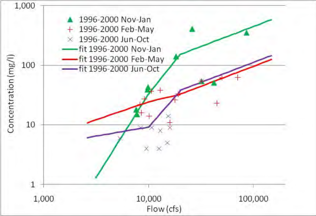
Figure 2-3. 1996 to 2000 suspended sediment data given by time of year collected. Regression fits are shown as solid lines and data is given as points.
