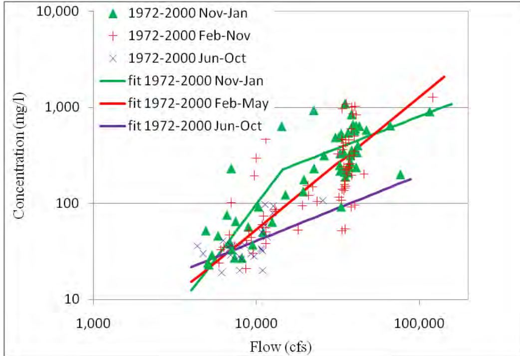
Figure 2-8. 1972 to 2000 suspended sediment data near the New Delevan Pipeline given by time of year collected. Fits are shown as solid lines and data is given as points.
