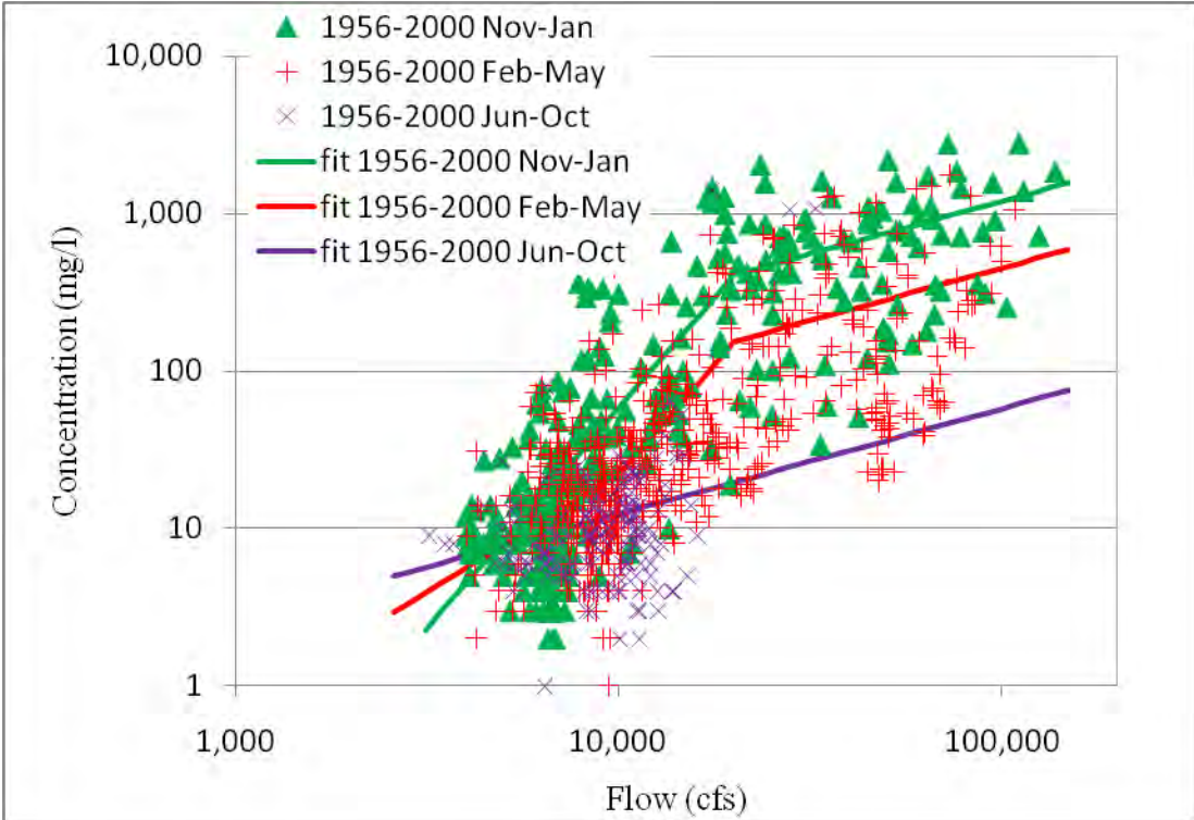
Figure 2-4. 1956 to 2000 suspended sediment data given by time of year collected. Regression fits are shown as solid lines and data is given as points.
