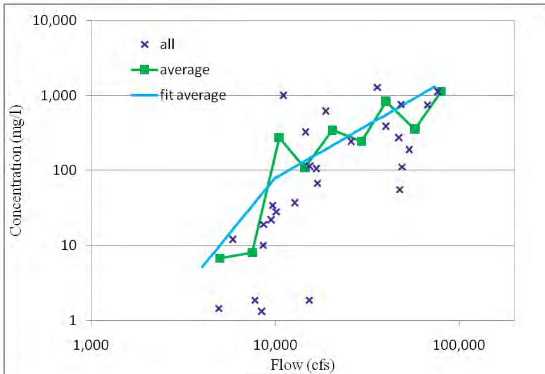
Figure 2-9. All suspended sediment data collected by USGS gages near the GC Canal. Fits are shown as solid lines and data is given as points.
