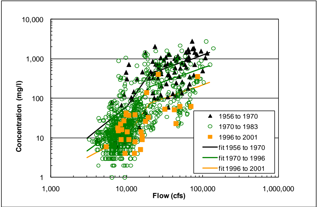
Figure 2-2. USGS suspended sediment data by various time periods. Regression fits are shown as solid lines and data is given as points.
