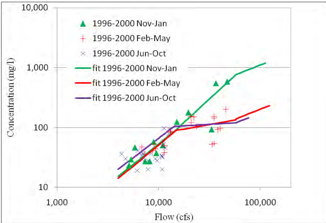
Figure 2-7. 1996 to 2000 suspended sediment data near the New Delevan Pipeline given by time of year collected. Fits are shown as solid lines and data is given as points.
