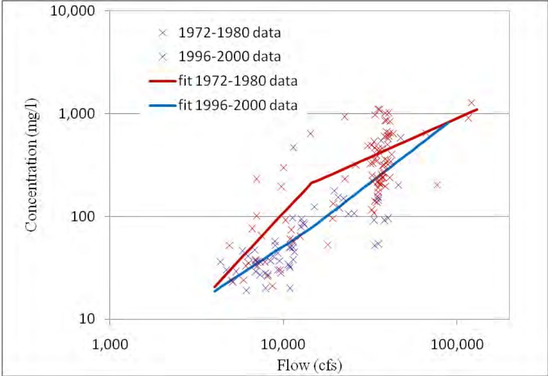
Figure 2-6. USGS suspended sediment data near the New Delevan Pipeline by various time periods. Fits are shown as solid lines and data is given as points.
